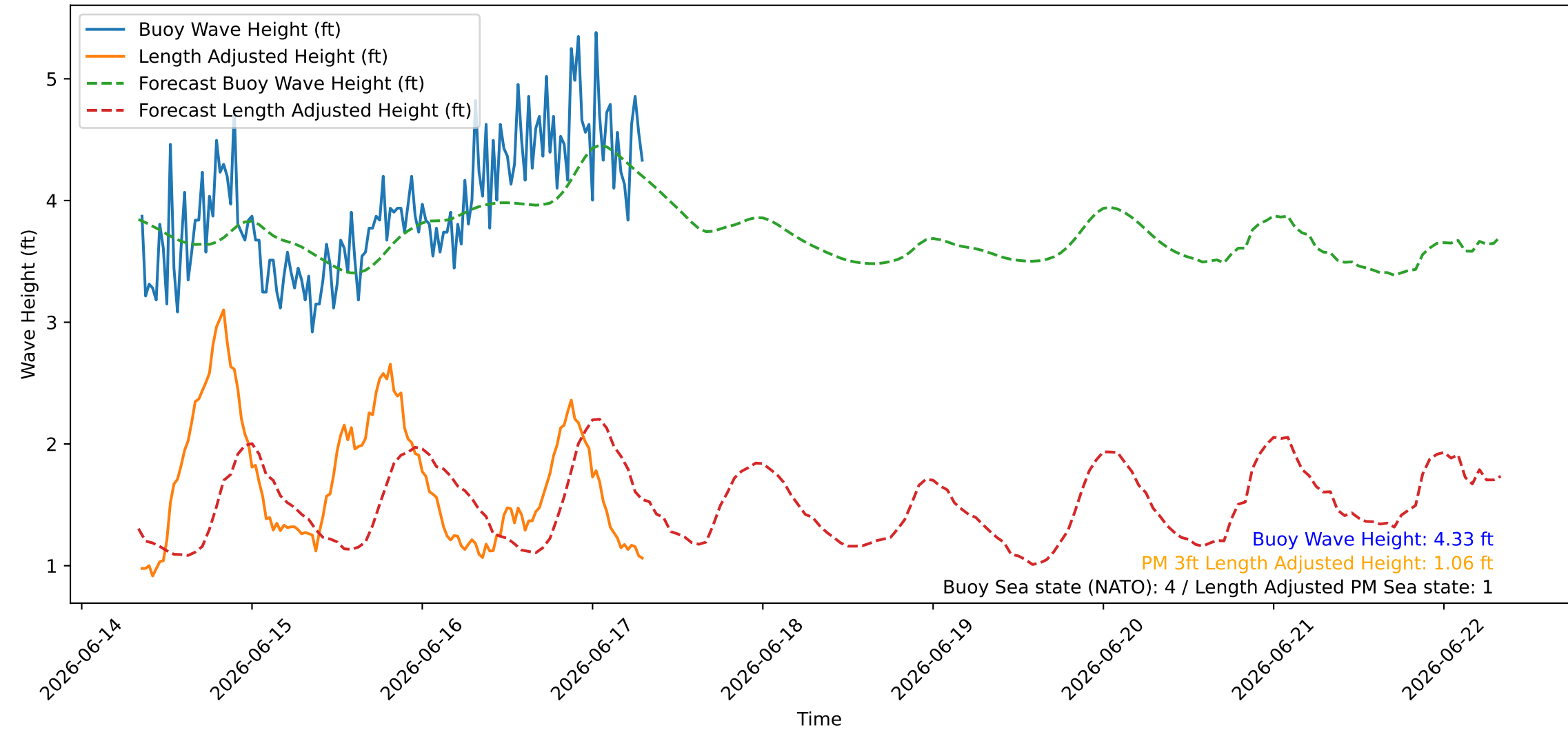
Wave Heights over Time for Red Beach at 2026-06-17 08:00:45
