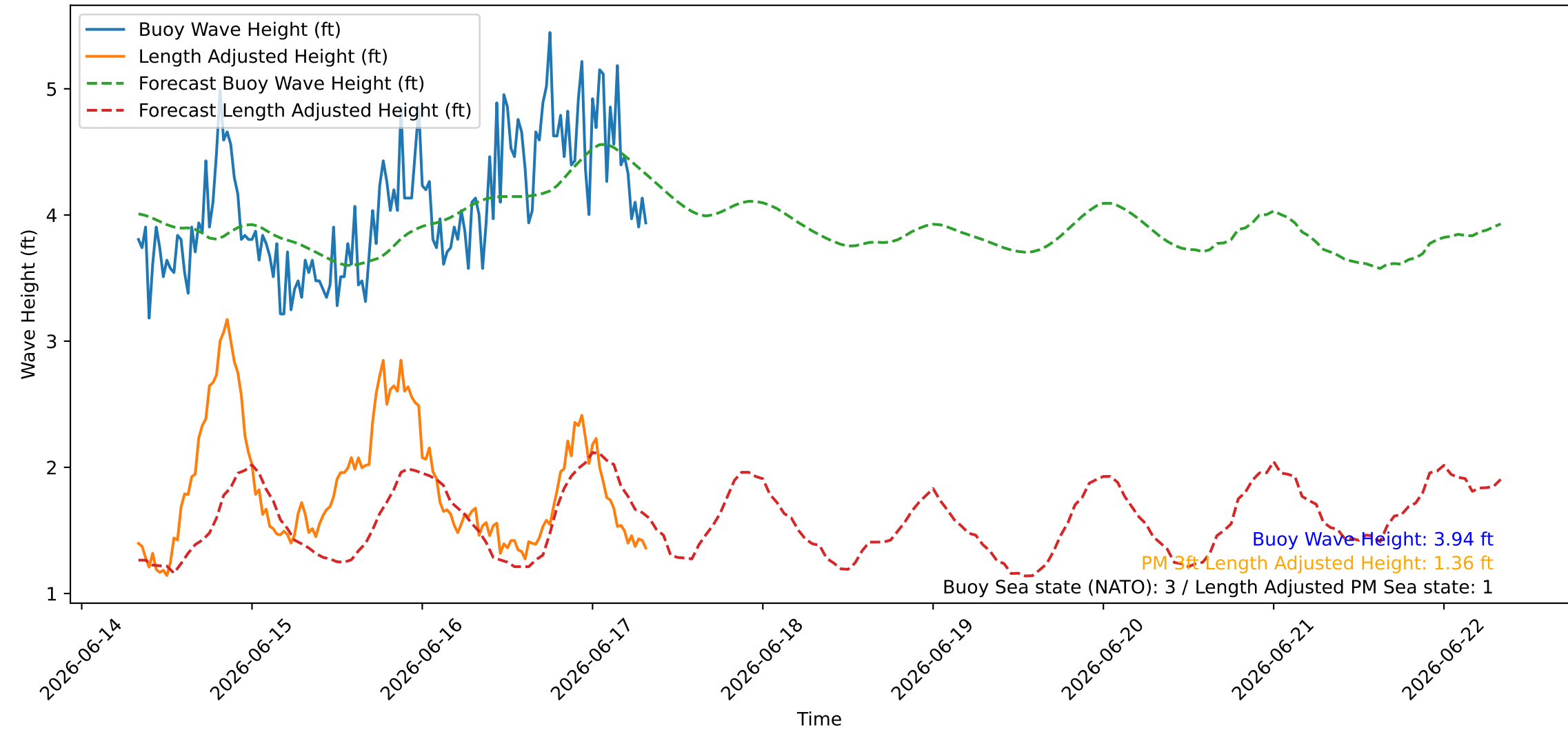
Wave Heights over Time for Oceanside Harbor at 2026-06-17 08:00:26
