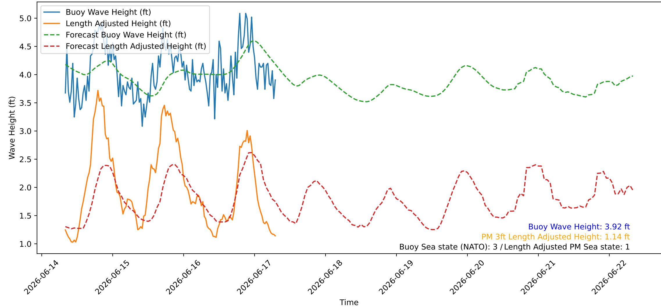
Wave Heights over Time for Green Beach at 2026-06-17 08:01:07
