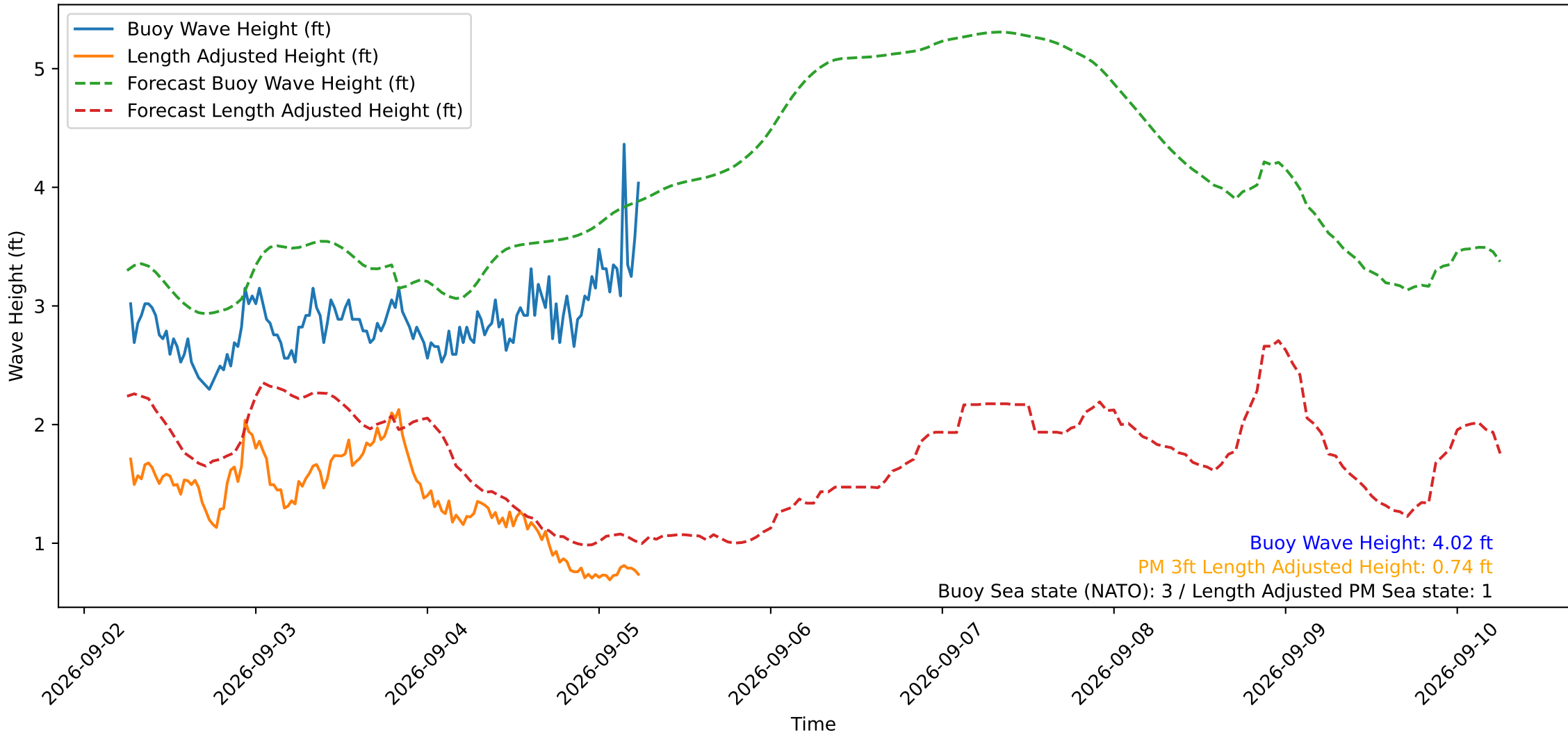
Wave Heights over Time for Red Beach at 2026-09-05 06:10:50
