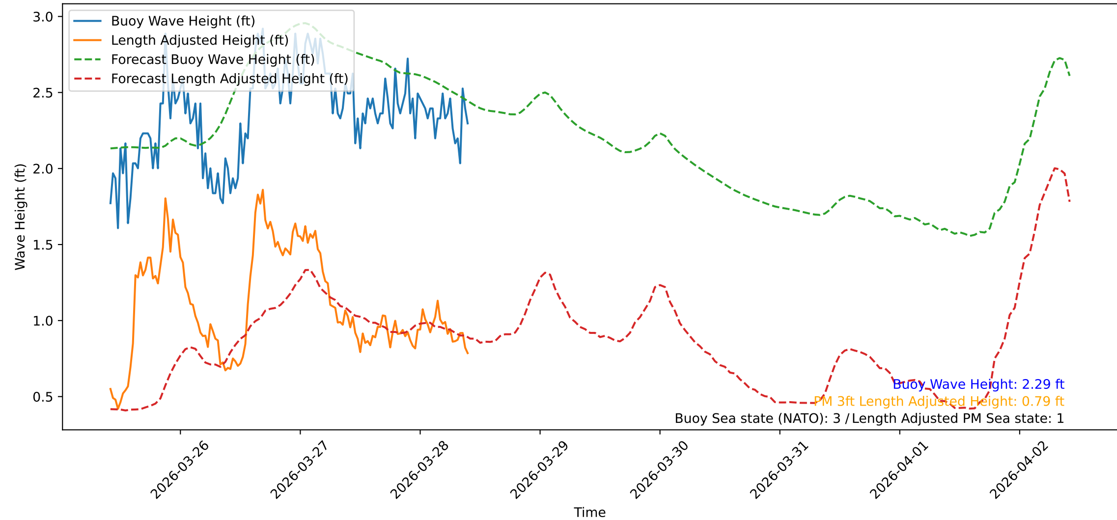
Wave Heights over Time for Oceanside Harbor at 2026-03-28 10:10:31
