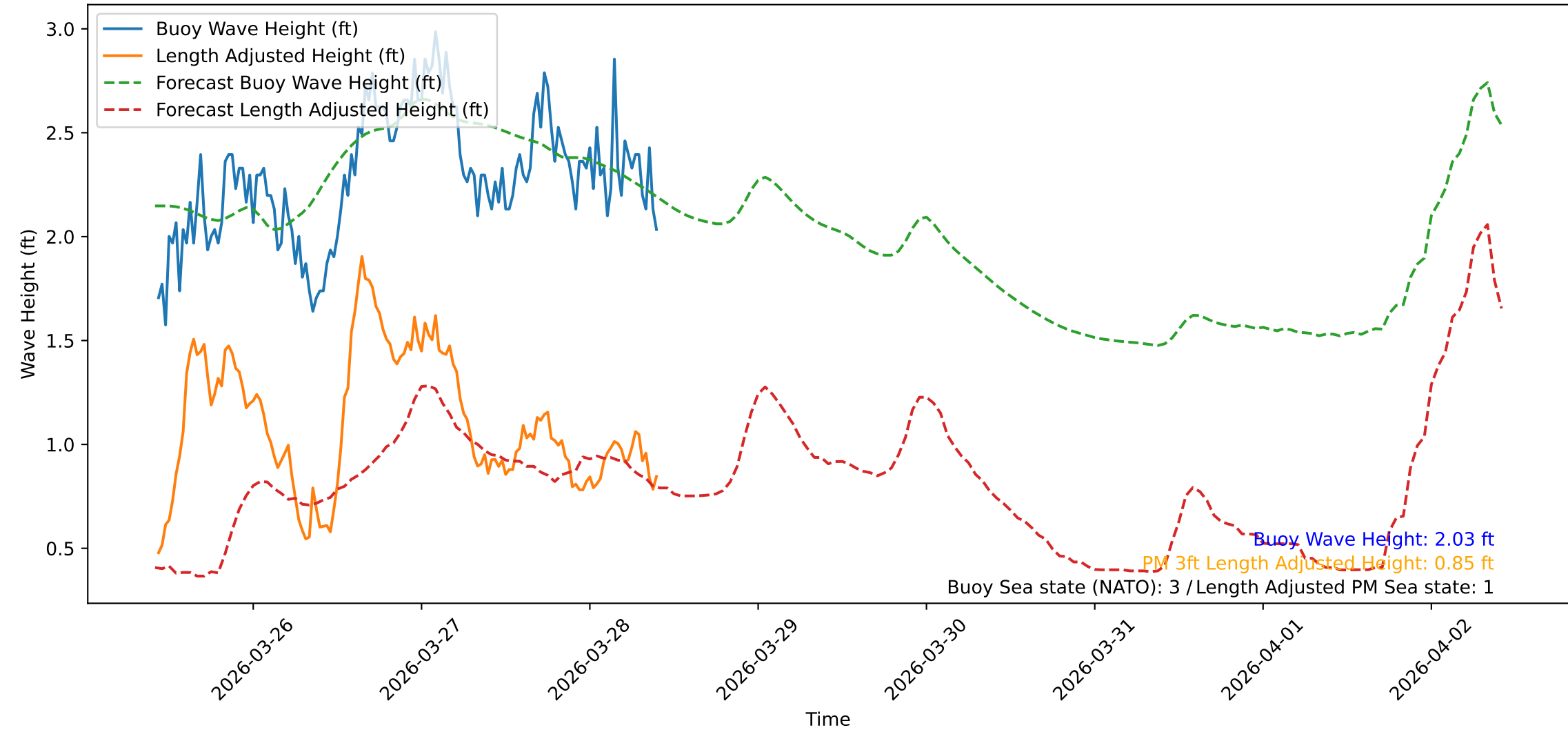
Wave Heights over Time for Red Beach at 2026-03-28 10:10:47
