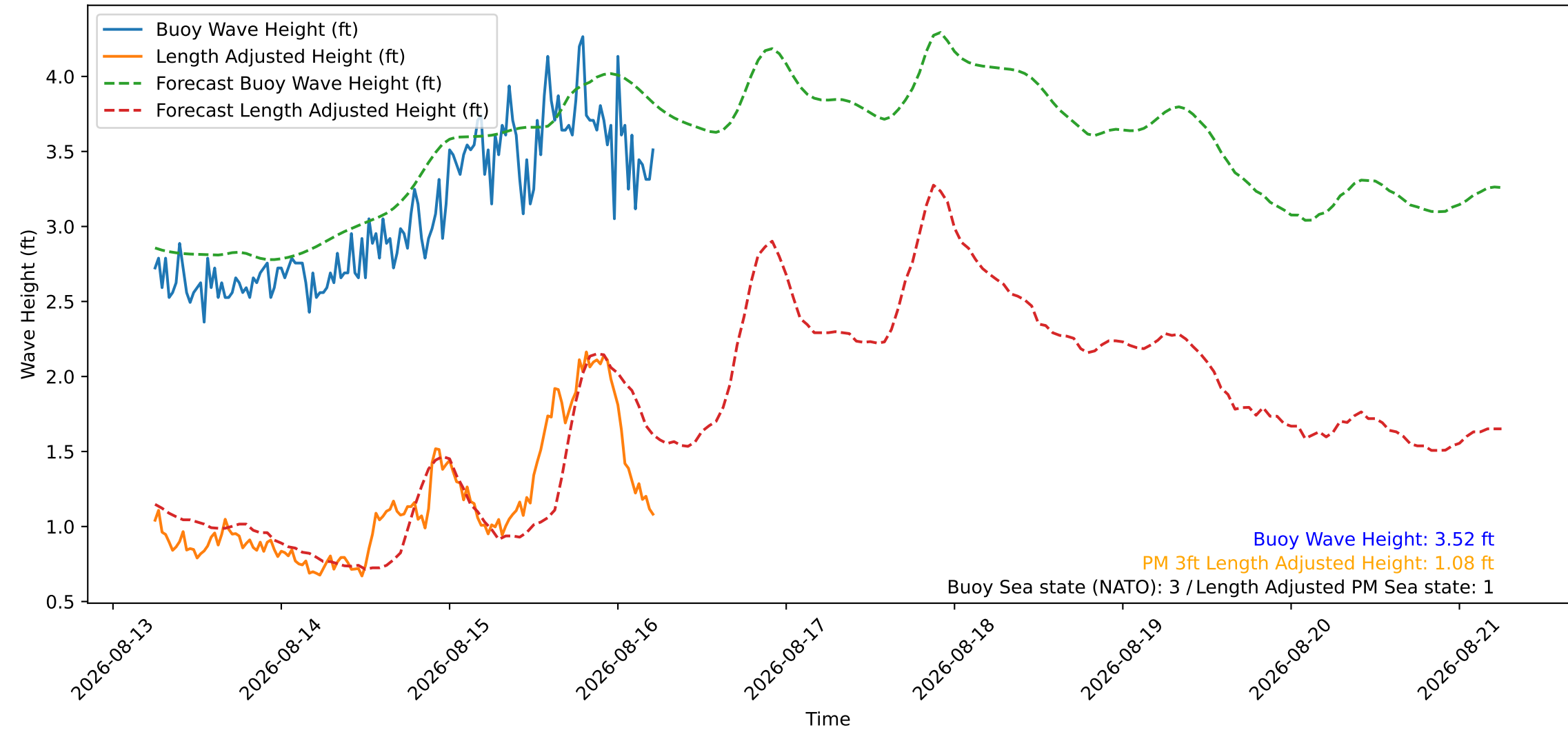
Wave Heights over Time for Green Beach at 2026-08-16 05:41:08
