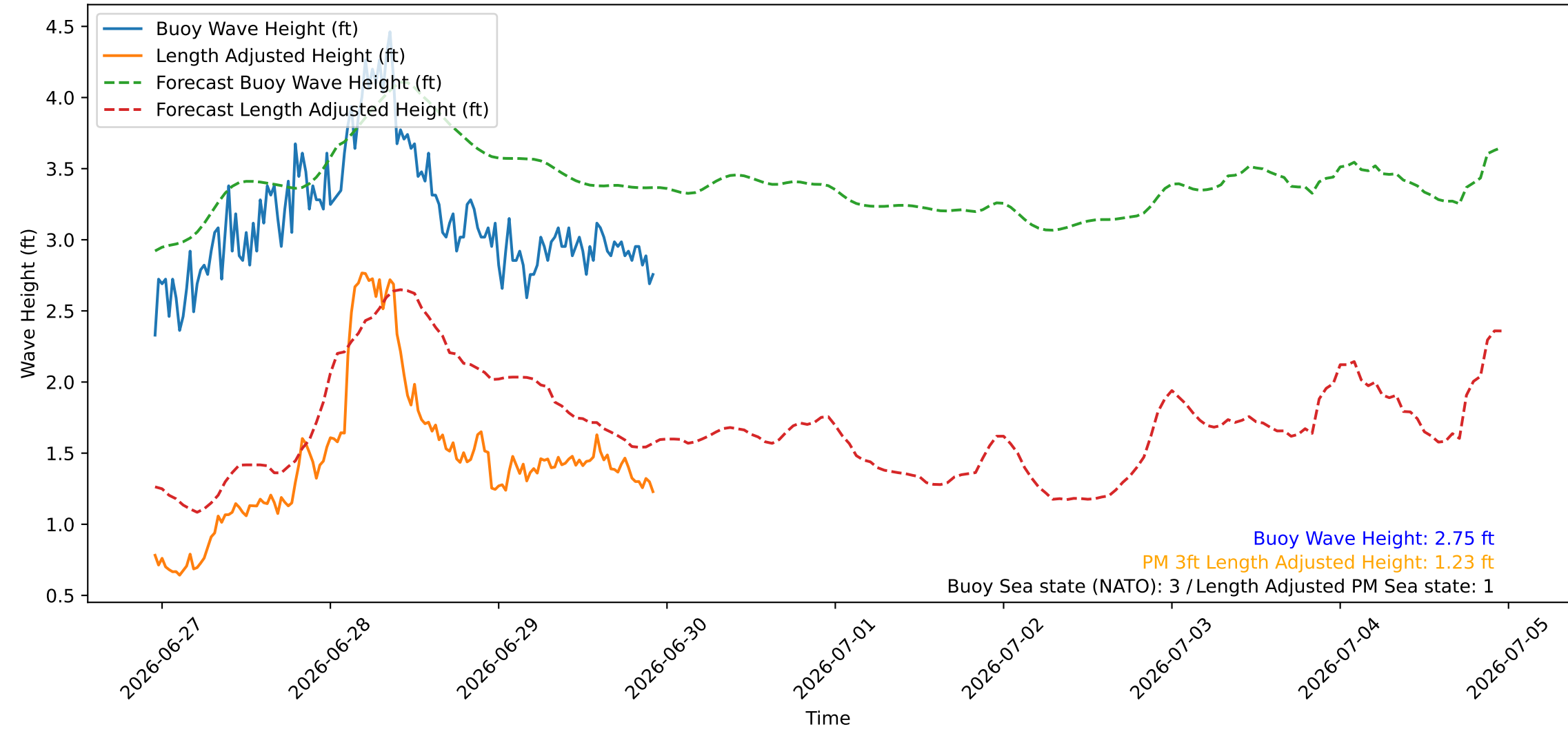
Wave Heights over Time for Red Beach at 2026-06-29 22:50:48
