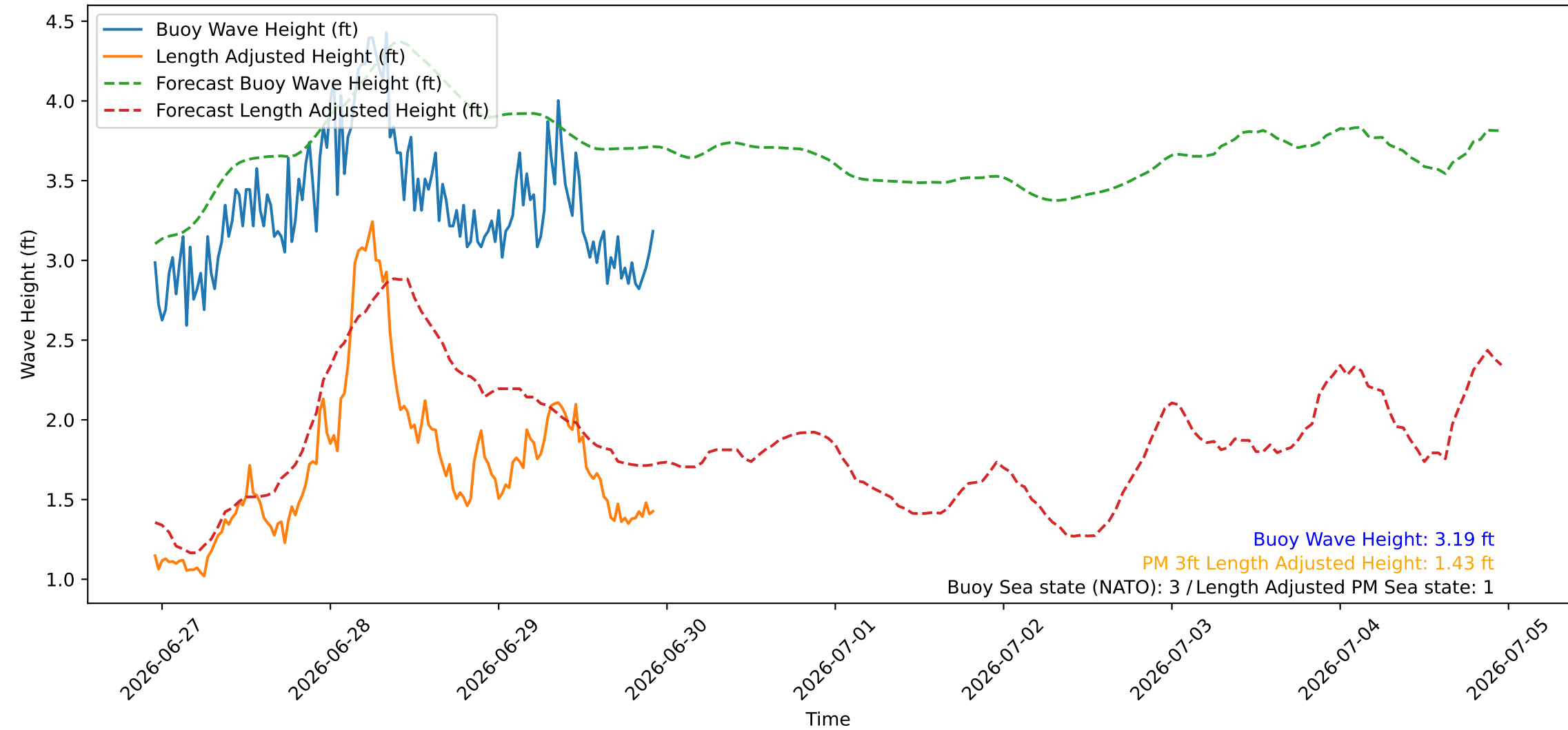
Wave Heights over Time for Oceanside Harbor at 2026-06-29 22:50:27
