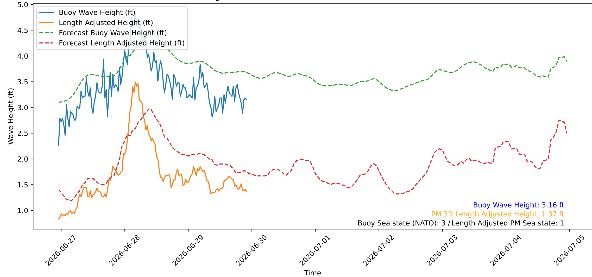
Wave Heights over Time for Green Beach at 2026-06-29 22:51:10
