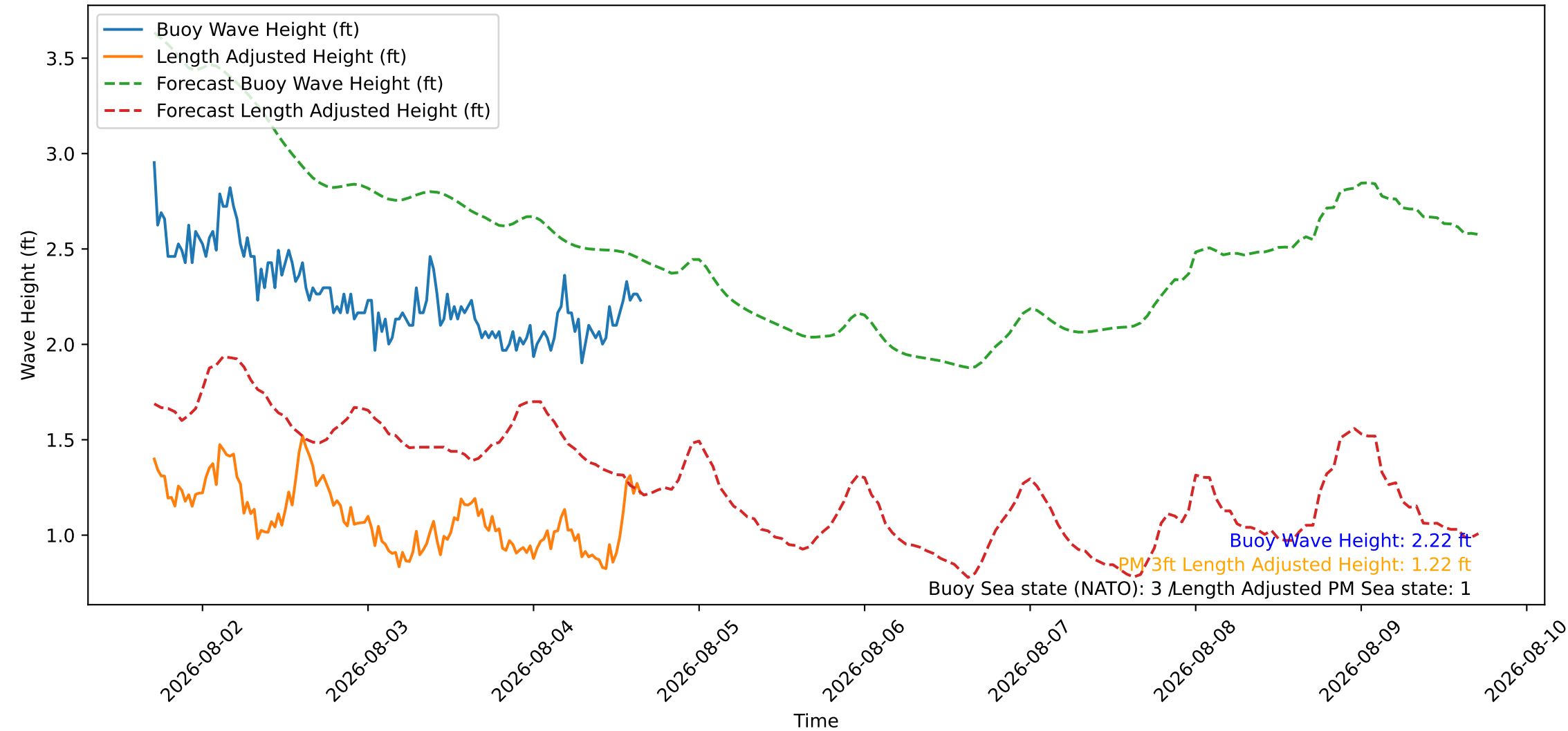
Wave Heights over Time for Red Beach at 2026-08-04 16:30:46
