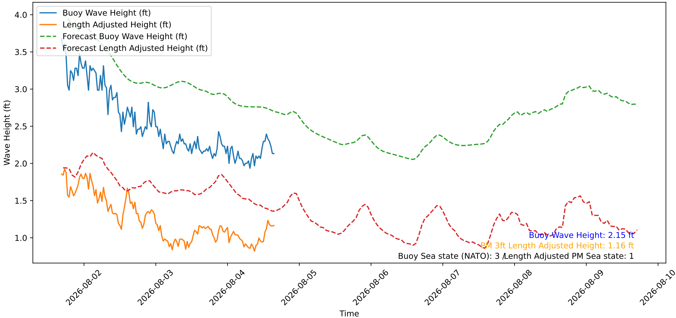
Wave Heights over Time for Green Beach at 2026-08-04 16:31:08
