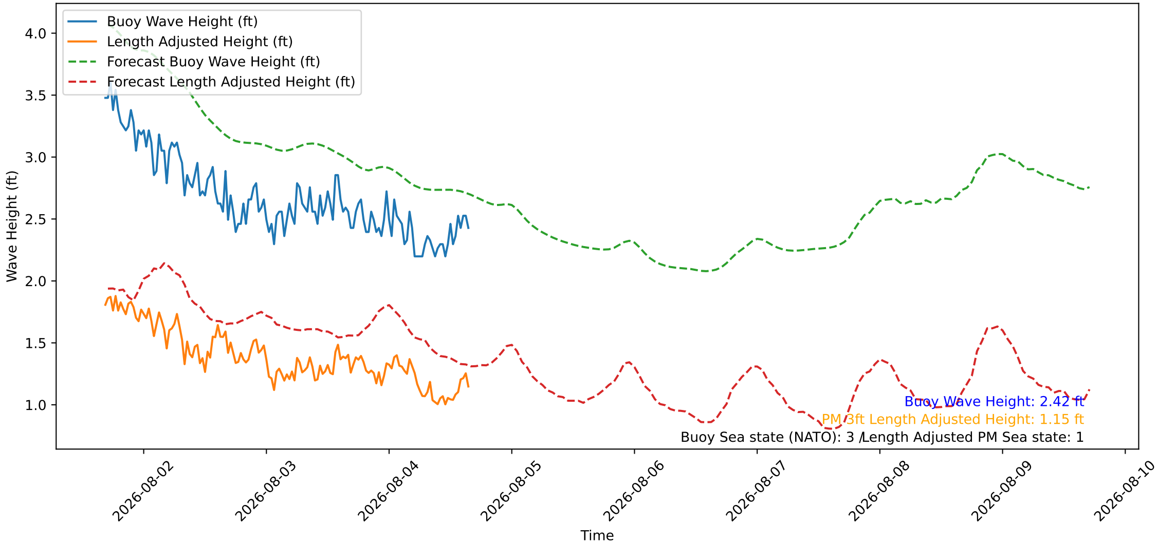
Wave Heights over Time for Oceanside Harbor at 2026-08-04 16:30:26
