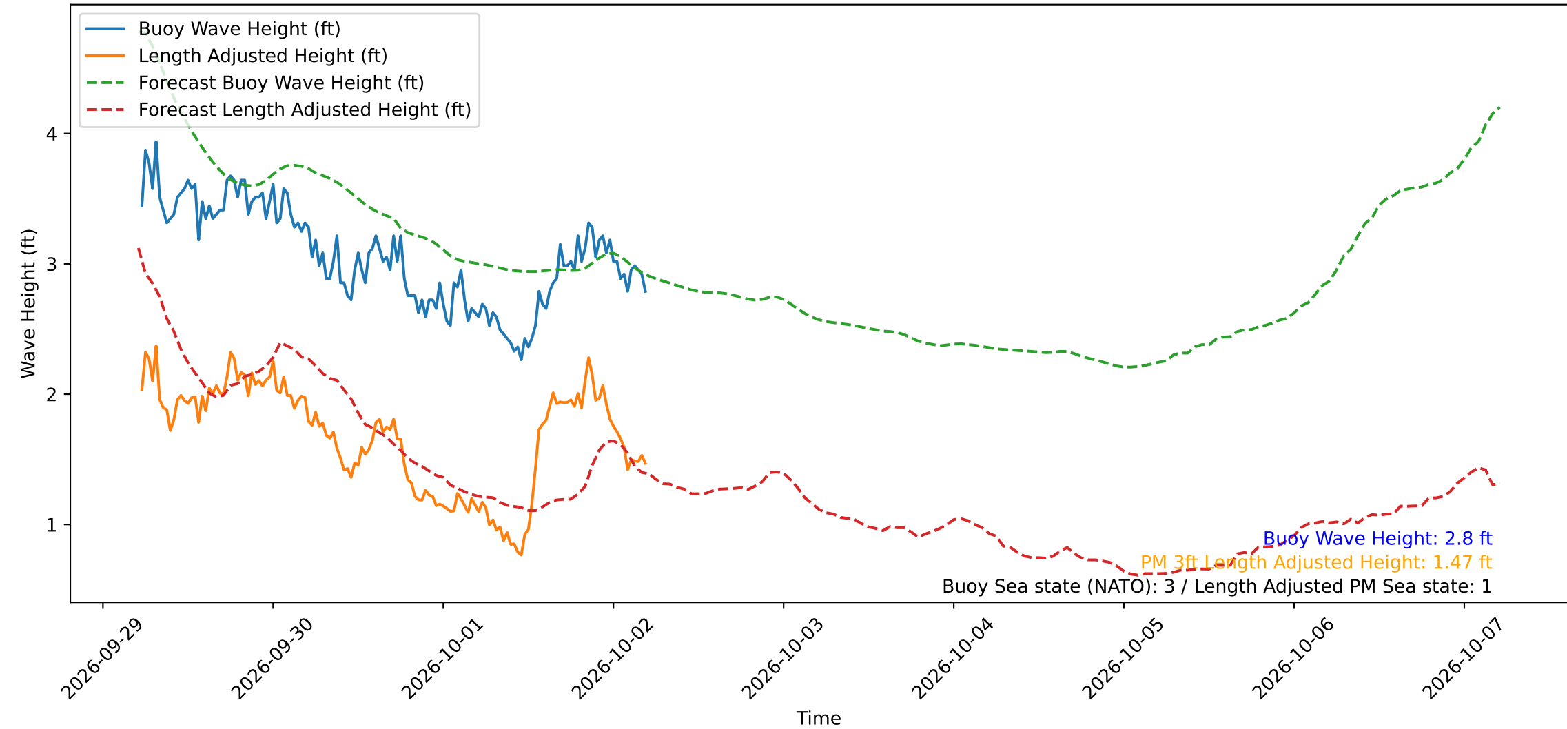
Wave Heights over Time for Oceanside Harbor at 2026-10-02 05:20:29
