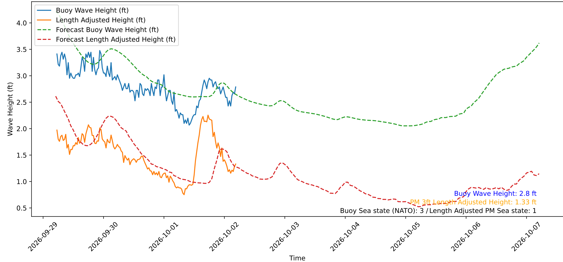
Wave Heights over Time for Red Beach at 2026-10-02 05:20:50
