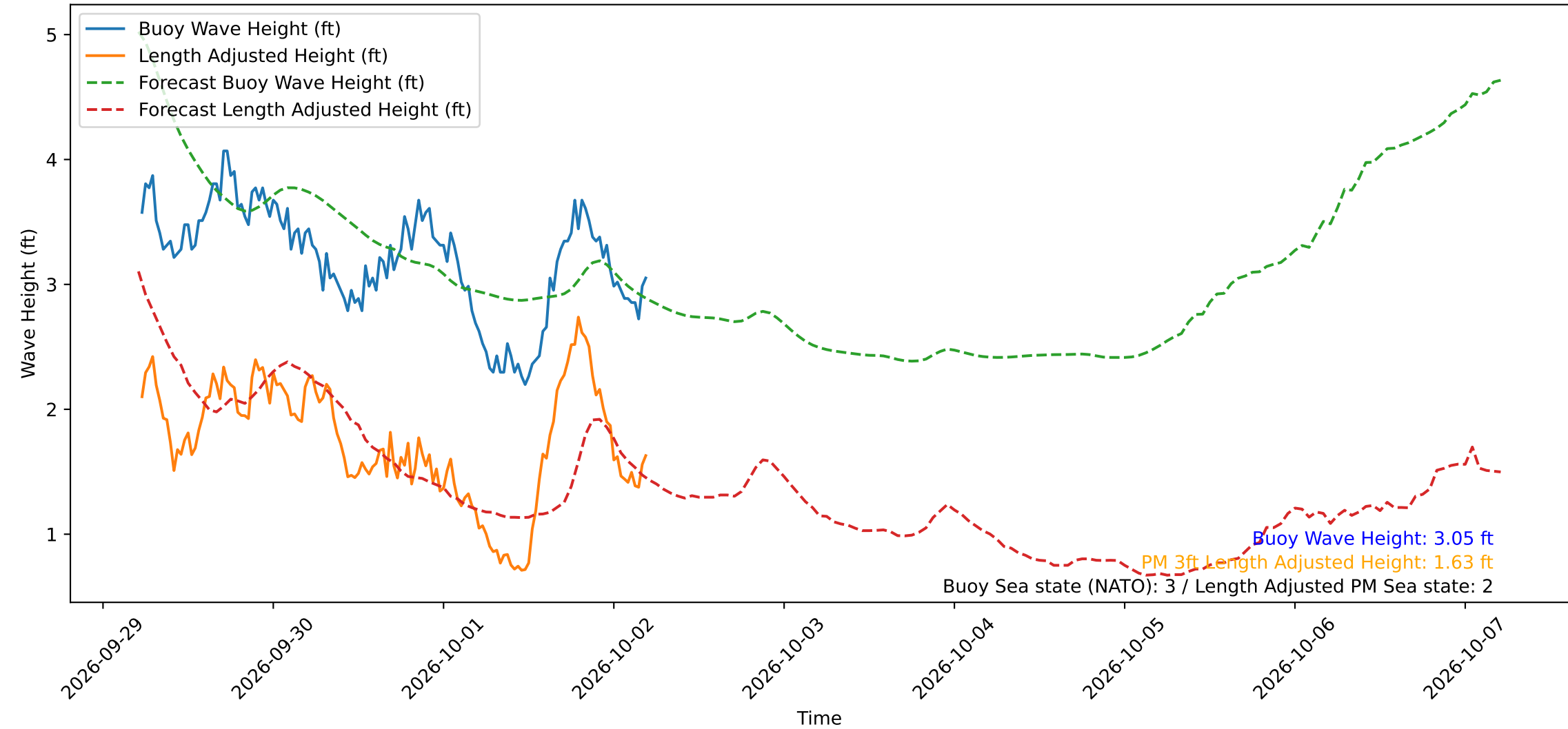
Wave Heights over Time for Green Beach at 2026-10-02 05:21:14
