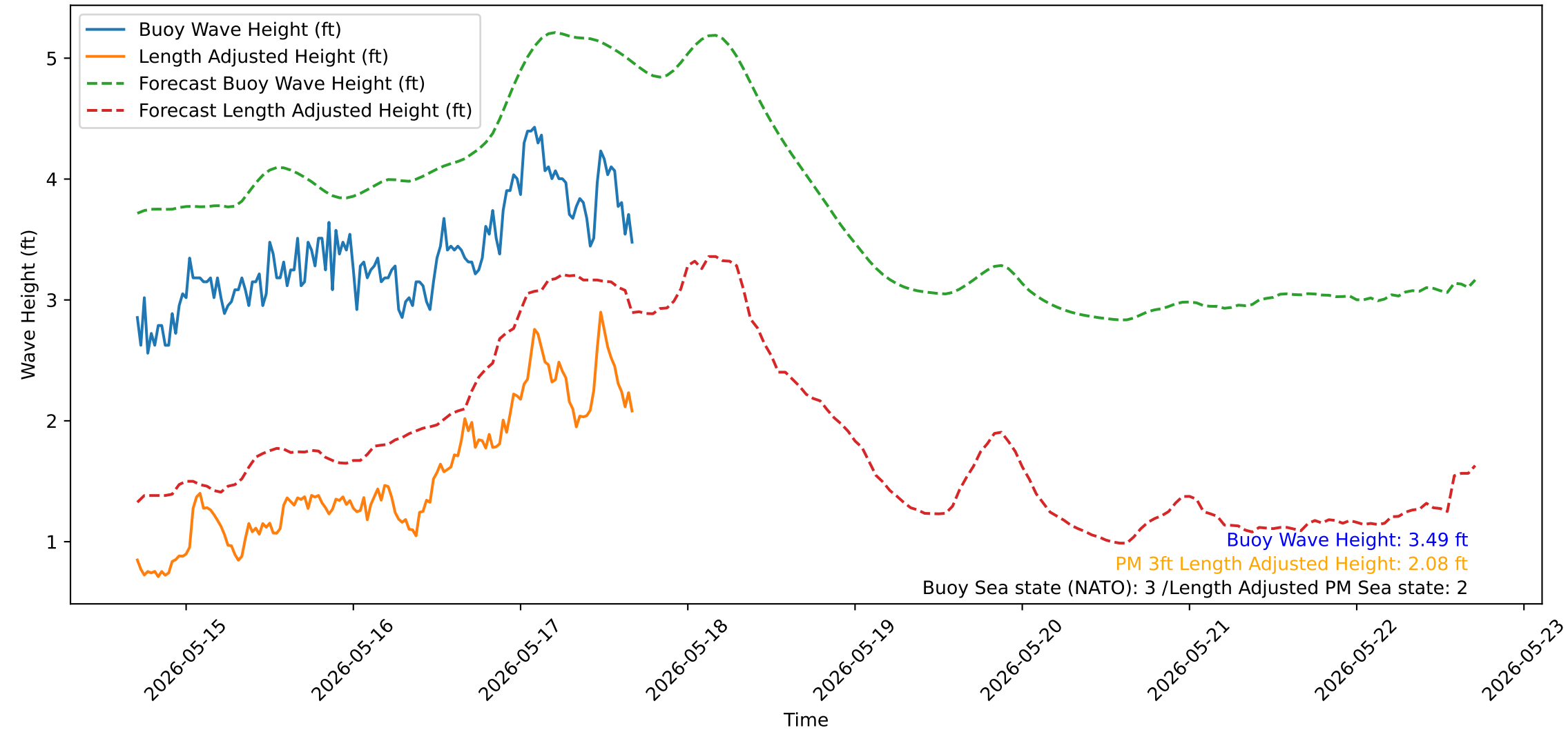
Wave Heights over Time for Green Beach at 2026-05-17 16:51:14
