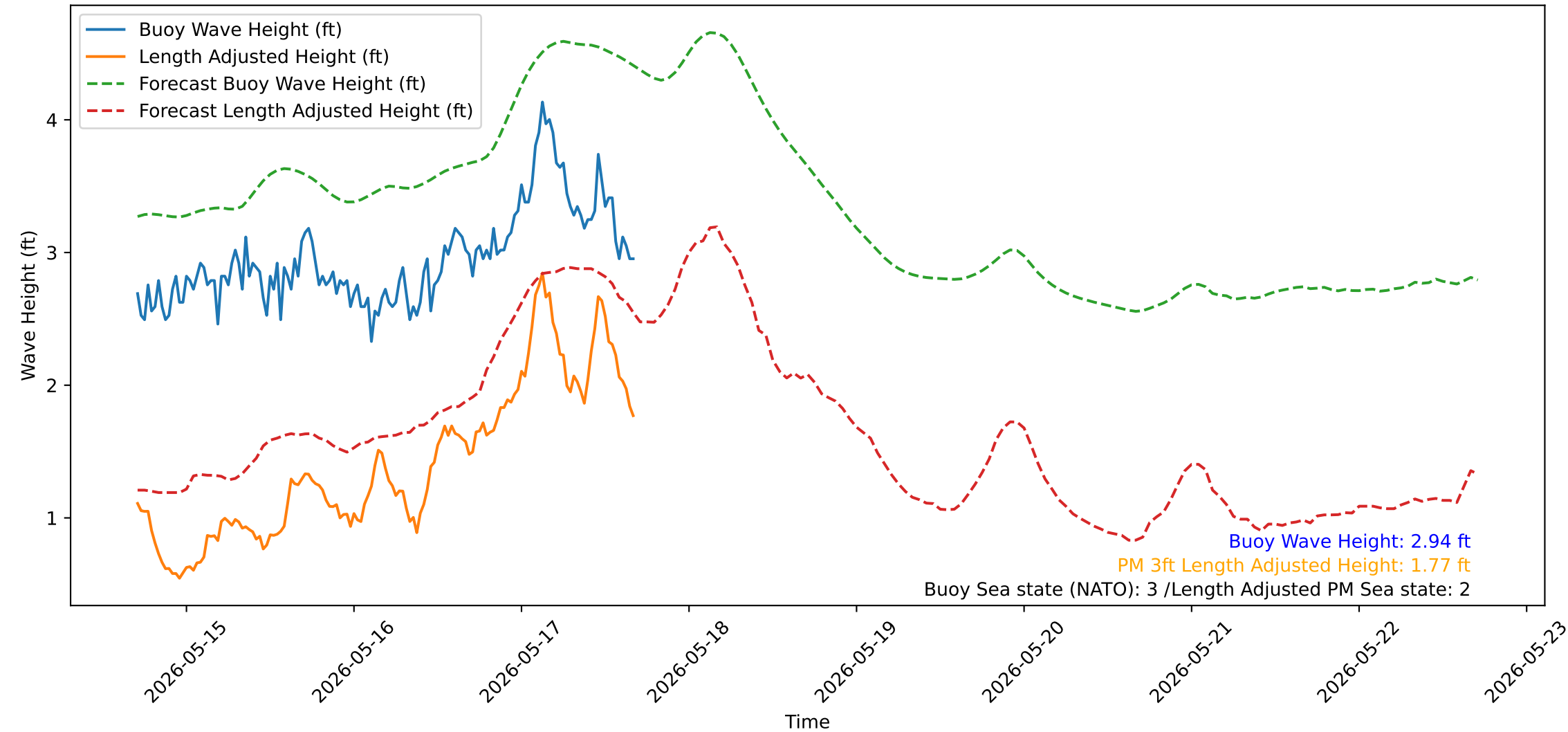
Wave Heights over Time for Red Beach at 2026-05-17 16:50:51
