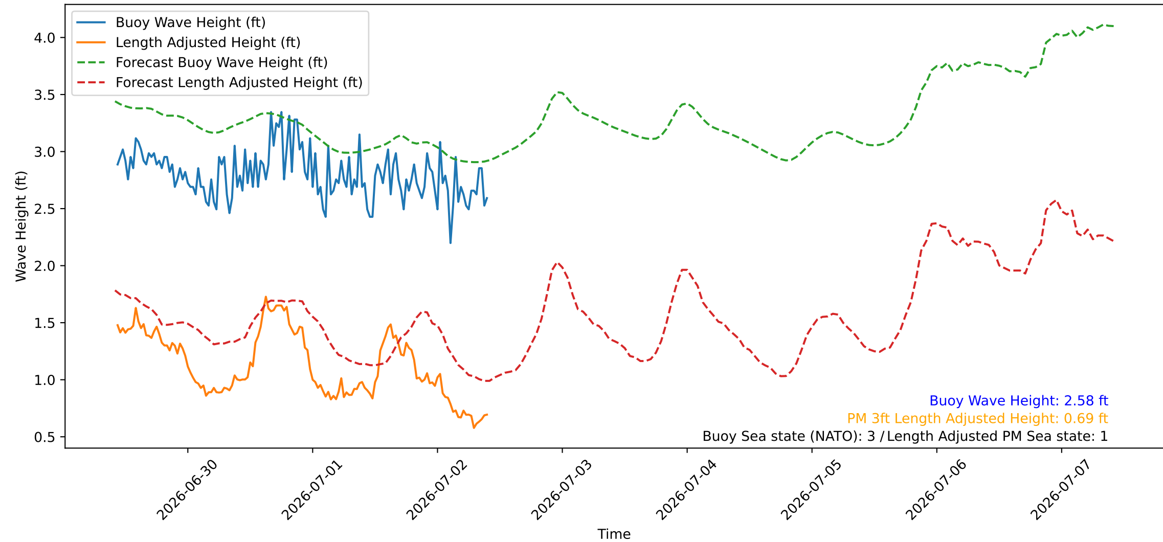
Wave Heights over Time for Red Beach at 2026-07-02 10:20:47
