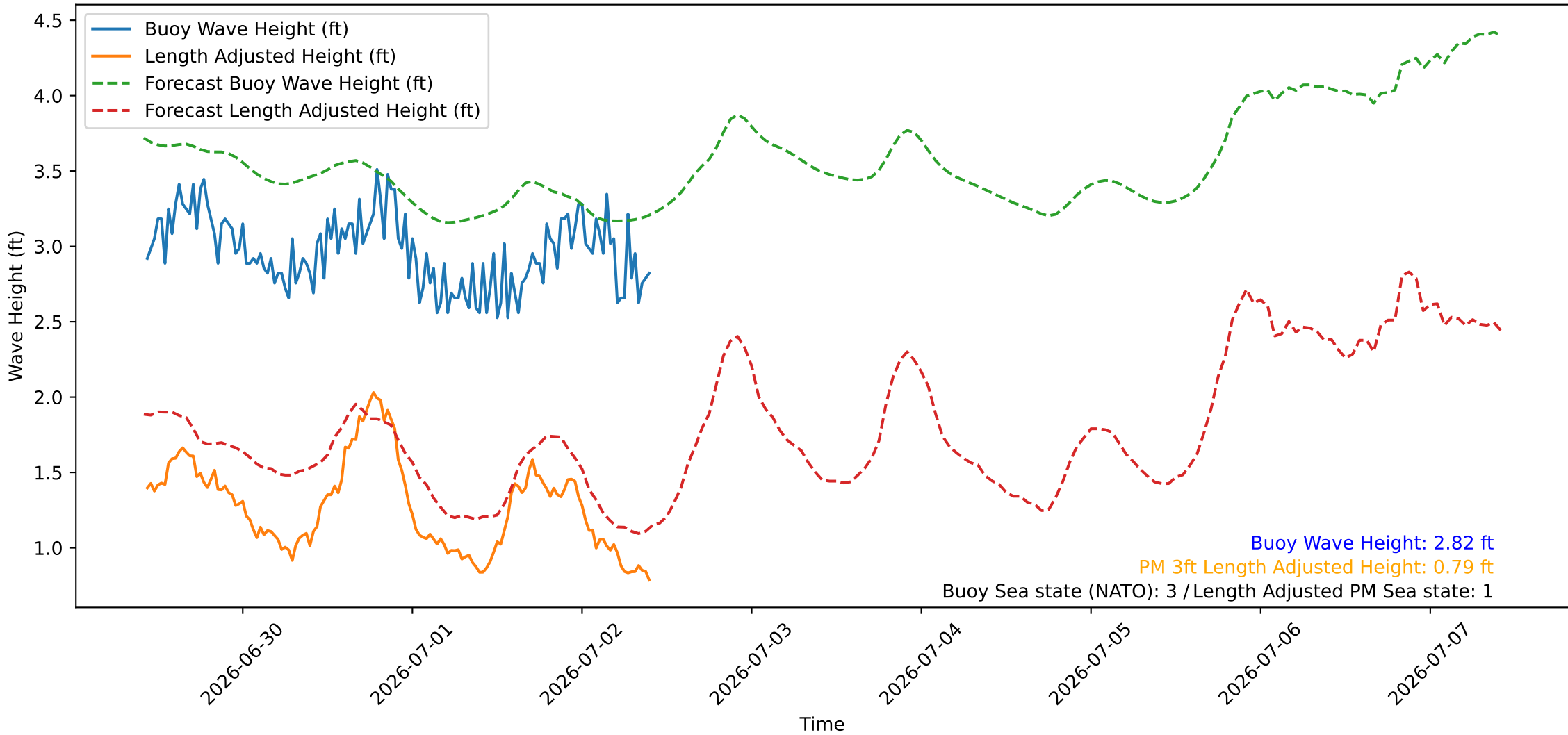
Wave Heights over Time for Green Beach at 2026-07-02 10:21:09
