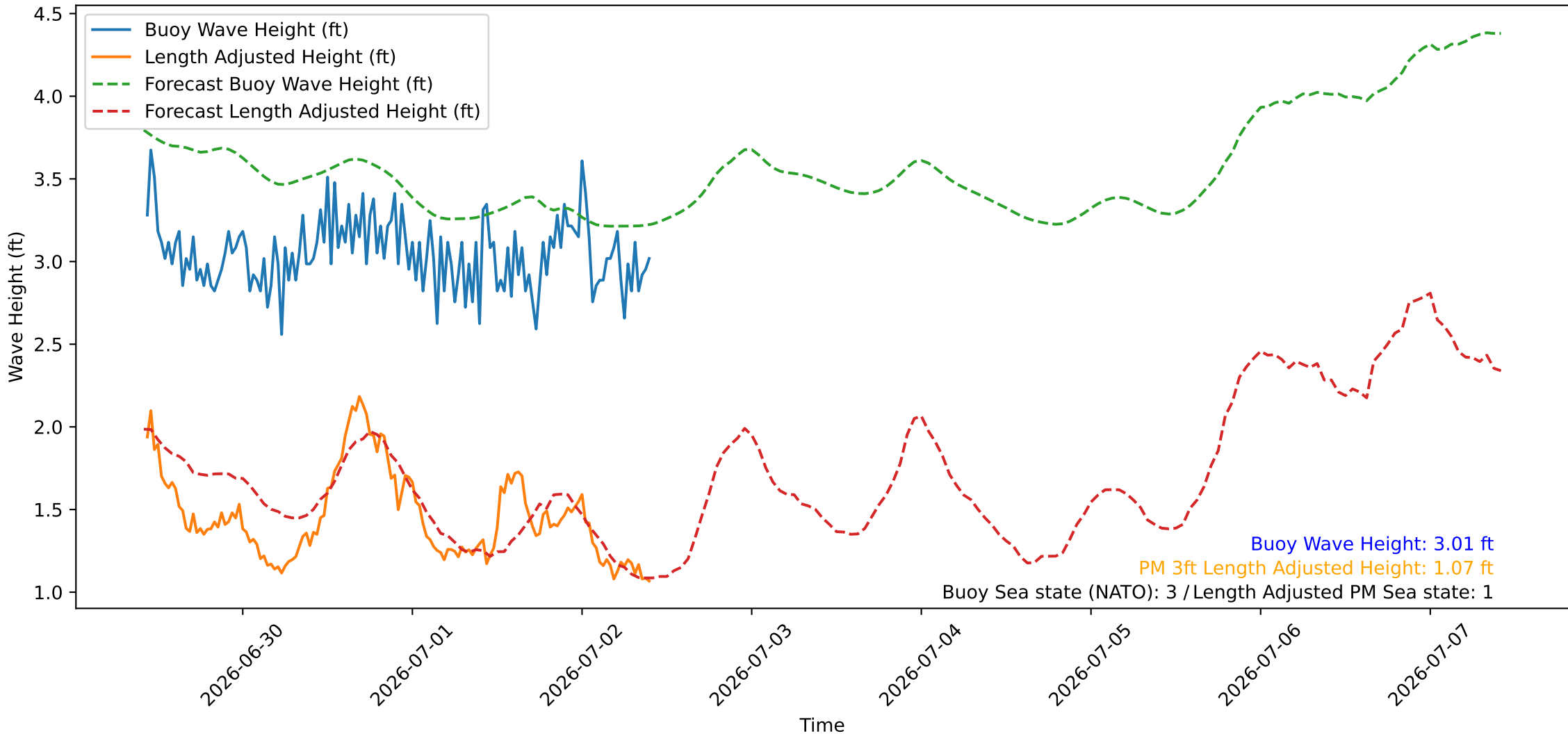
Wave Heights over Time for Oceanside Harbor at 2026-07-02 10:20:27
