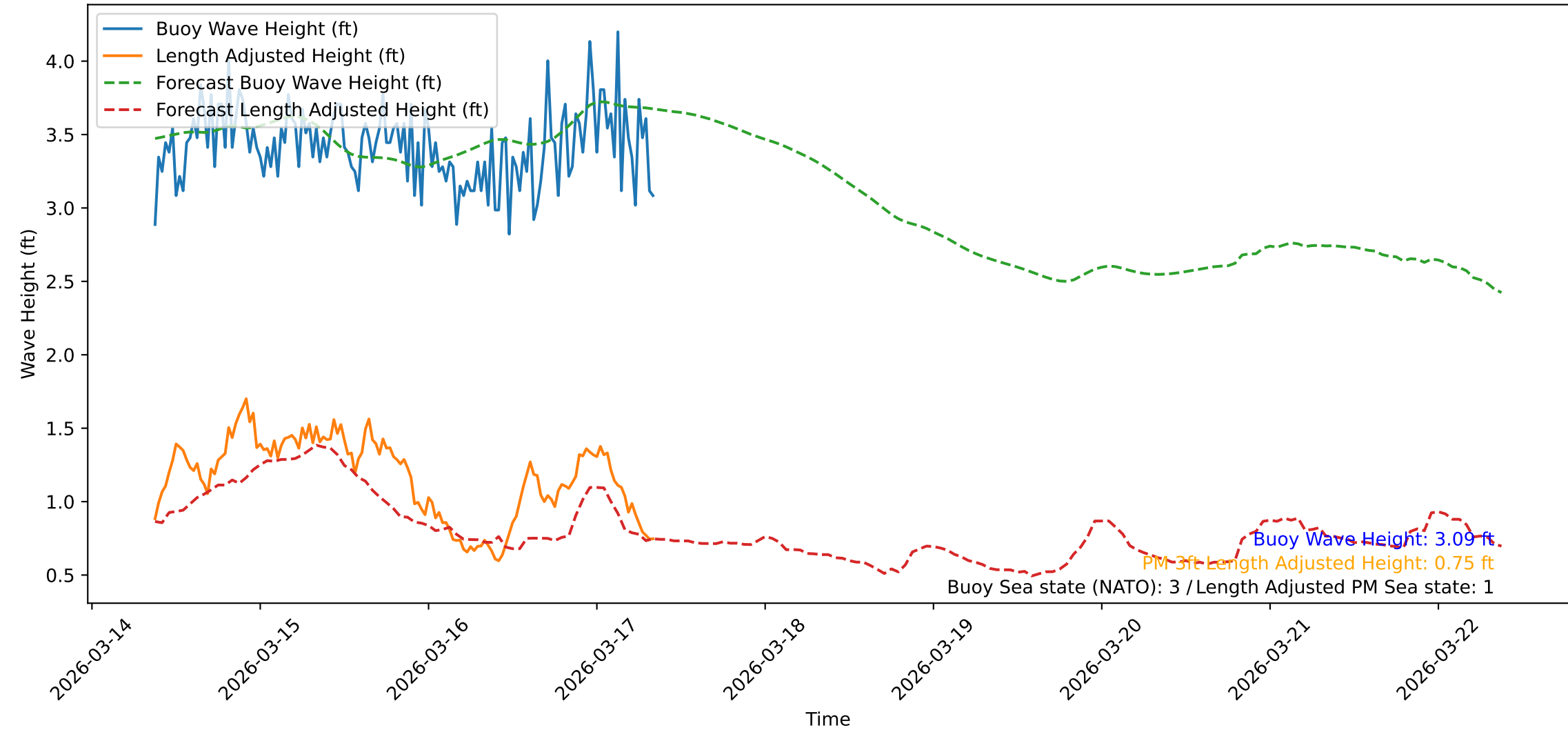
Wave Heights over Time for Green Beach at 2026-03-17 09:01:47
