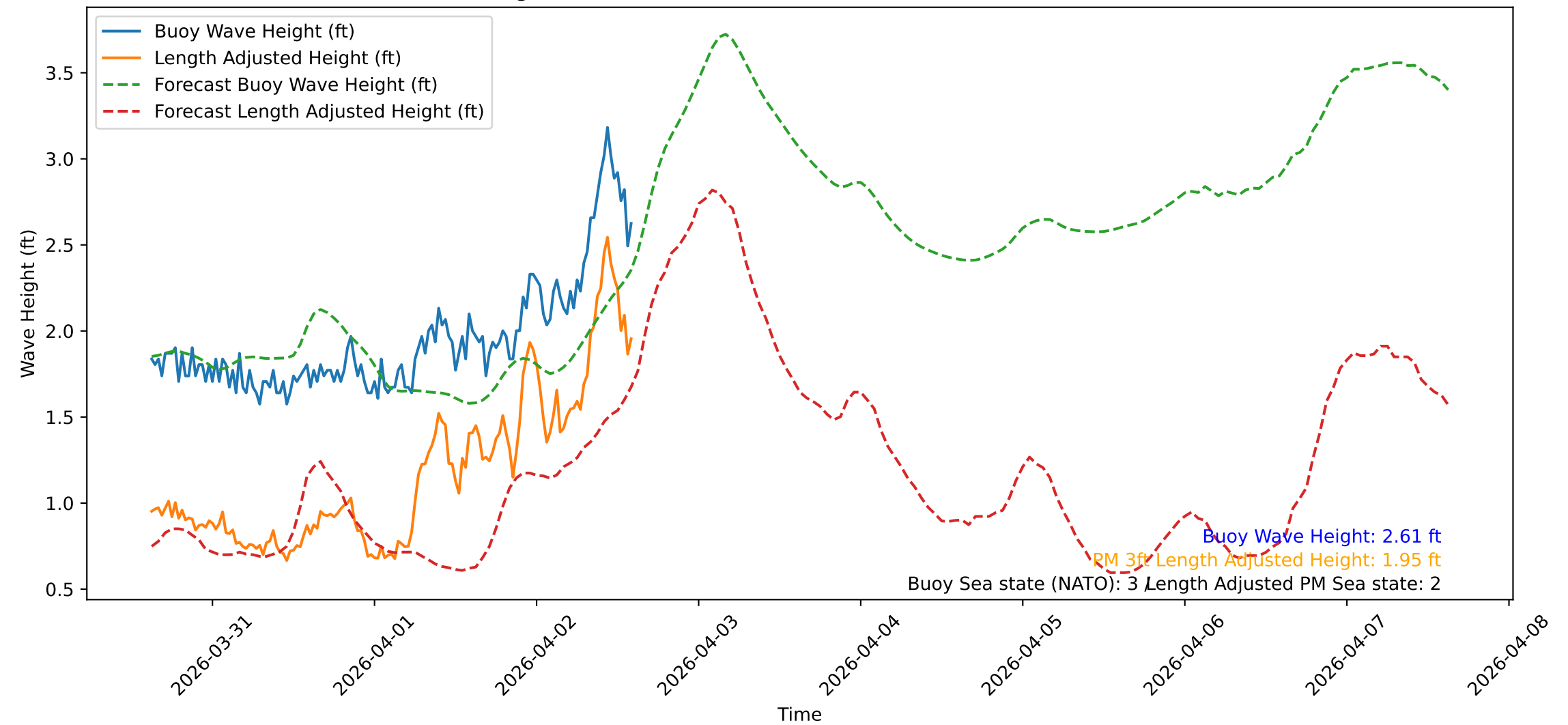
Wave Heights over Time for Oceanside Harbor at 2026-04-02 14:50:31
