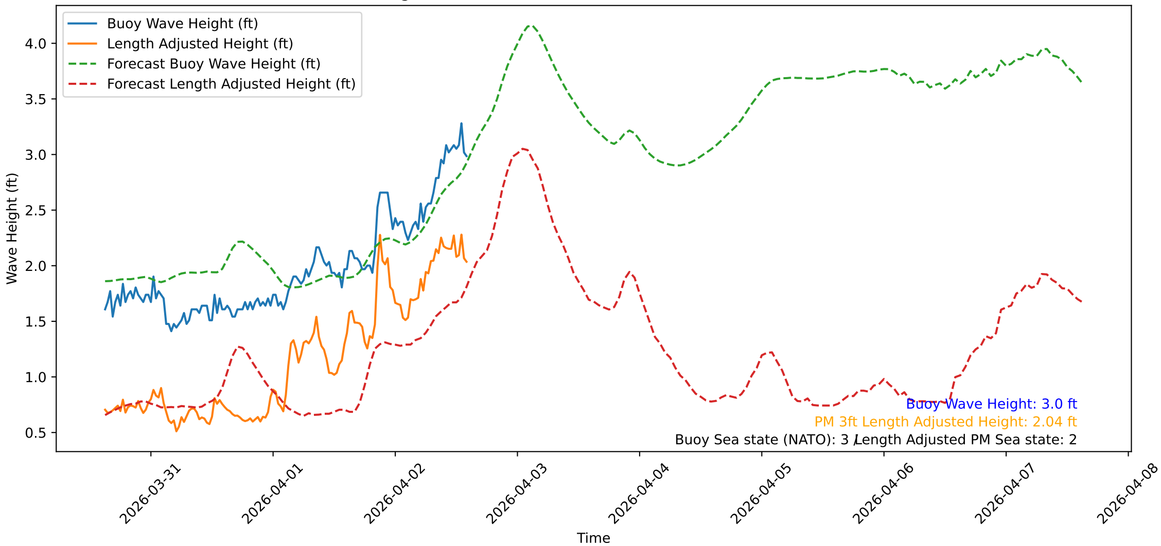
Wave Heights over Time for Green Beach at 2026-04-02 14:51:09
