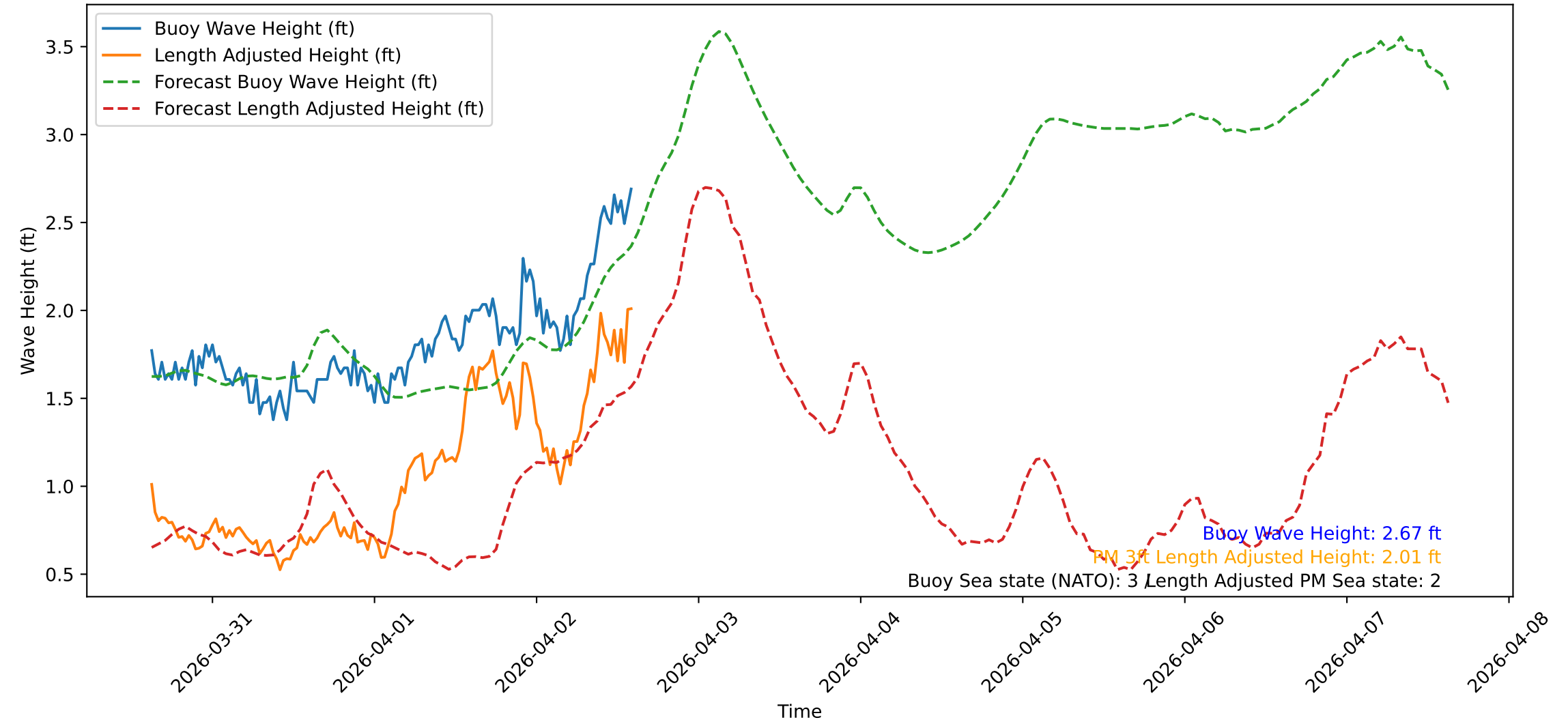
Wave Heights over Time for Red Beach at 2026-04-02 14:50:47
