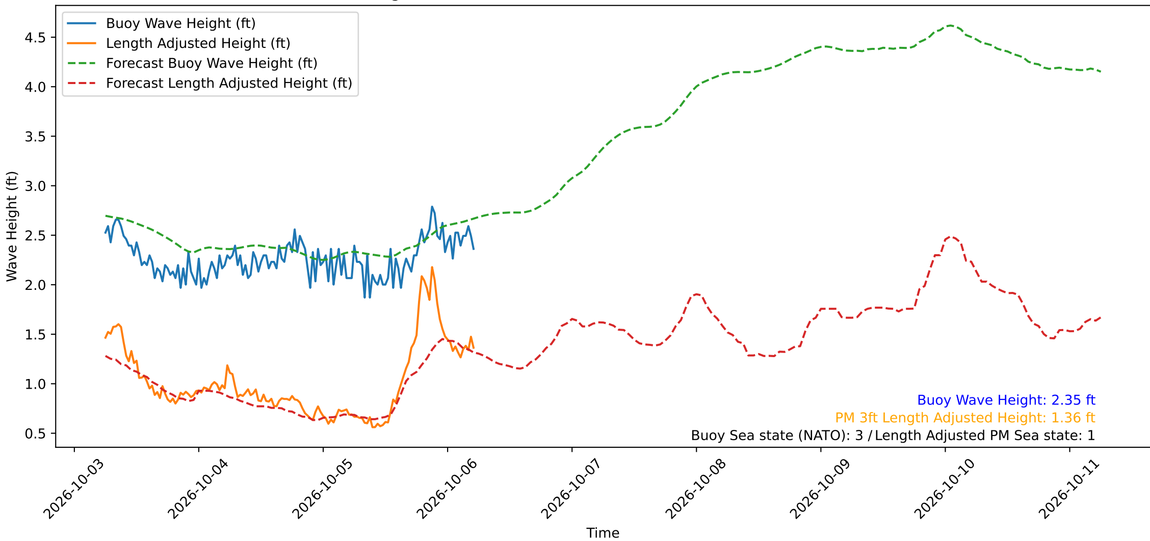
Wave Heights over Time for Oceanside Harbor at 2026-10-06 06:00:29
