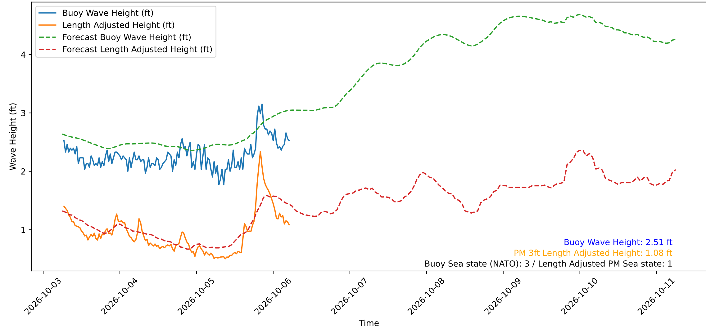
Wave Heights over Time for Green Beach at 2026-10-06 06:01:11
