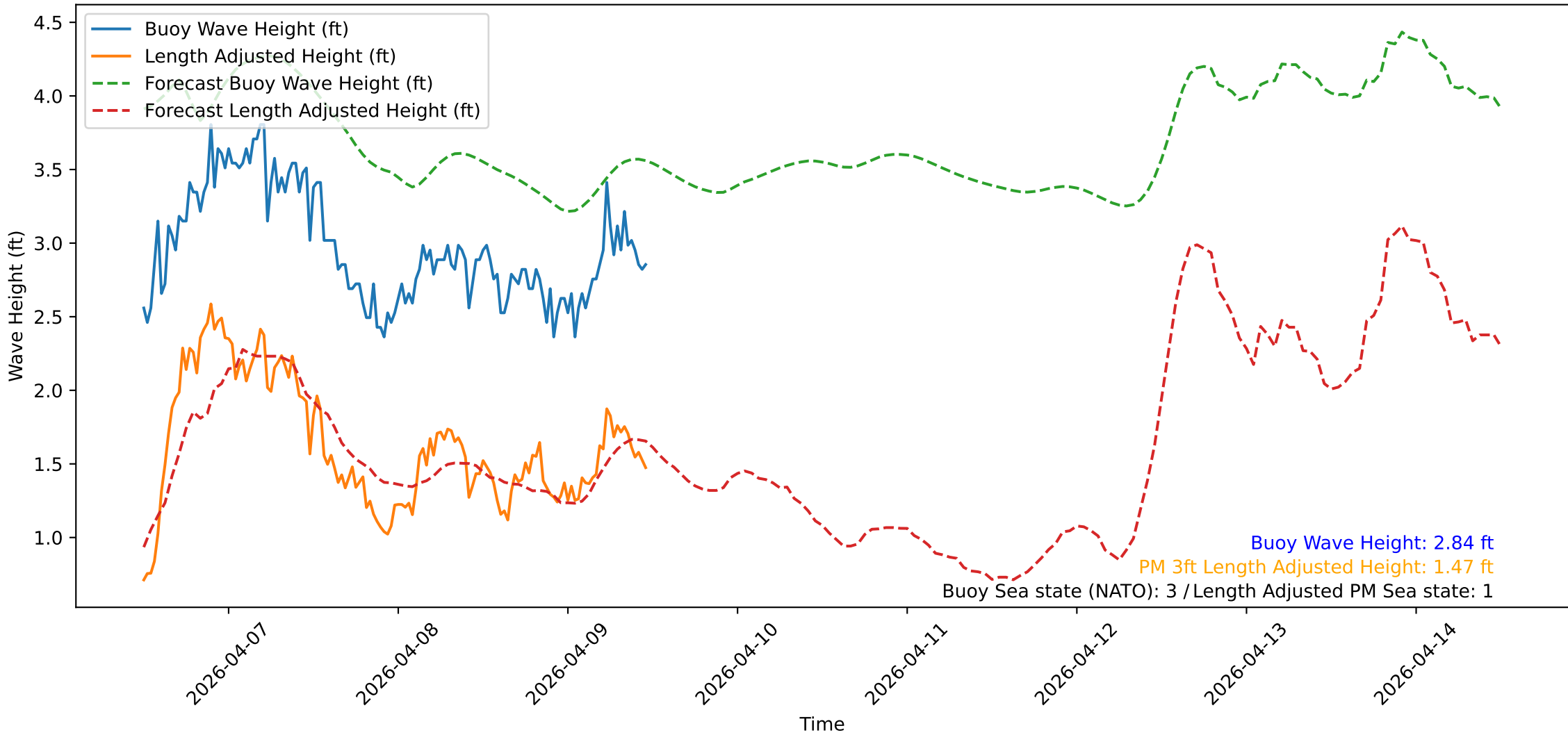
Wave Heights over Time for Green Beach at 2026-04-09 11:51:09
