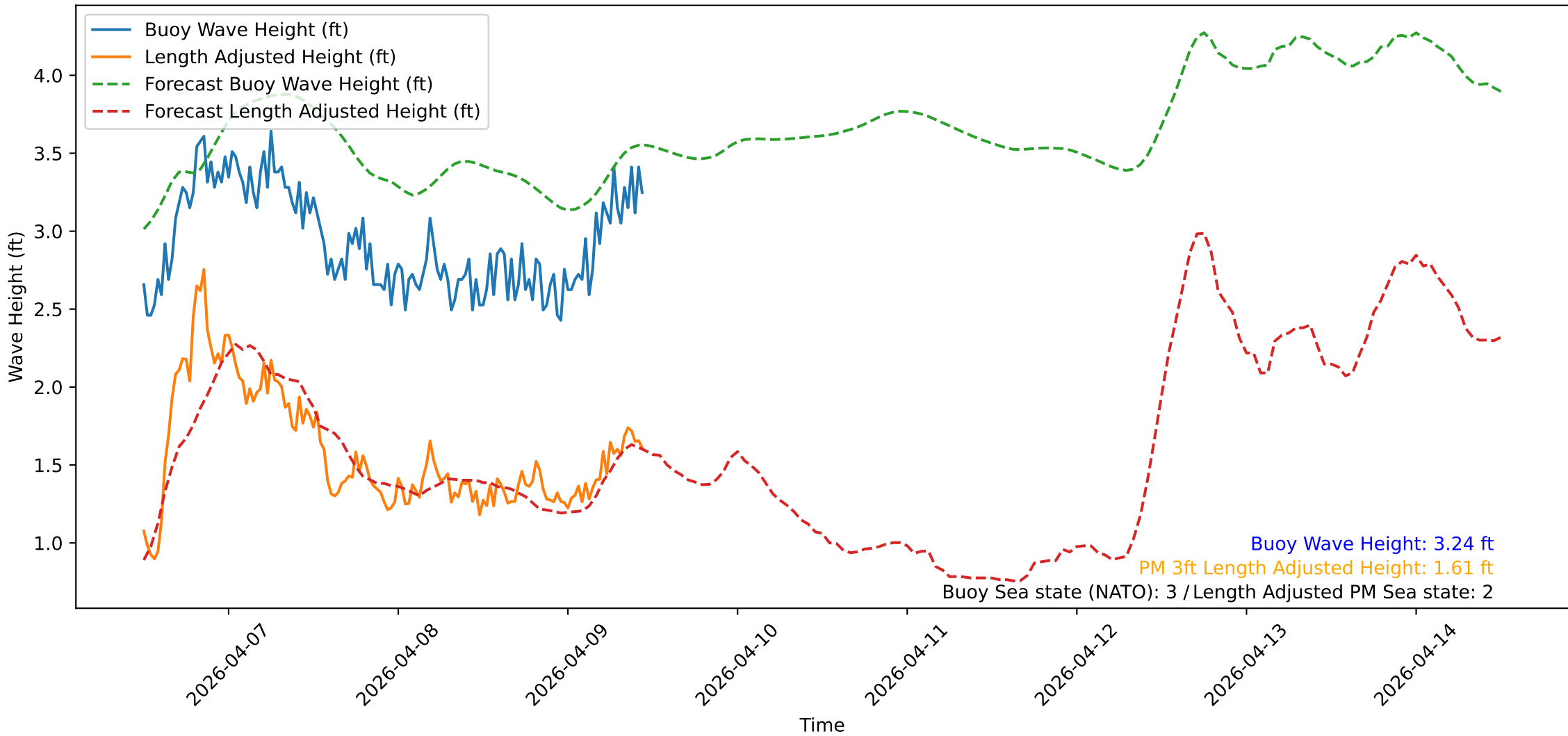
Wave Heights over Time for Oceanside Harbor at 2026-04-09 11:50:31
