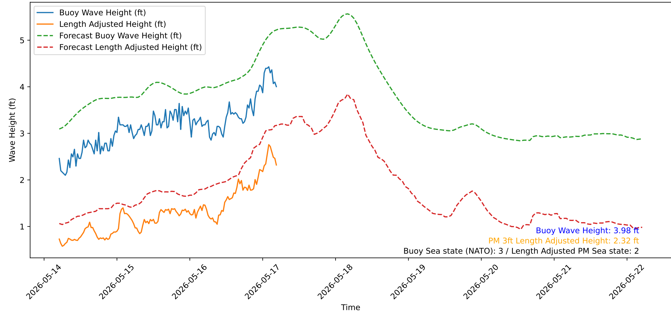
Wave Heights over Time for Green Beach at 2026-05-17 05:11:13
