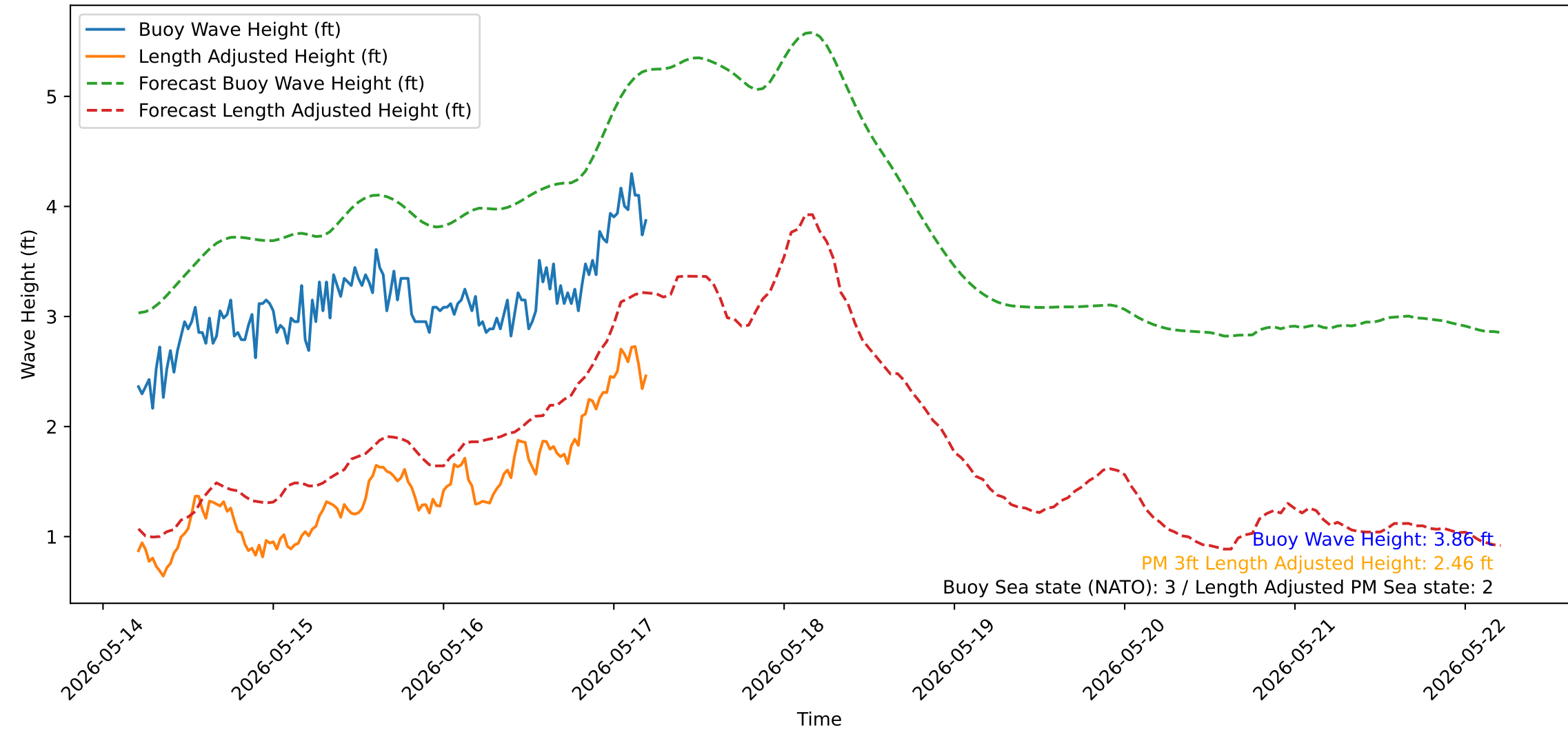
Wave Heights over Time for Oceanside Harbor at 2026-05-17 05:10:31
