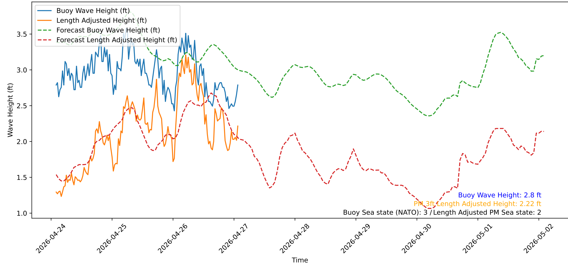
Wave Heights over Time for Green Beach at 2026-04-27 02:11:12
