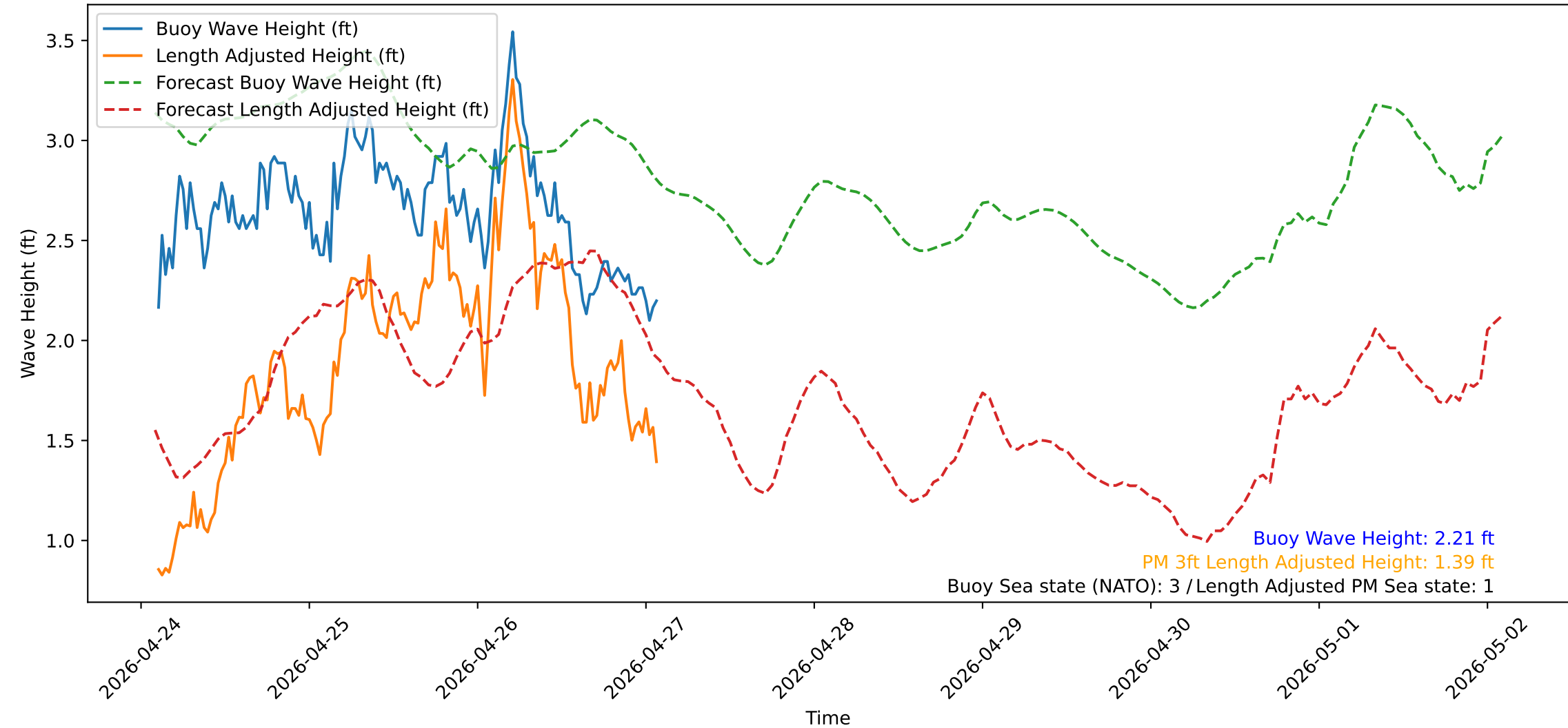
Wave Heights over Time for Red Beach at 2026-04-27 02:10:50
