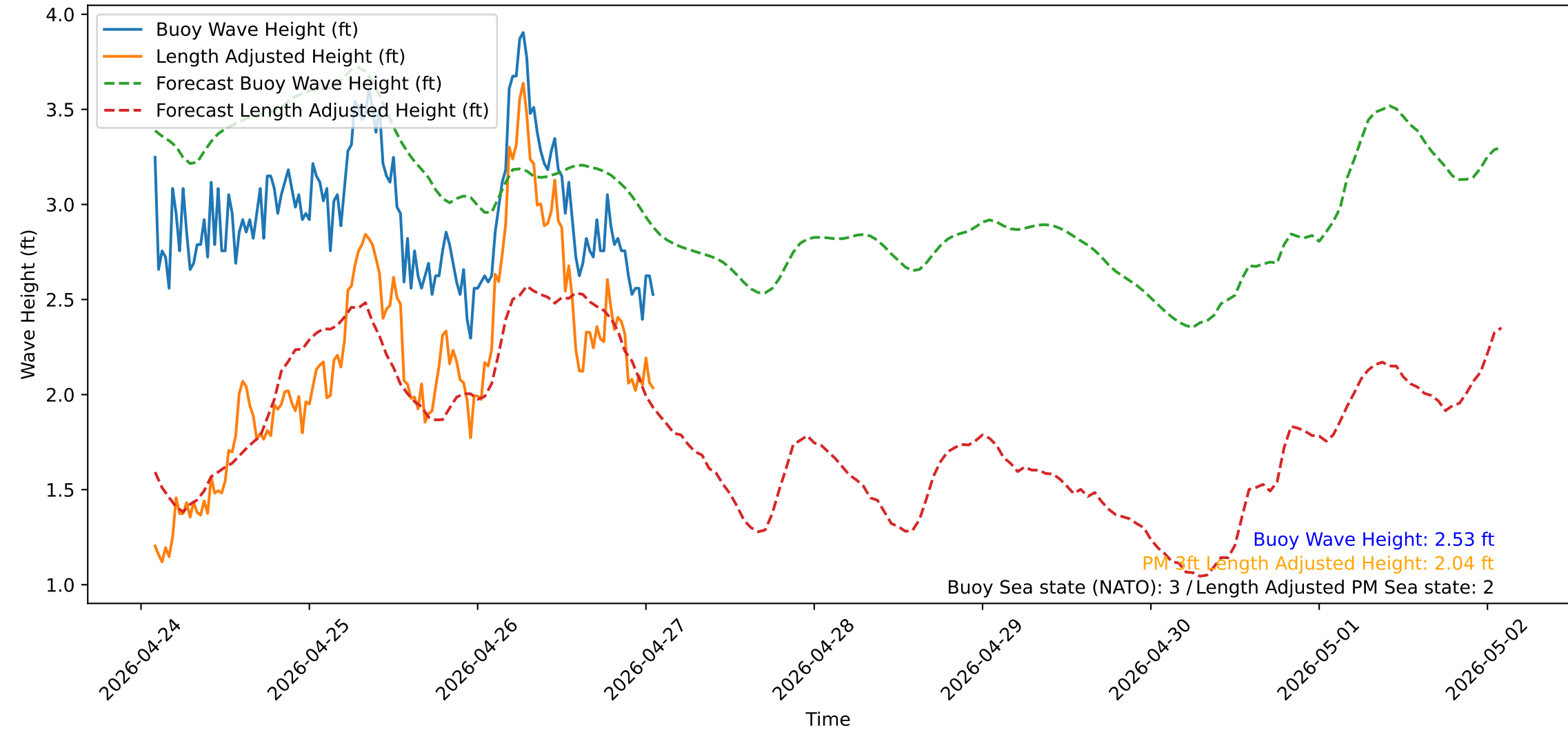
Wave Heights over Time for Oceanside Harbor at 2026-04-27 02:10:31
