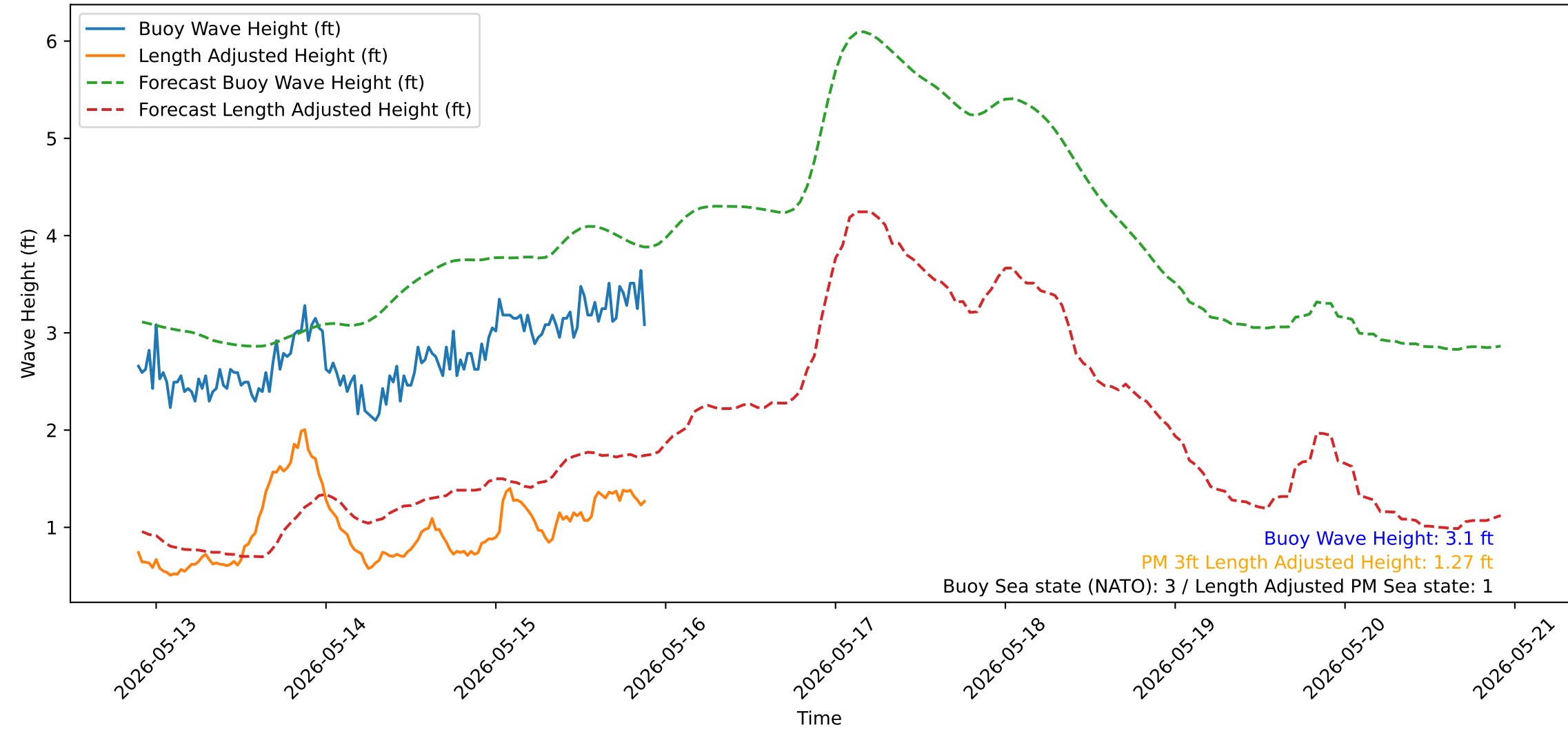
Wave Heights over Time for Green Beach at 2026-05-15 21:41:14
