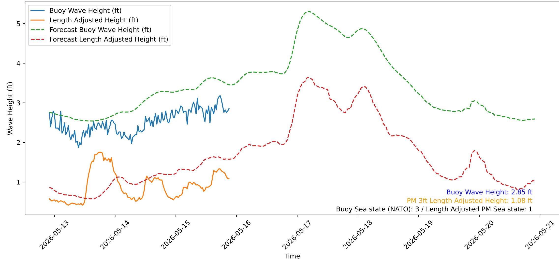
Wave Heights over Time for Red Beach at 2026-05-15 21:40:51
