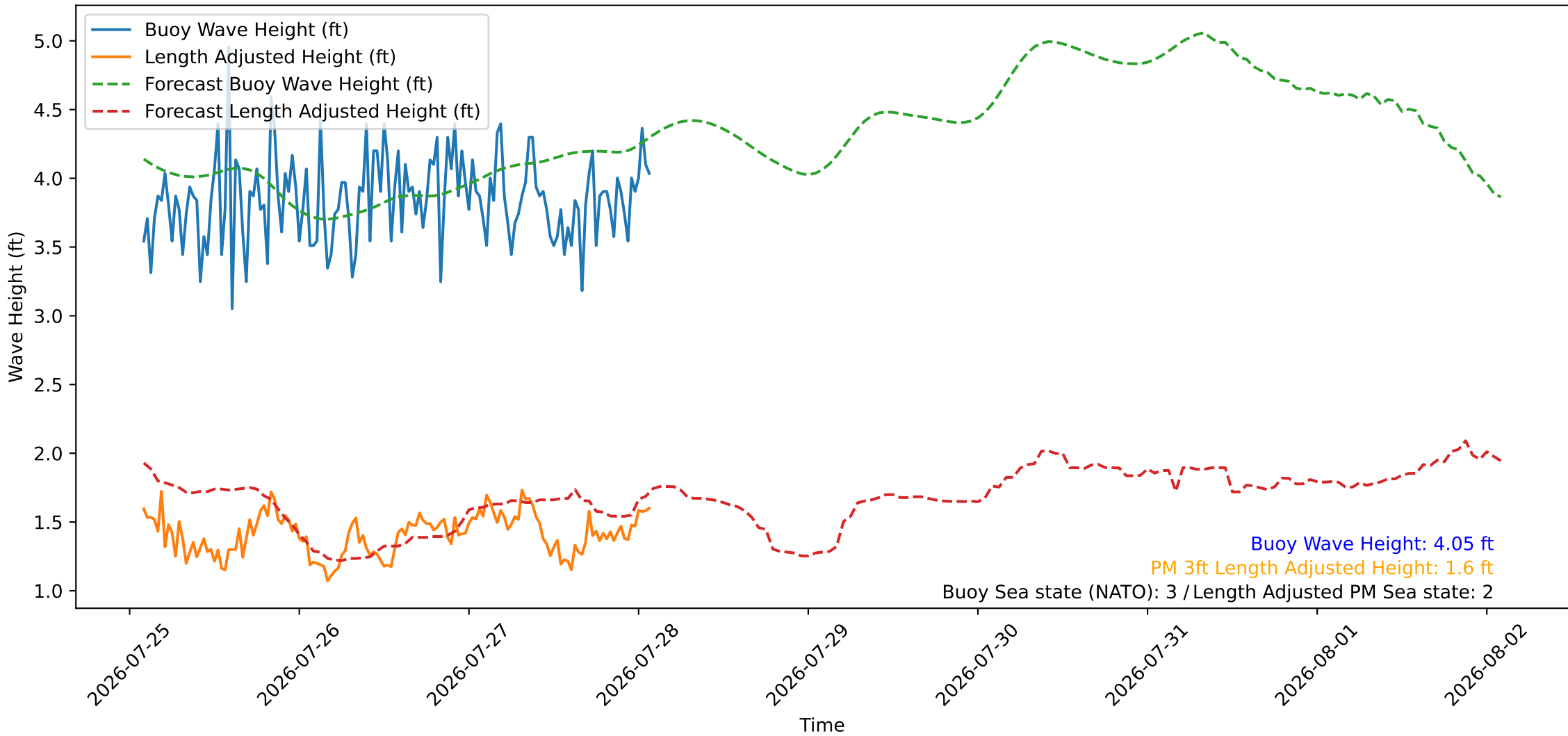
Wave Heights over Time for Oceanside Harbor at 2026-07-28 02:10:26
