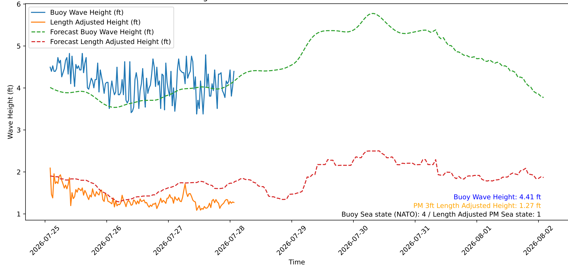
Wave Heights over Time for Green Beach at 2026-07-28 02:11:08
