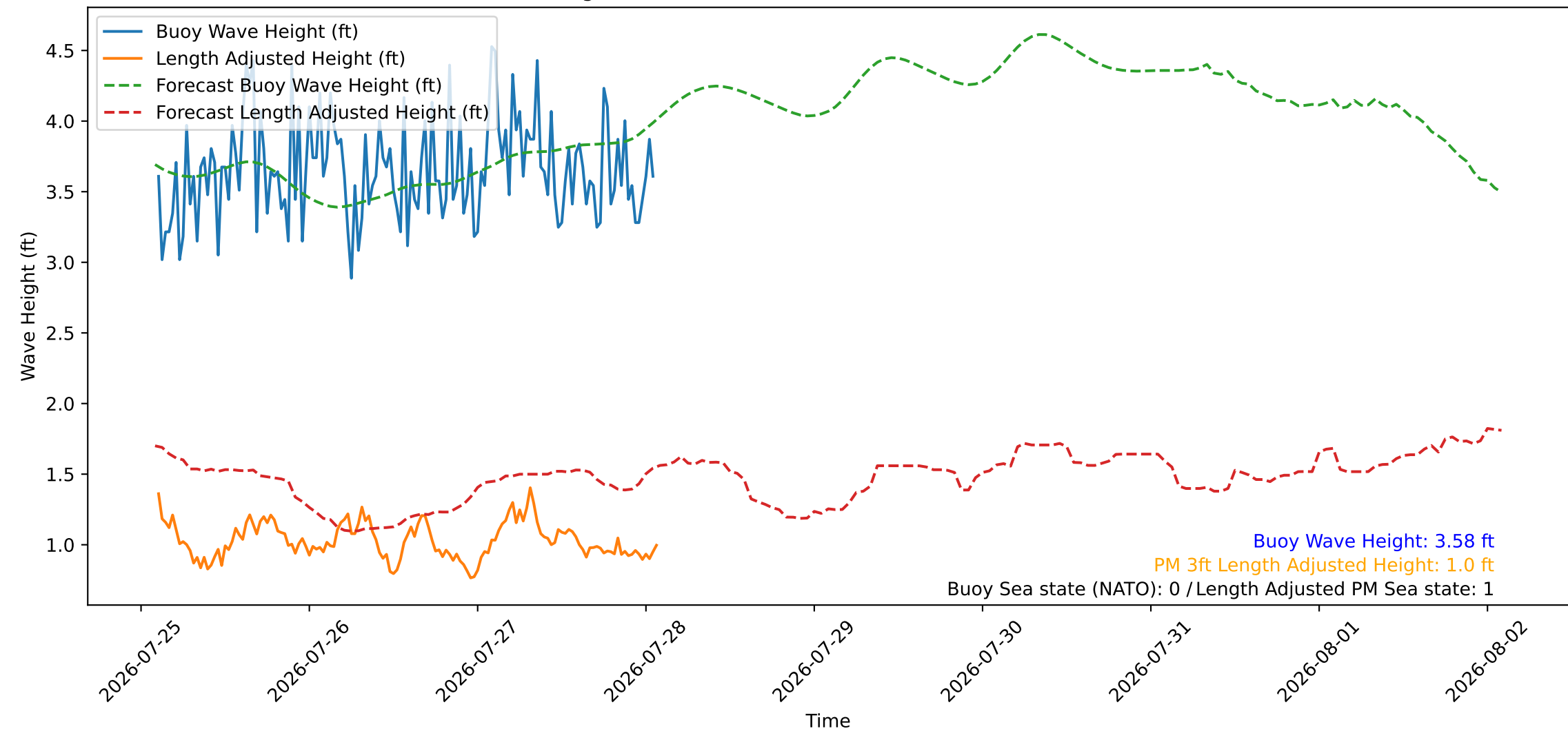
Wave Heights over Time for Red Beach at 2026-07-28 02:10:45
