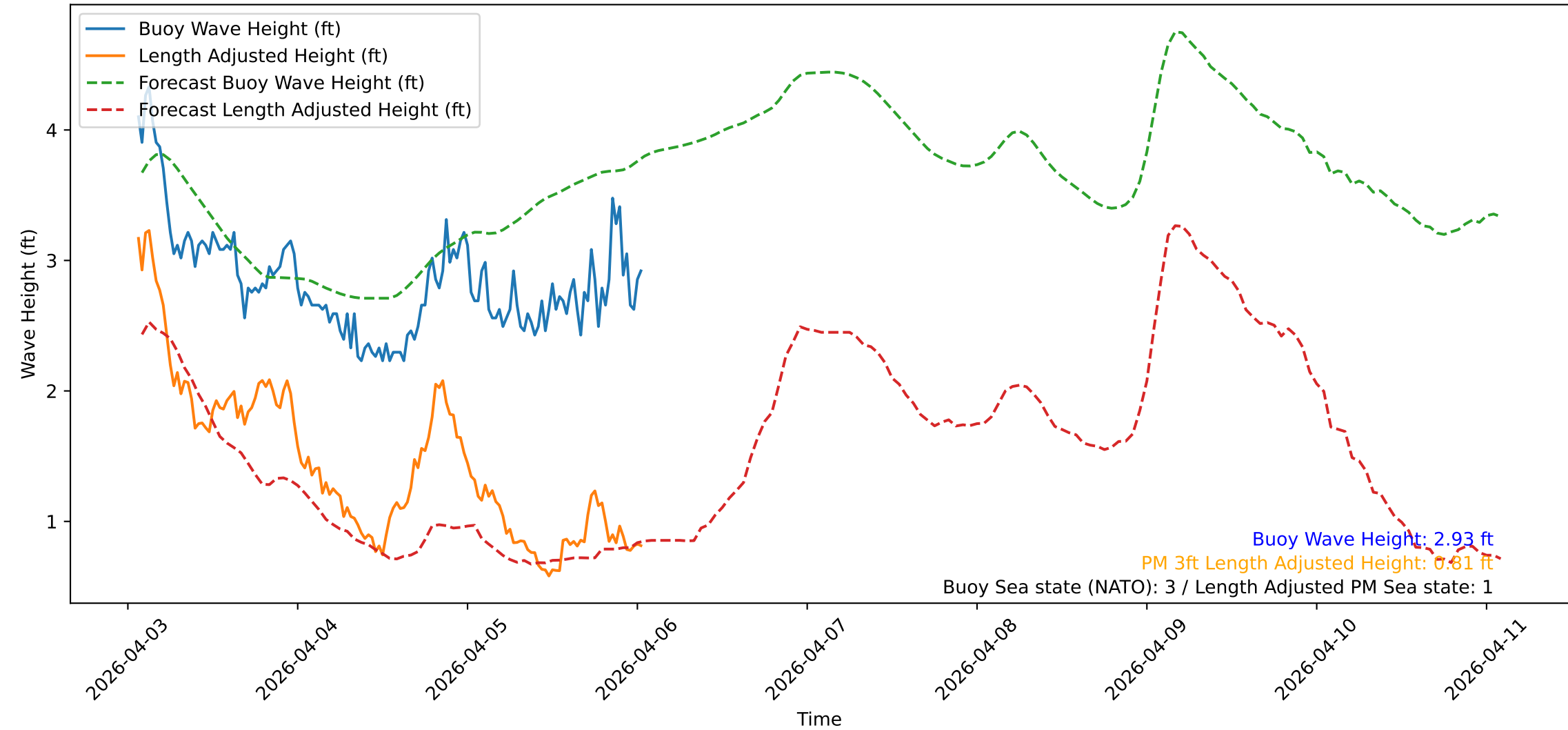
Wave Heights over Time for Green Beach at 2026-04-06 01:31:09
