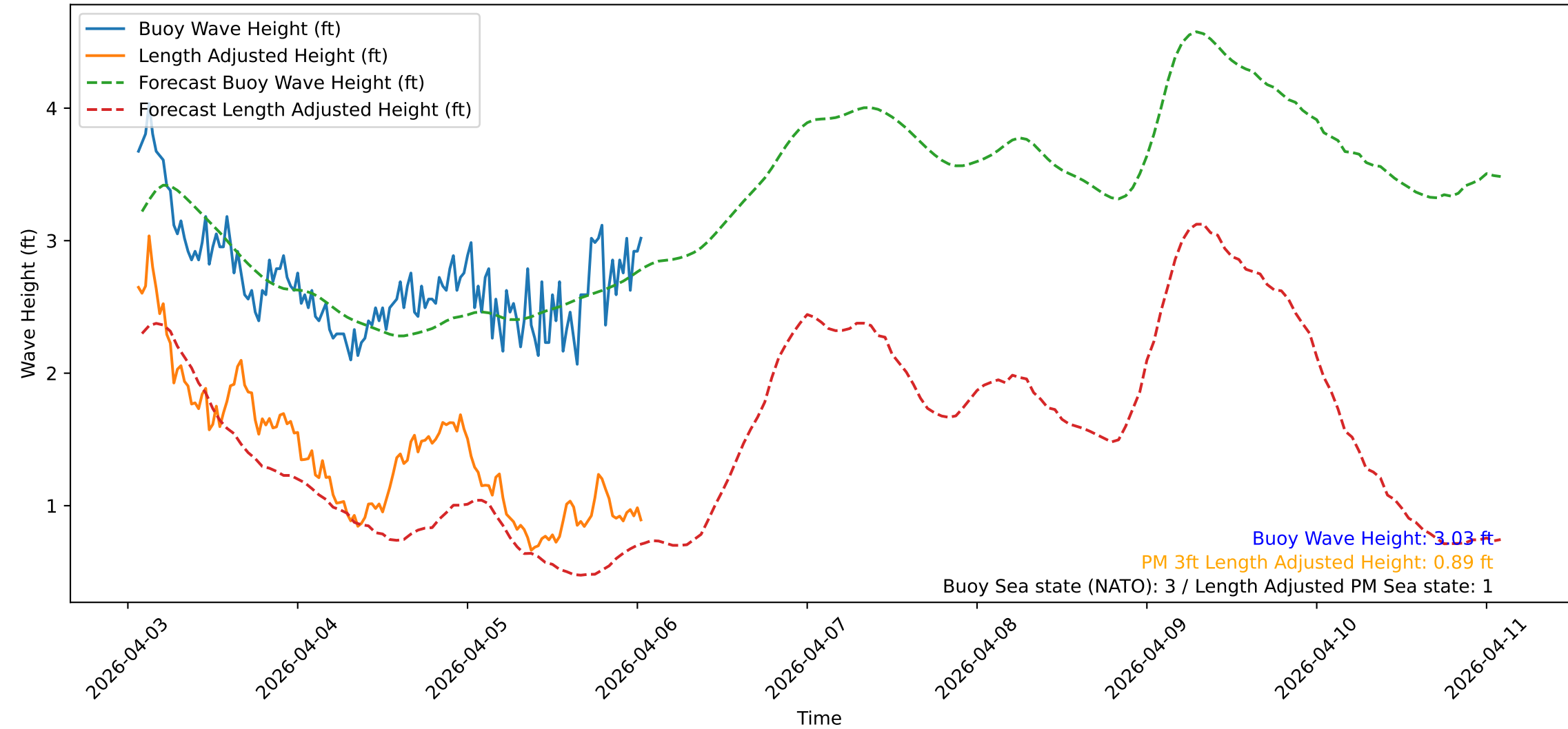
Wave Heights over Time for Oceanside Harbor at 2026-04-06 01:30:31
