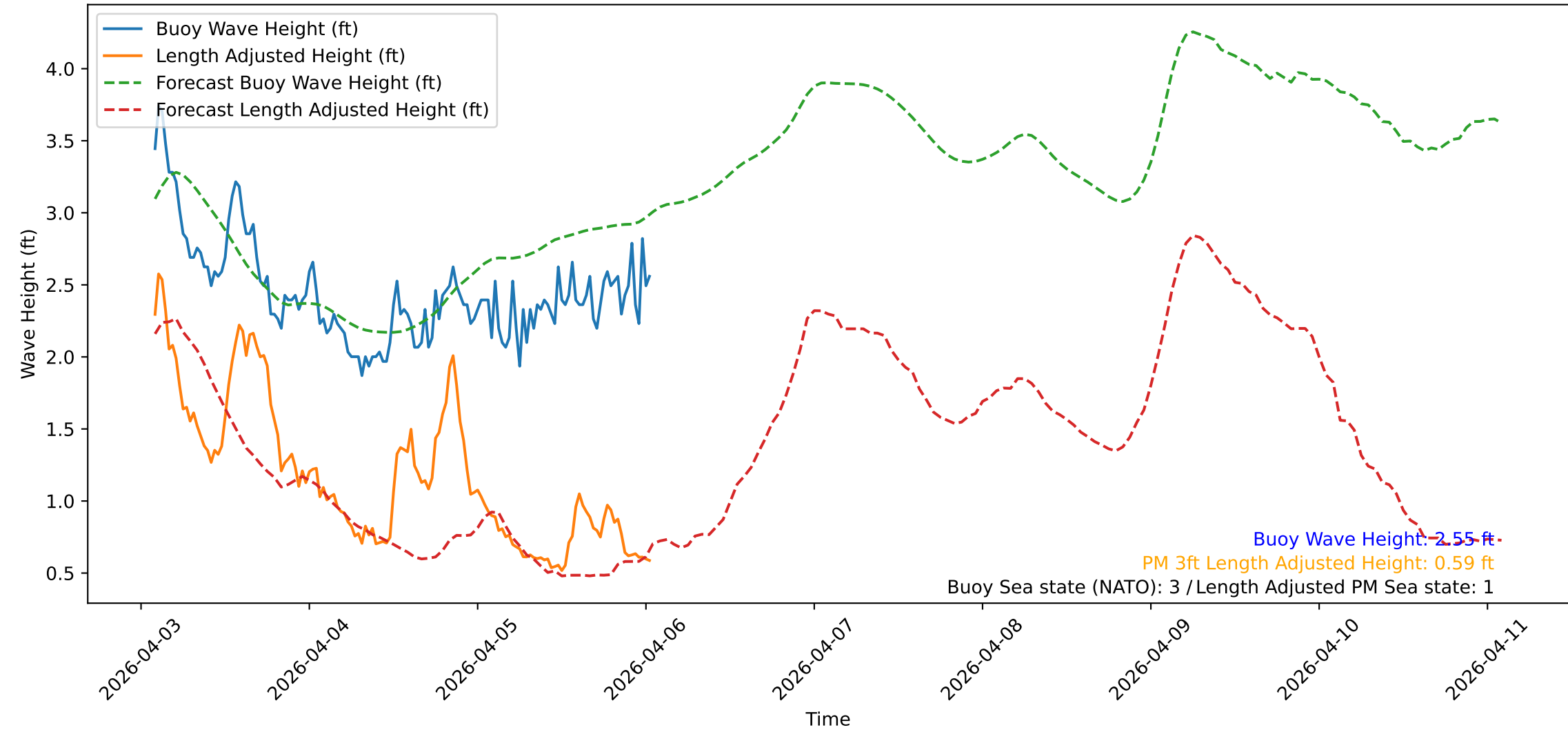
Wave Heights over Time for Red Beach at 2026-04-06 01:30:47
