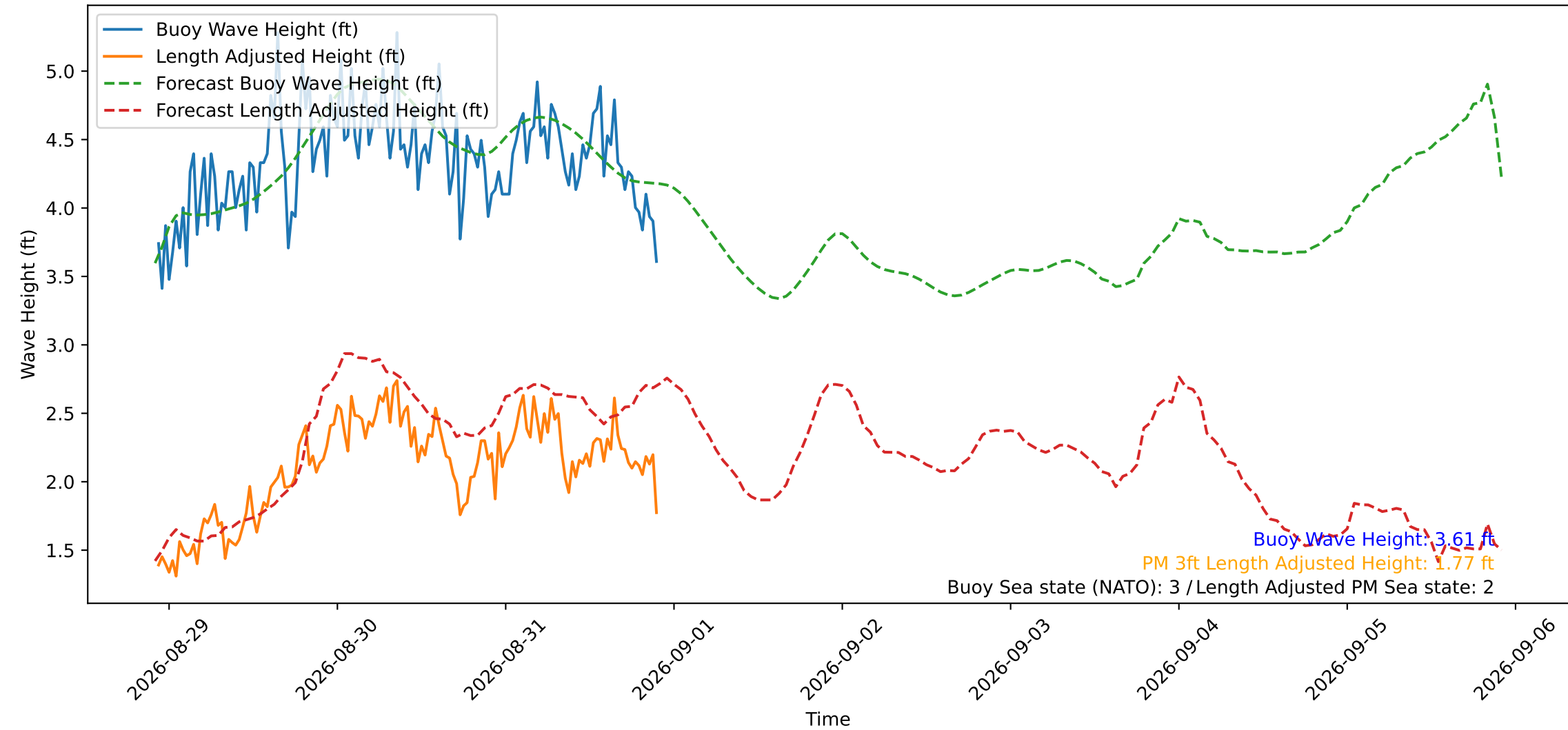
Wave Heights over Time for Oceanside Harbor at 2026-08-31 22:20:30
