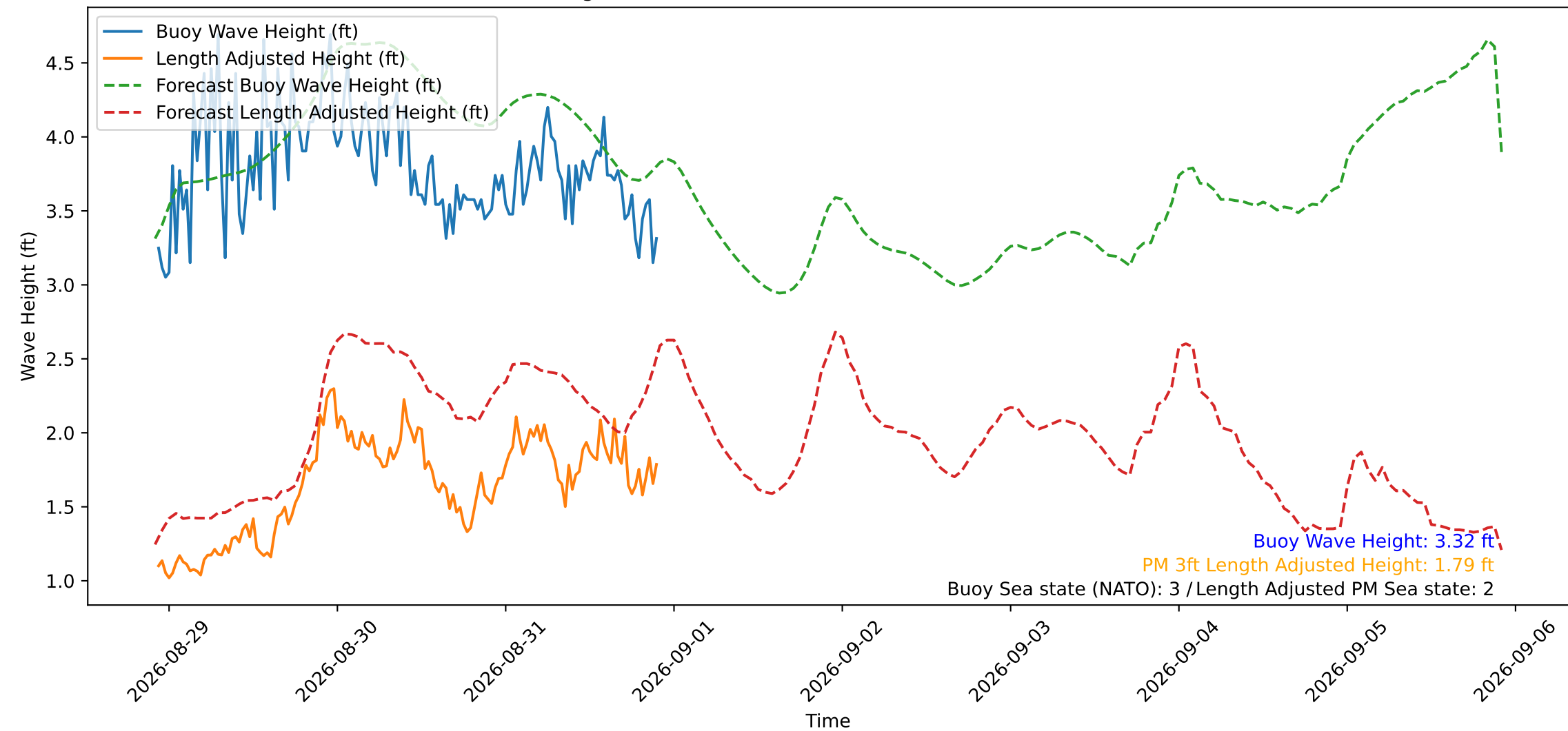
Wave Heights over Time for Red Beach at 2026-08-31 22:20:51
