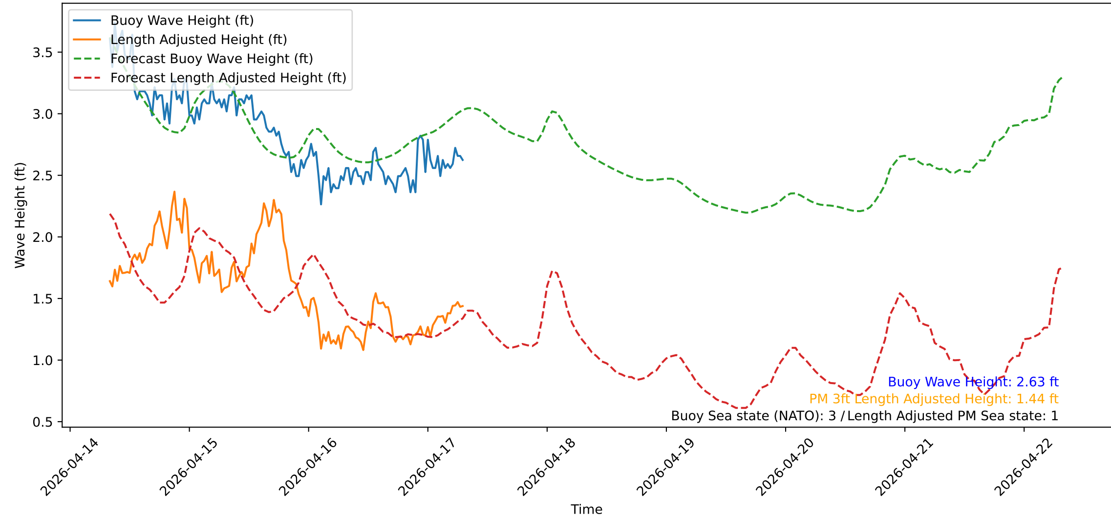
Wave Heights over Time for Red Beach at 2026-04-17 07:50:52
