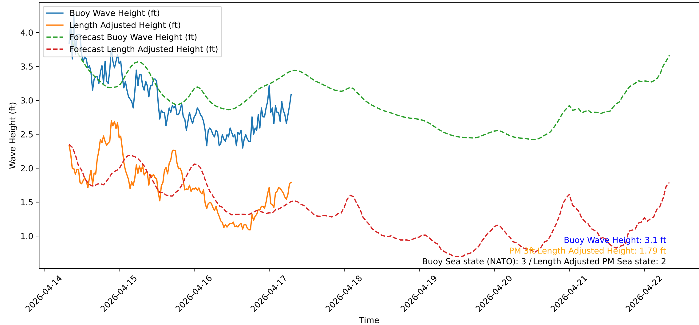
Wave Heights over Time for Oceanside Harbor at 2026-04-17 07:50:31
