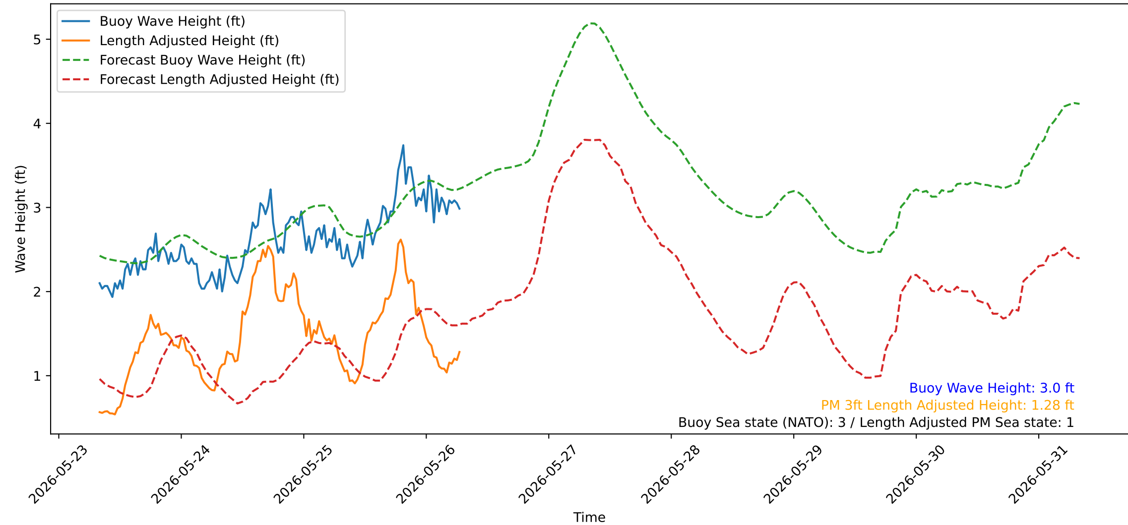
Wave Heights over Time for Red Beach at 2026-05-26 07:40:48
