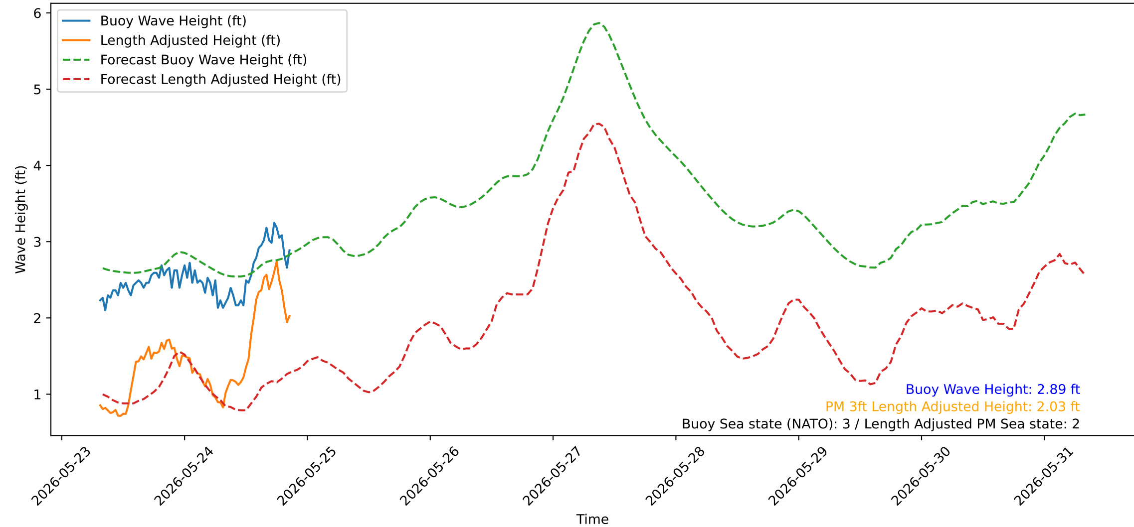
Wave Heights over Time for Oceanside Harbor at 2026-05-26 07:40:28
