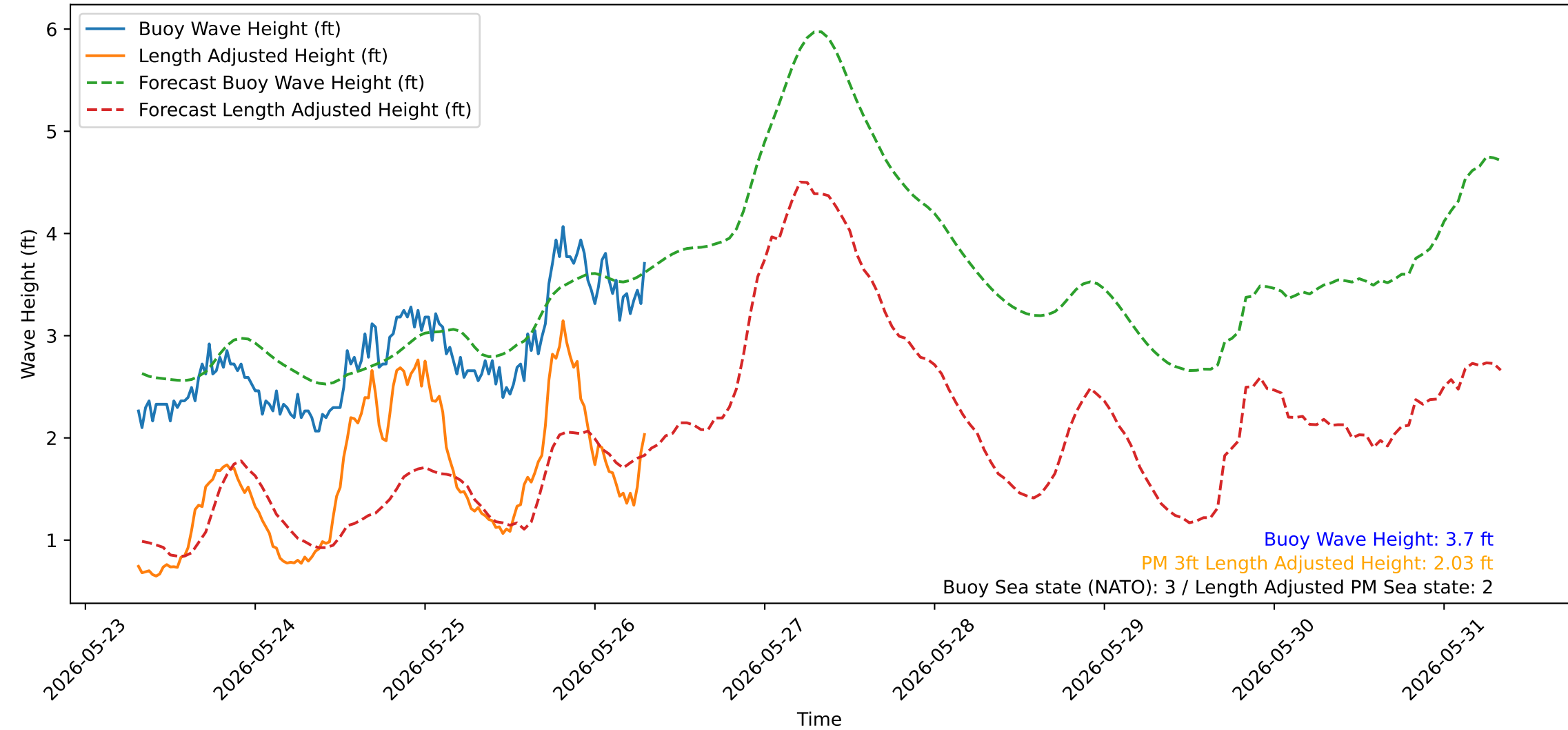
Wave Heights over Time for Green Beach at 2026-05-26 07:41:11
