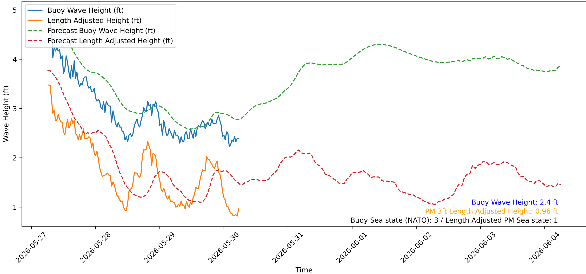
Wave Heights over Time for Red Beach at 2026-05-30 06:10:42
