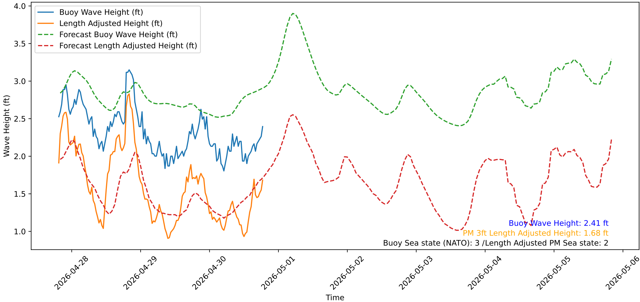
Wave Heights over Time for Green Beach at 2026-04-30 19:31:13
