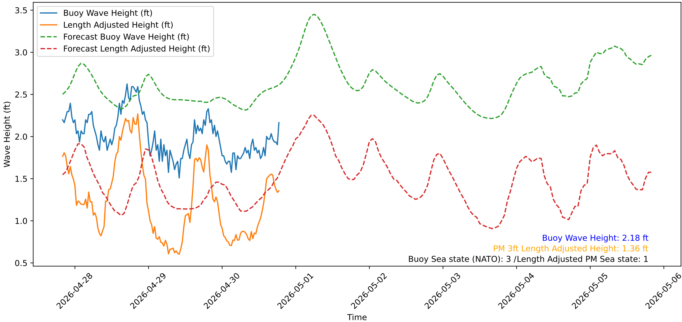
Wave Heights over Time for Red Beach at 2026-04-30 19:30:50
