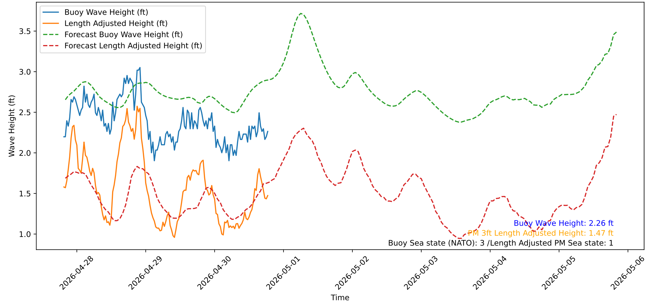
Wave Heights over Time for Oceanside Harbor at 2026-04-30 19:30:31
