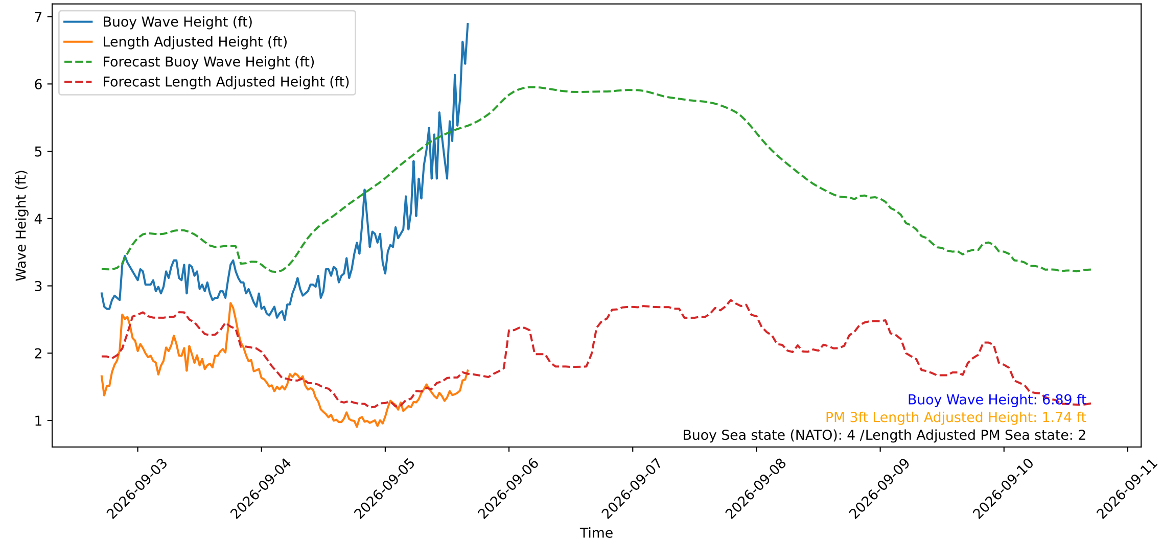
Wave Heights over Time for Green Beach at 2026-09-05 16:41:12
