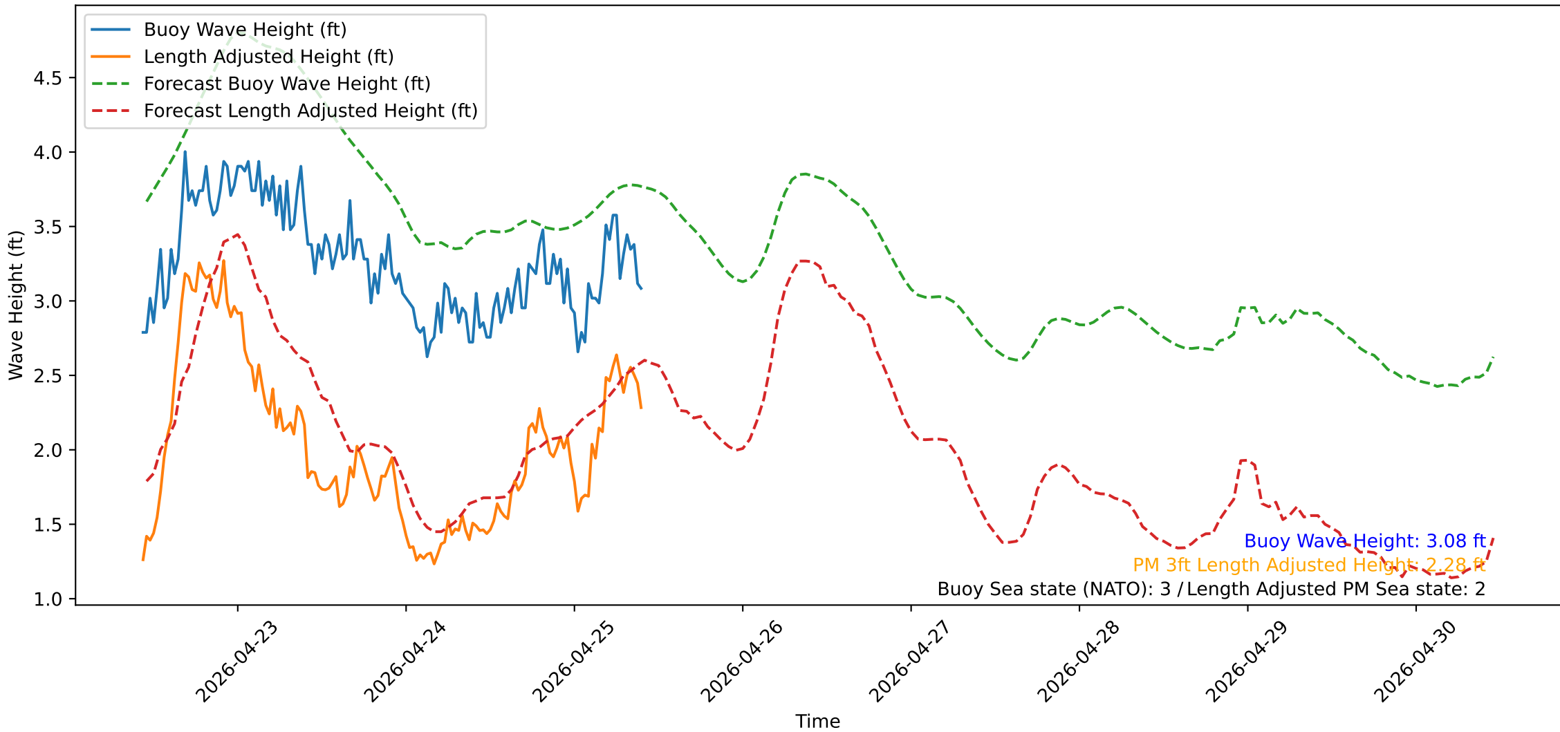
Wave Heights over Time for Green Beach at 2026-04-25 10:31:12
