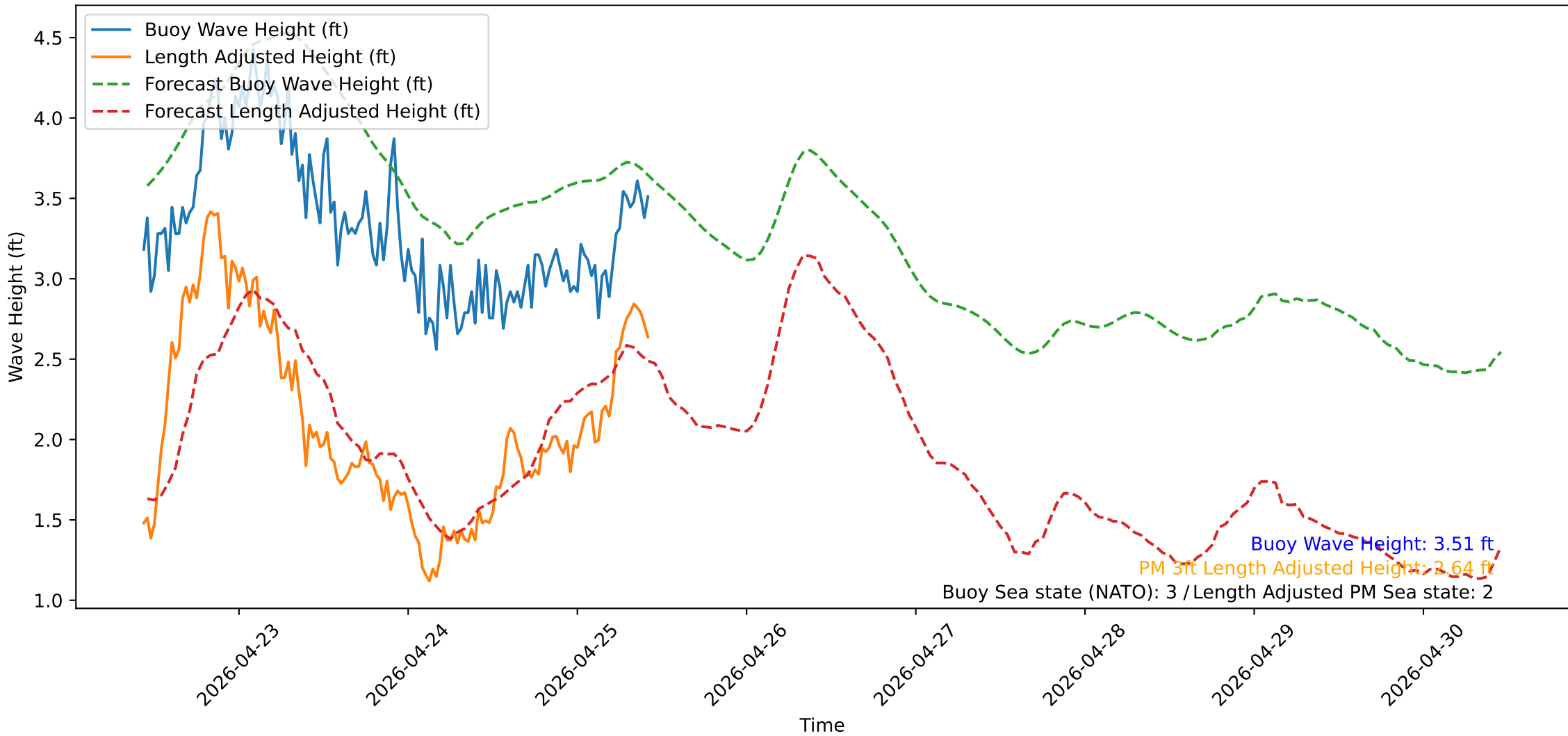
Wave Heights over Time for Oceanside Harbor at 2026-04-25 10:30:32
