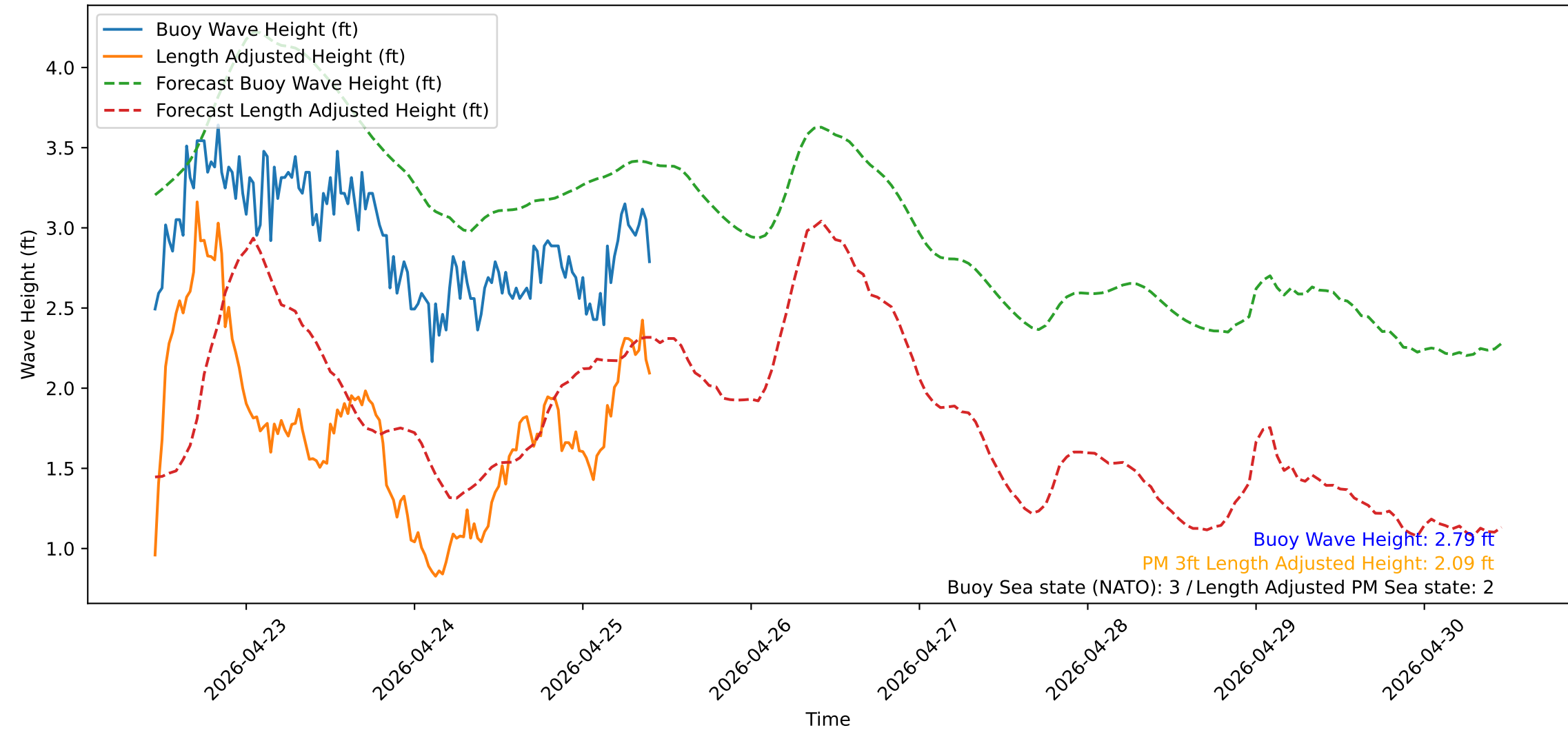
Wave Heights over Time for Red Beach at 2026-04-25 10:30:51
