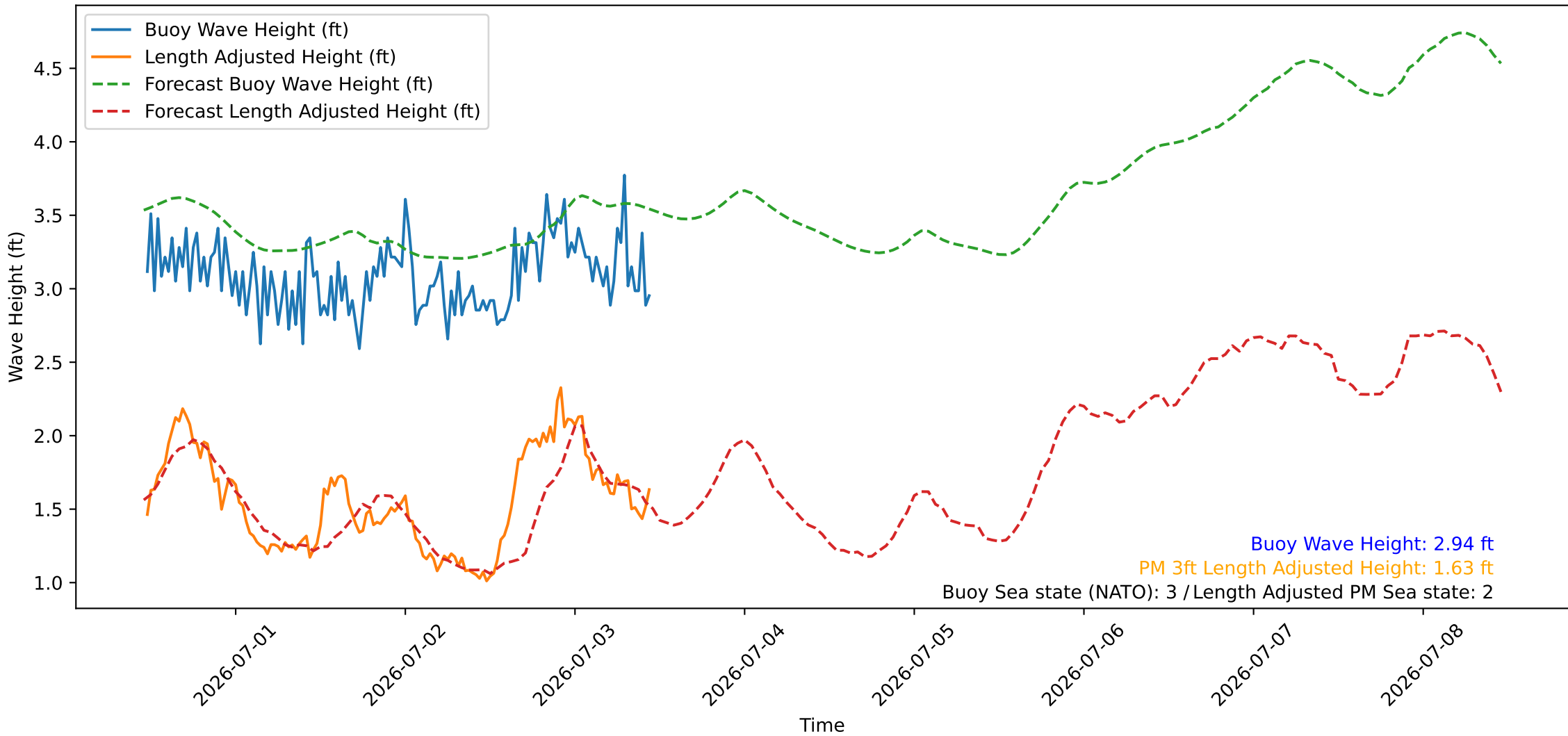
Wave Heights over Time for Oceanside Harbor at 2026-07-03 11:20:26
