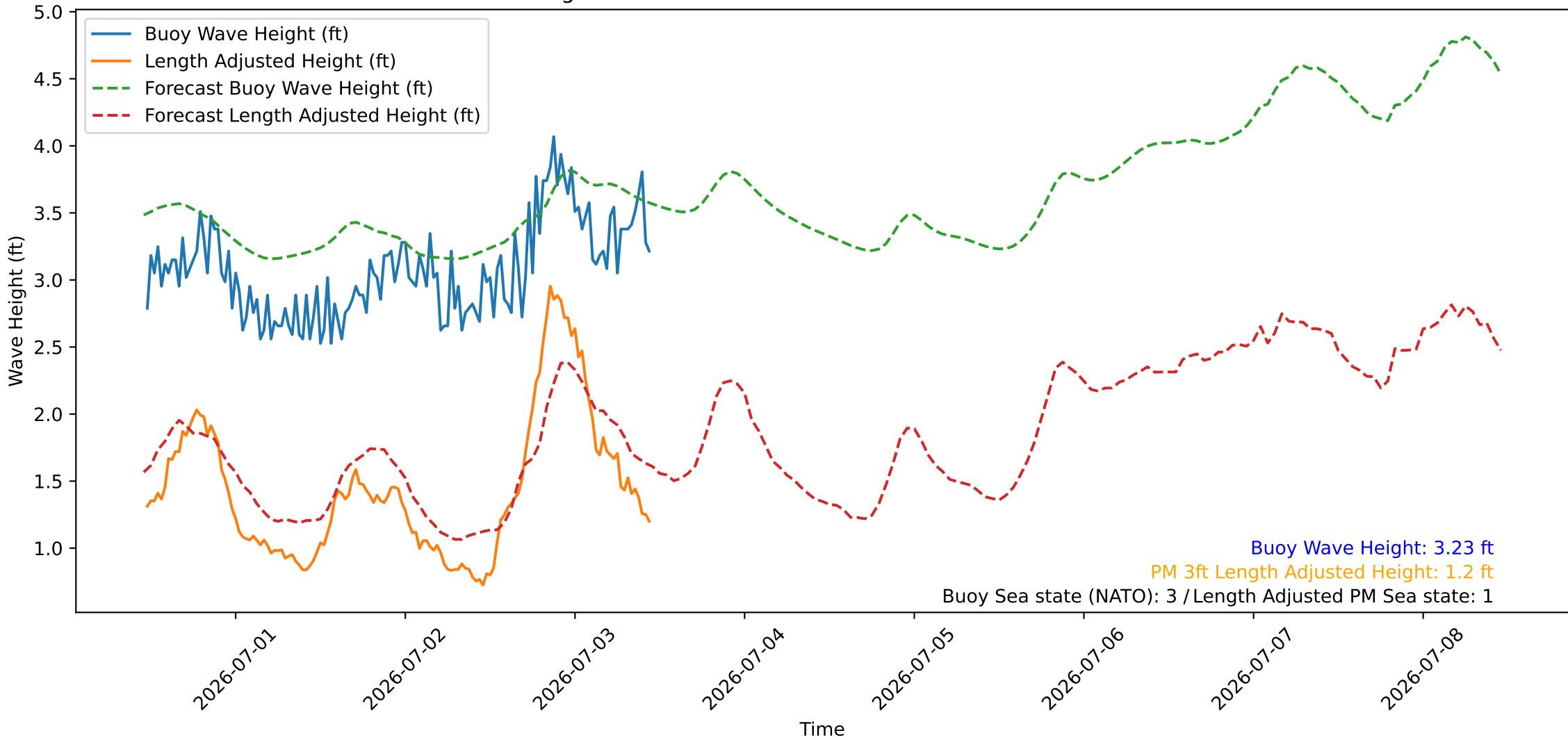
Wave Heights over Time for Green Beach at 2026-07-03 11:21:09
