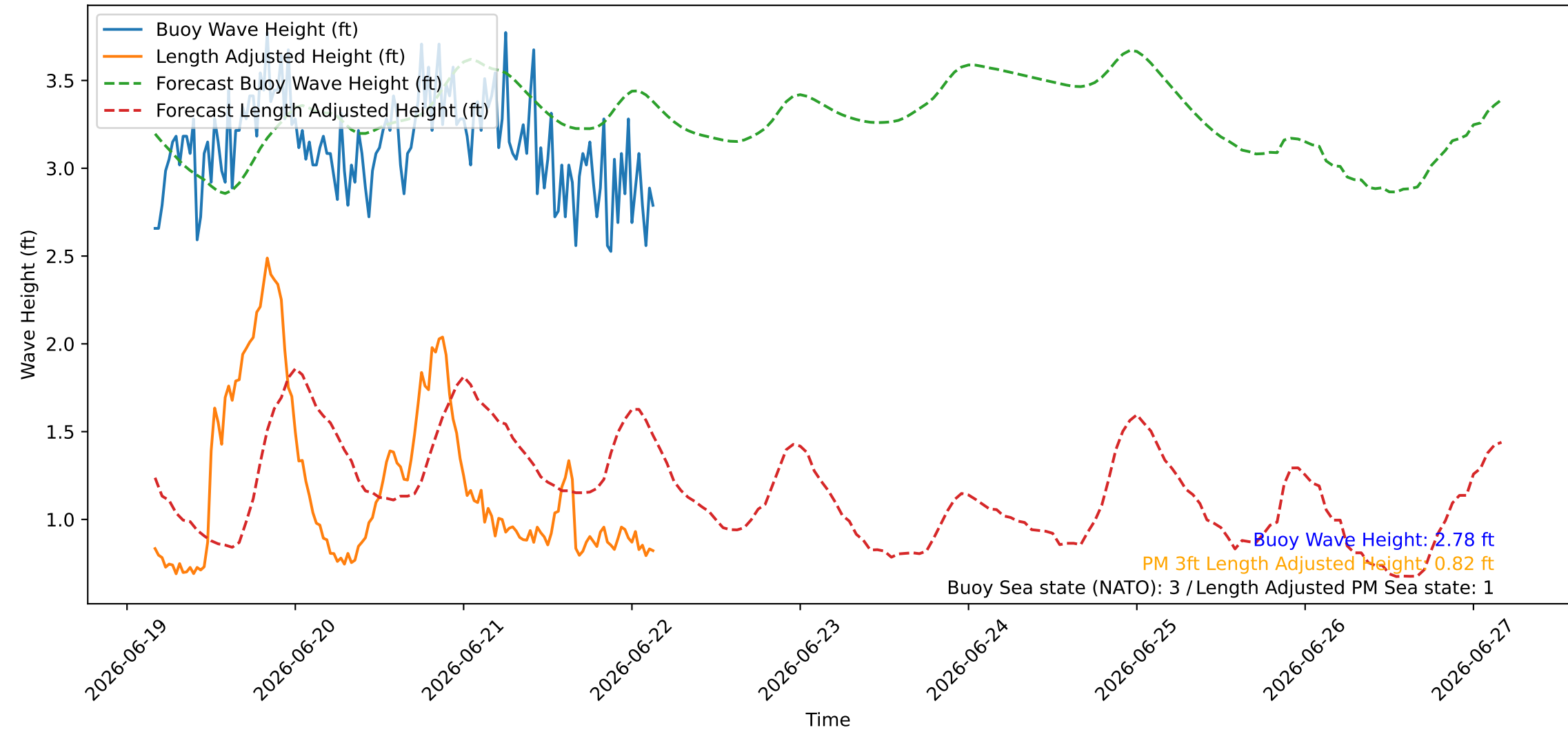
Wave Heights over Time for Red Beach at 2026-06-22 03:50:46
