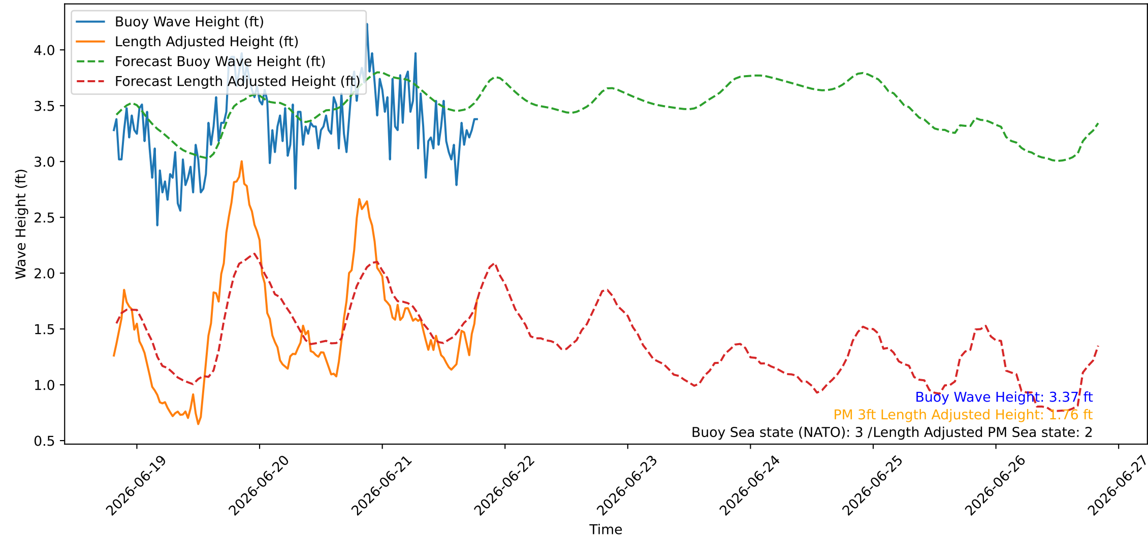
Wave Heights over Time for Green Beach at 2026-06-21 19:41:07
