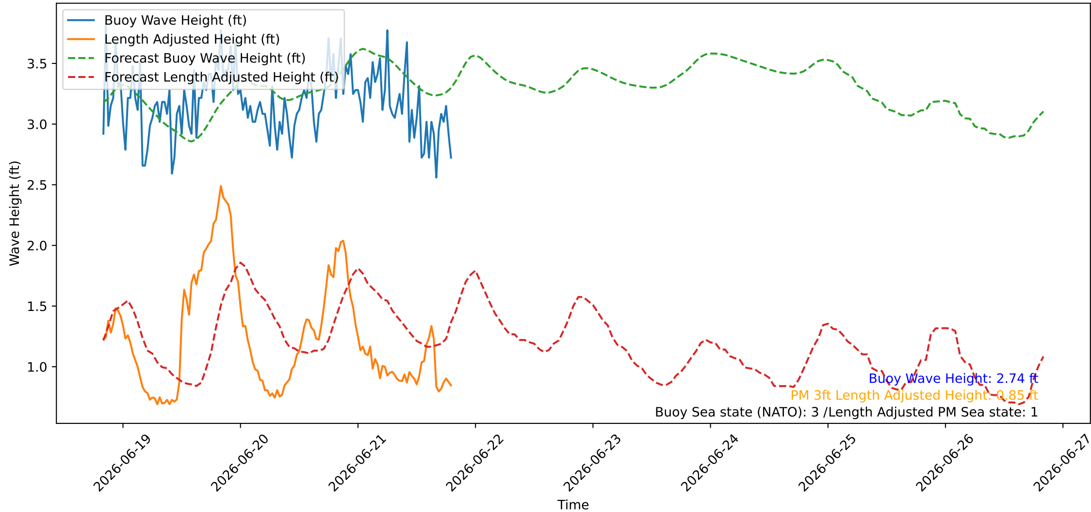
Wave Heights over Time for Red Beach at 2026-06-21 19:40:45
