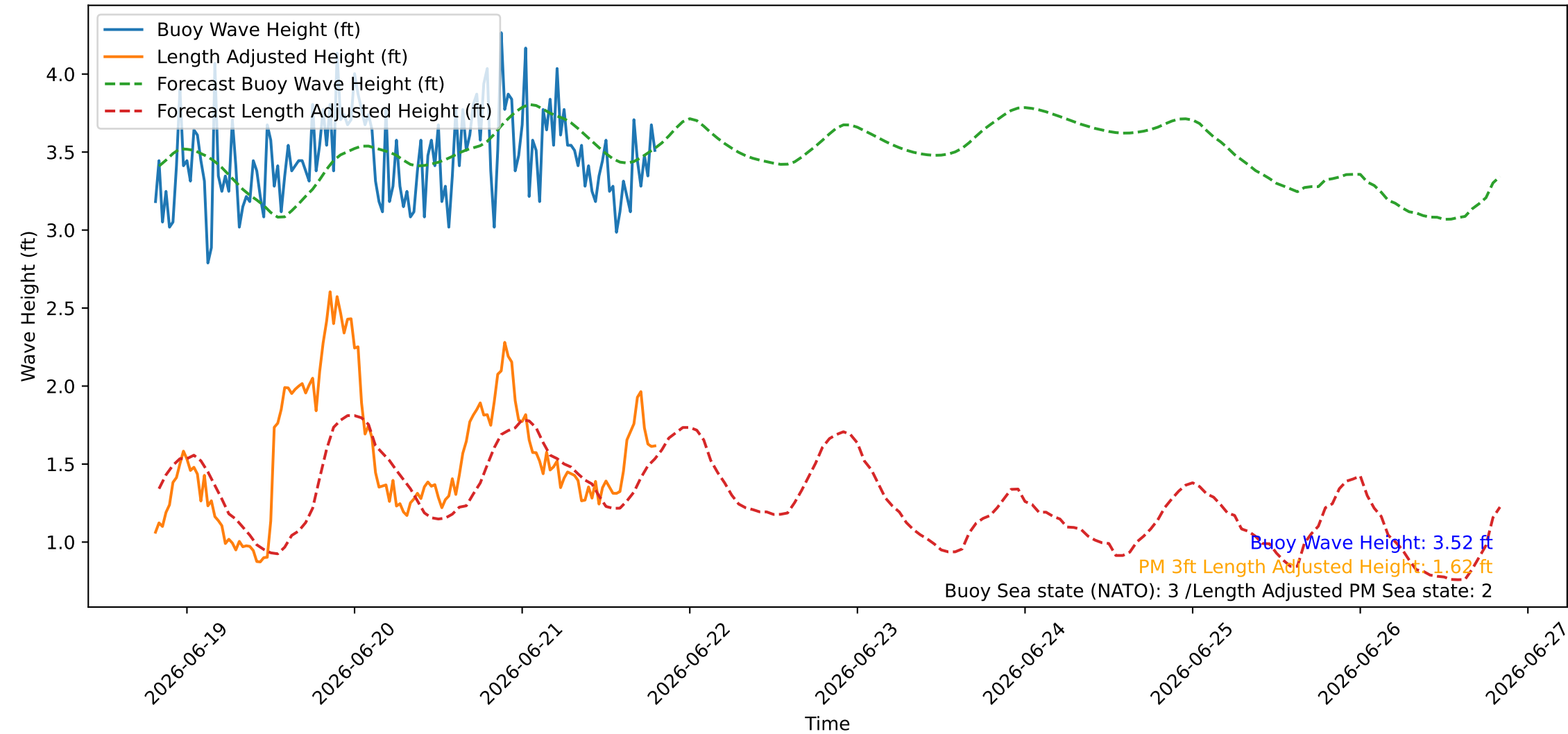
Wave Heights over Time for Oceanside Harbor at 2026-06-21 19:40:25
