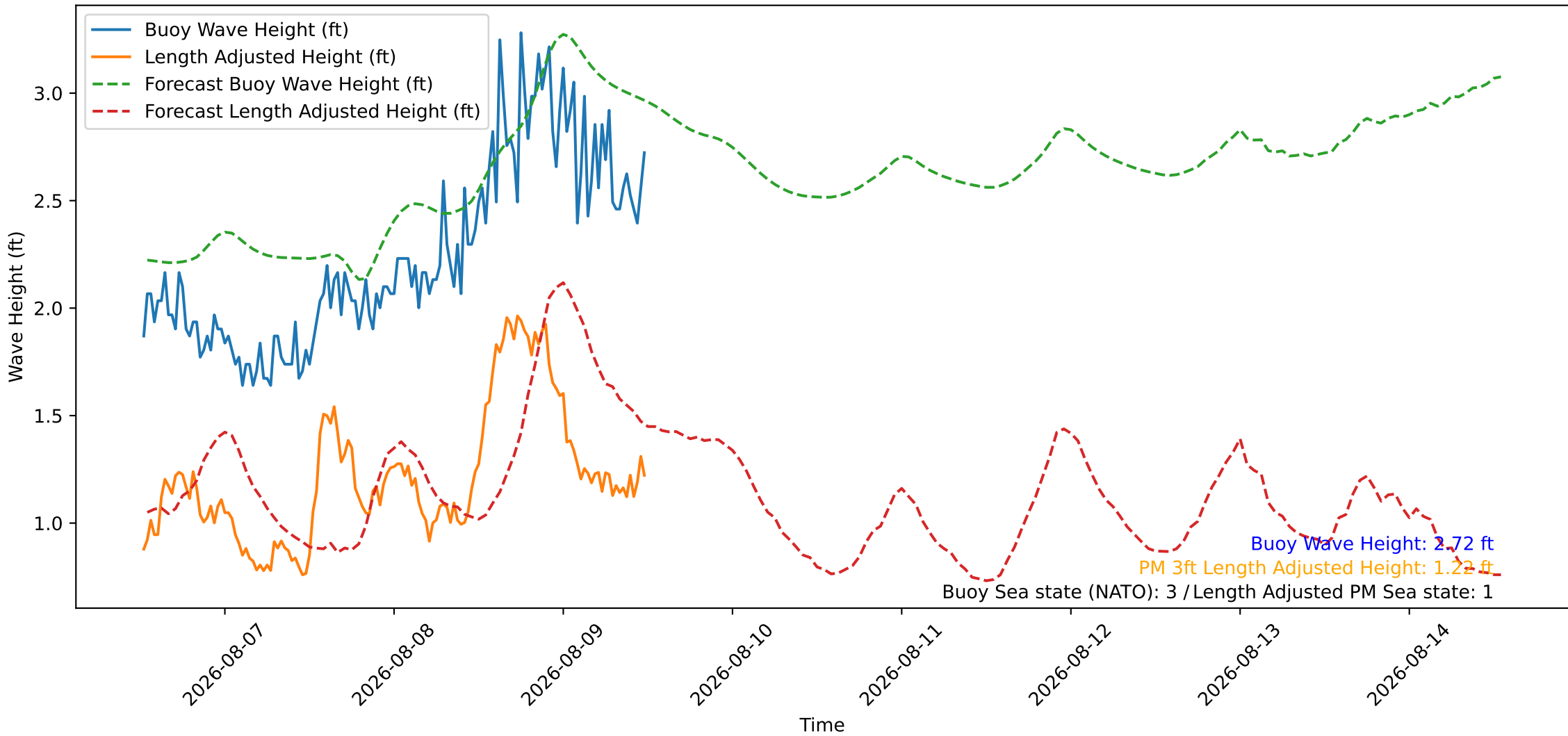
Wave Heights over Time for Oceanside Harbor at 2026-08-09 12:30:27
