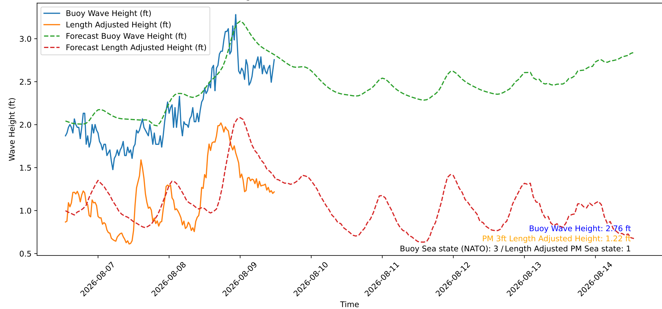
Wave Heights over Time for Red Beach at 2026-08-09 12:30:46
