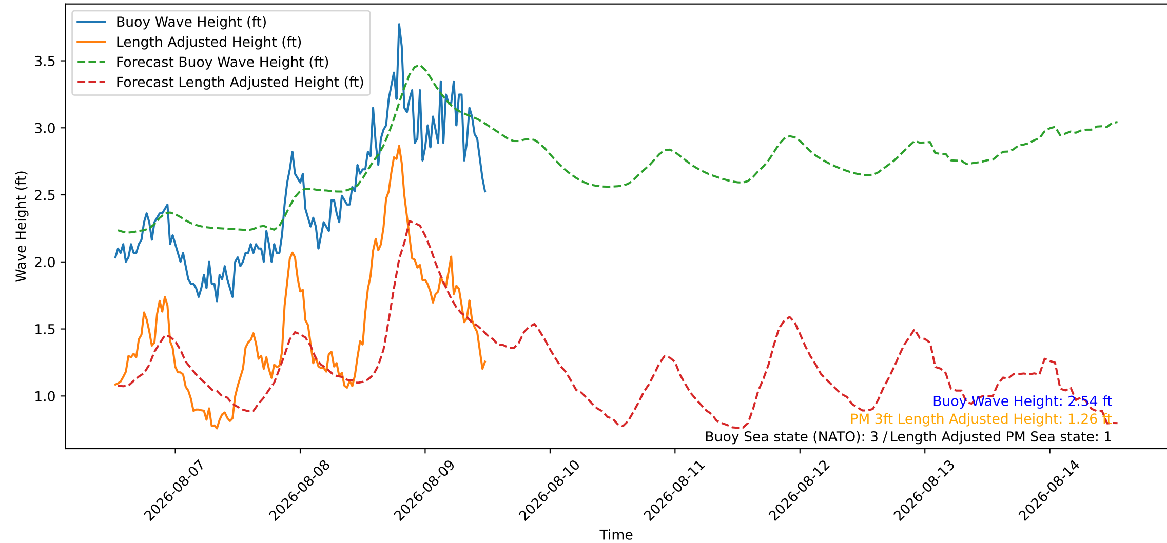
Wave Heights over Time for Green Beach at 2026-08-09 12:31:09
