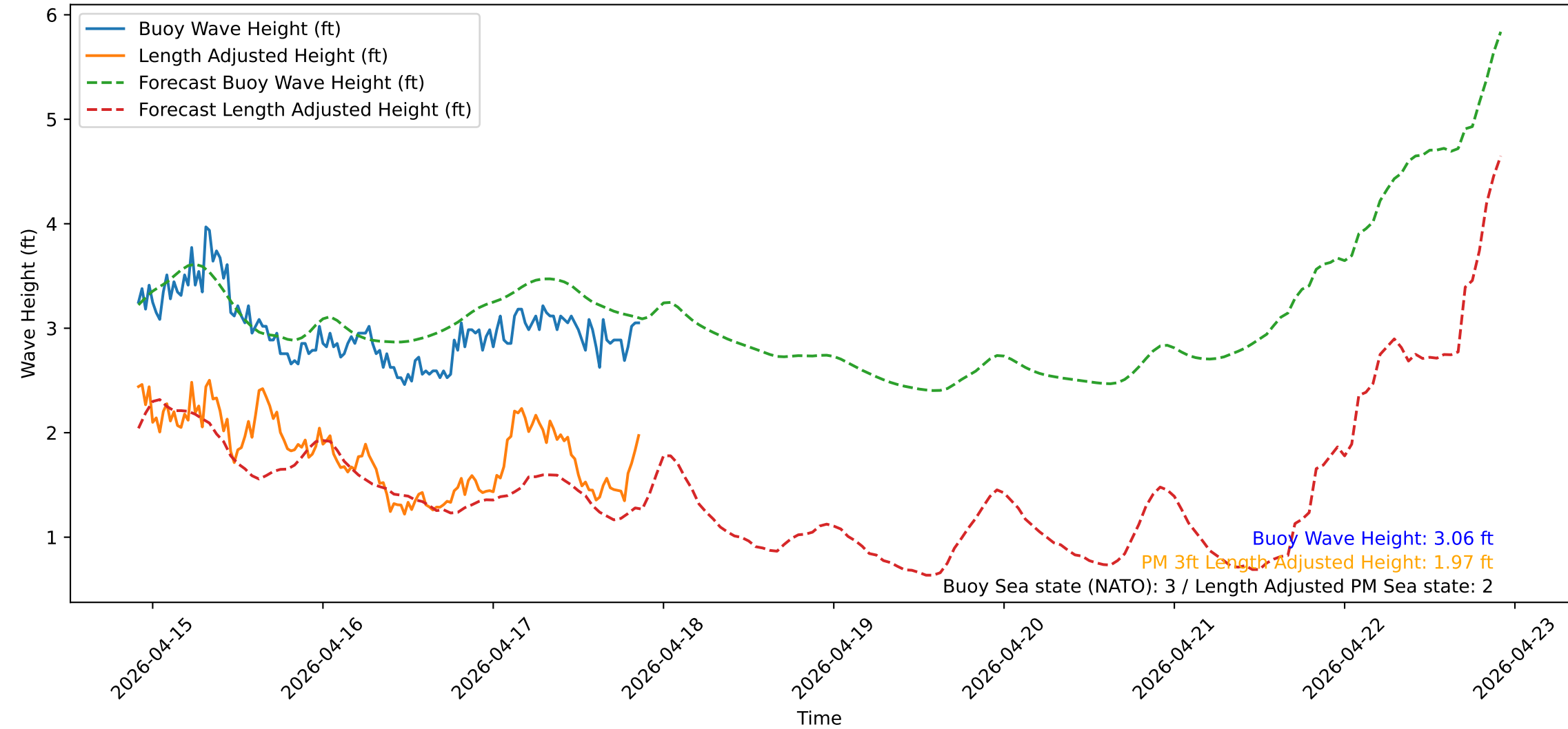
Wave Heights over Time for Green Beach at 2026-04-17 21:51:20
