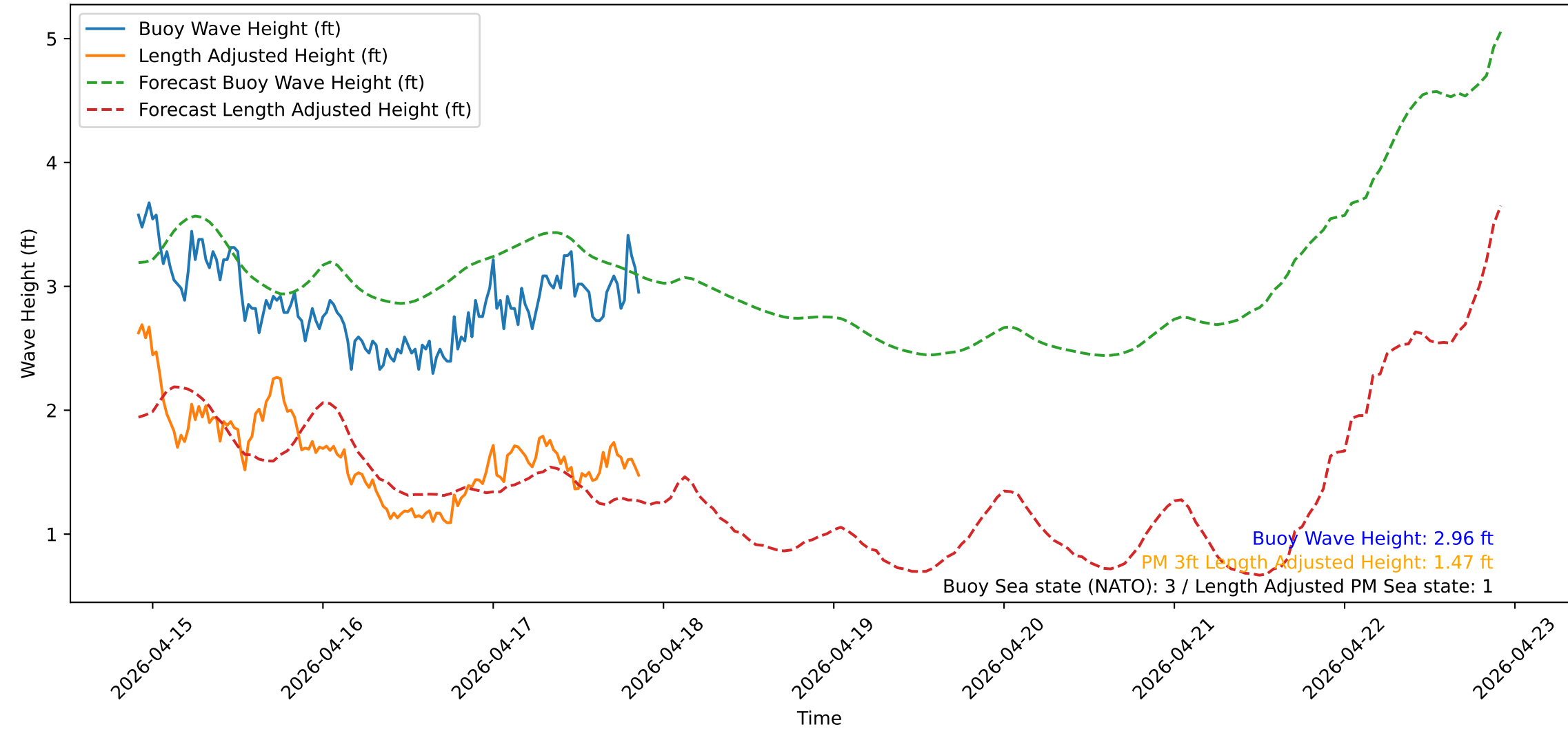
Wave Heights over Time for Oceanside Harbor at 2026-04-17 21:50:36
