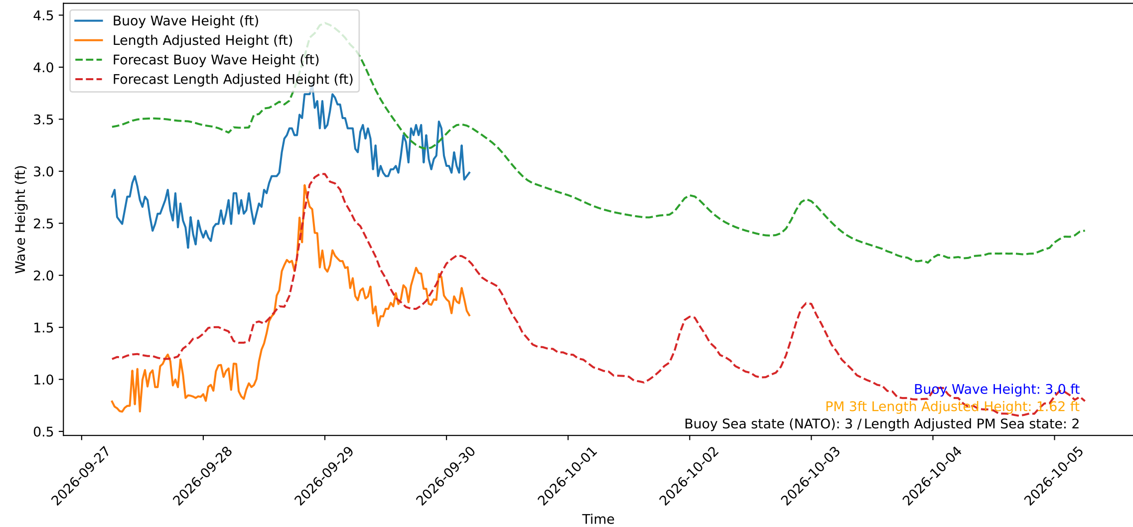
Wave Heights over Time for Red Beach at 2026-09-30 05:30:53
