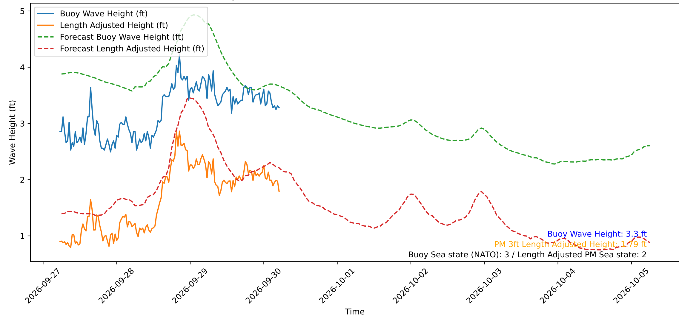
Wave Heights over Time for Oceanside Harbor at 2026-09-30 05:30:33
