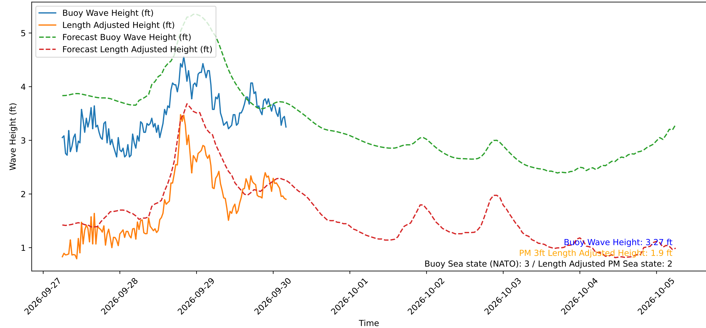
Wave Heights over Time for Green Beach at 2026-09-30 05:31:15
