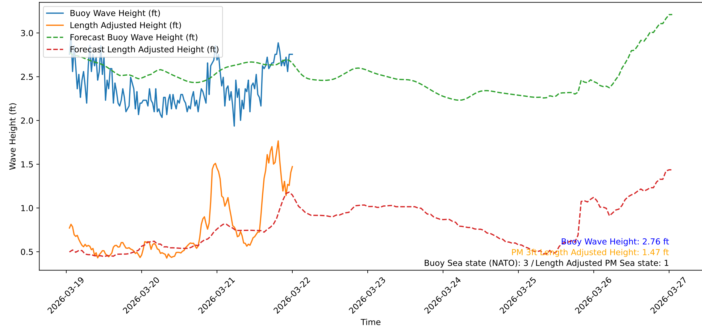
Wave Heights over Time for Green Beach at 2026-03-22 01:01:09
