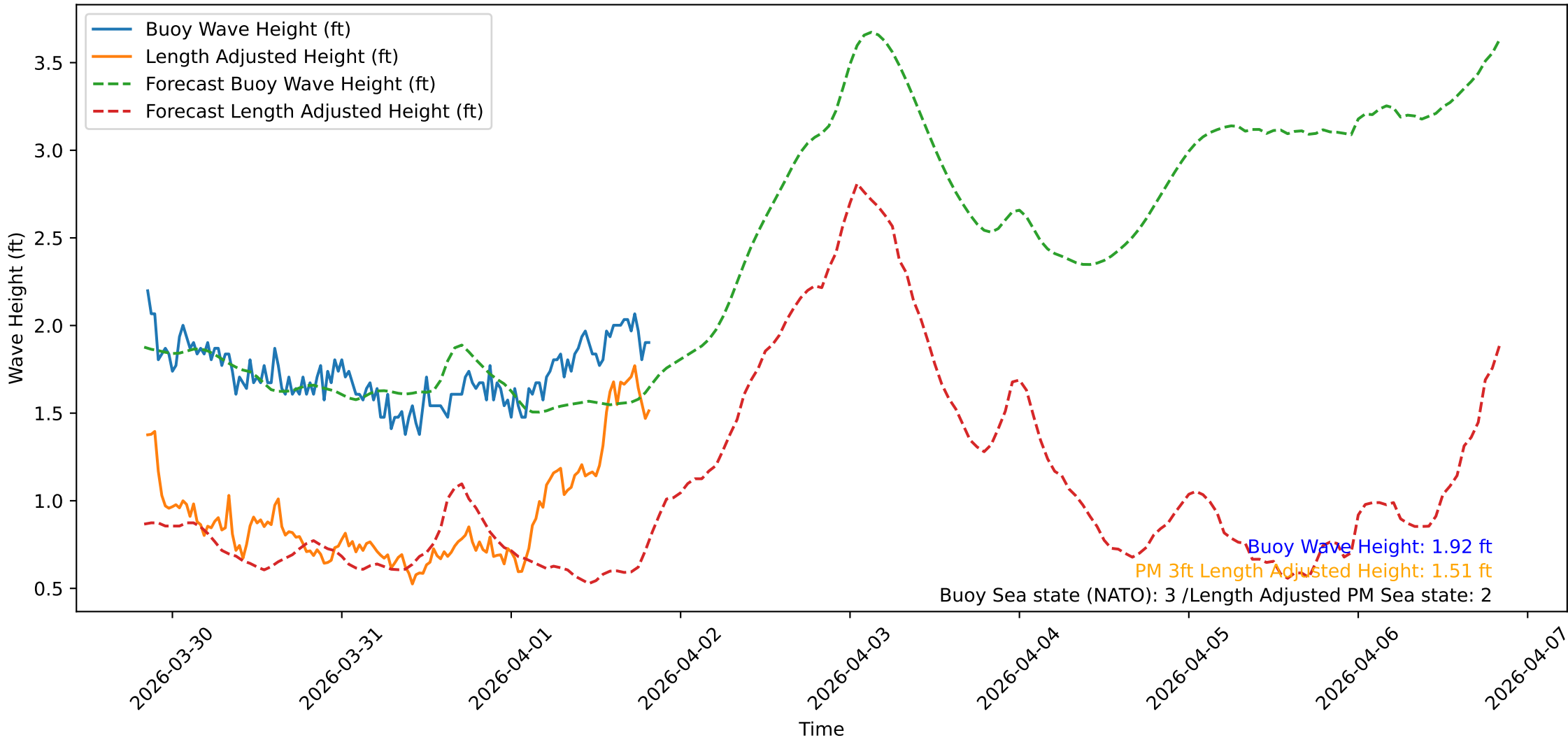
Wave Heights over Time for Red Beach at 2026-04-01 20:10:47
