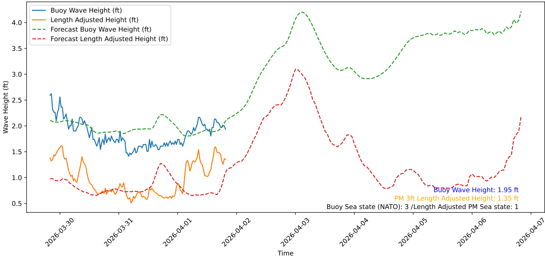
Wave Heights over Time for Green Beach at 2026-04-01 20:11:09
