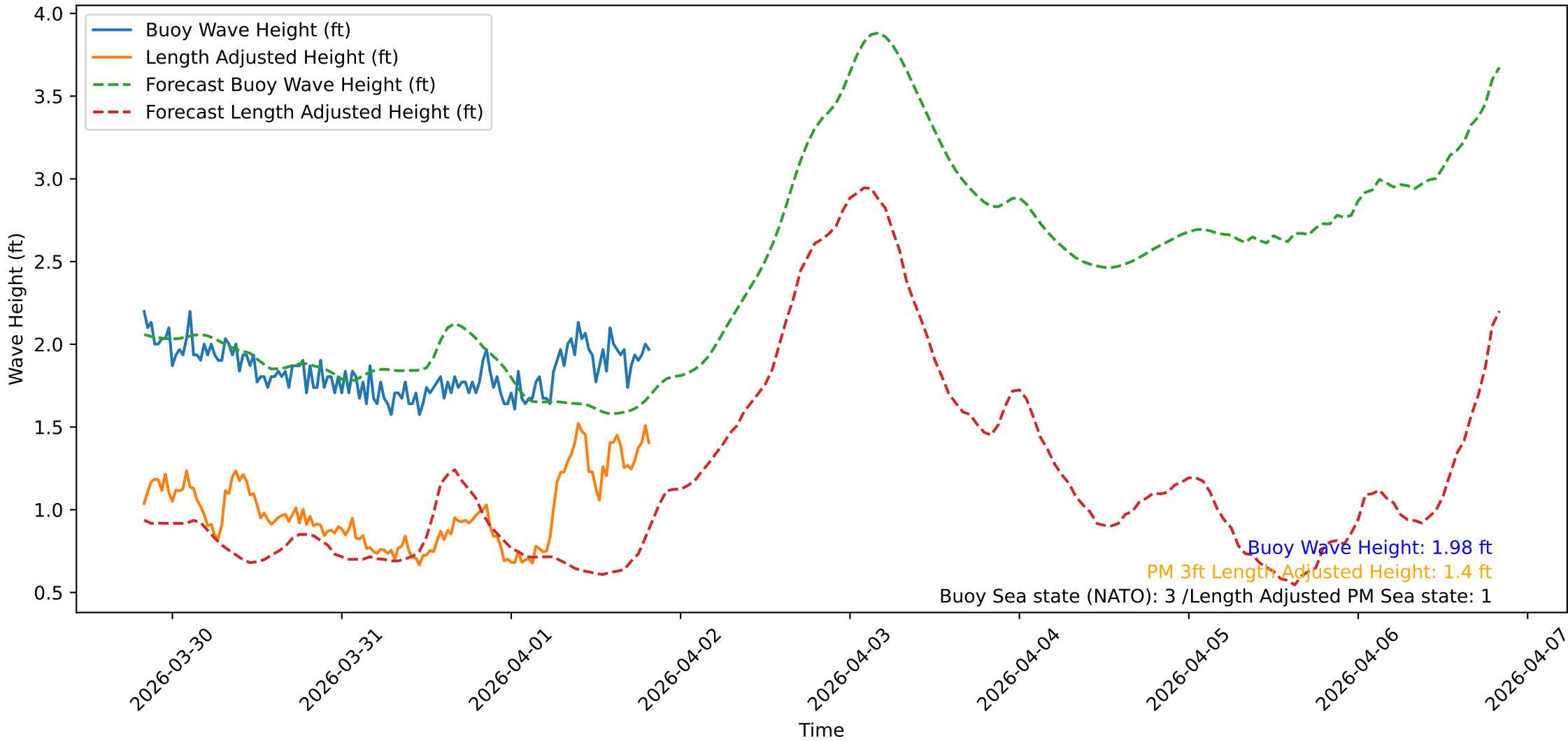
Wave Heights over Time for Oceanside Harbor at 2026-04-01 20:10:31
