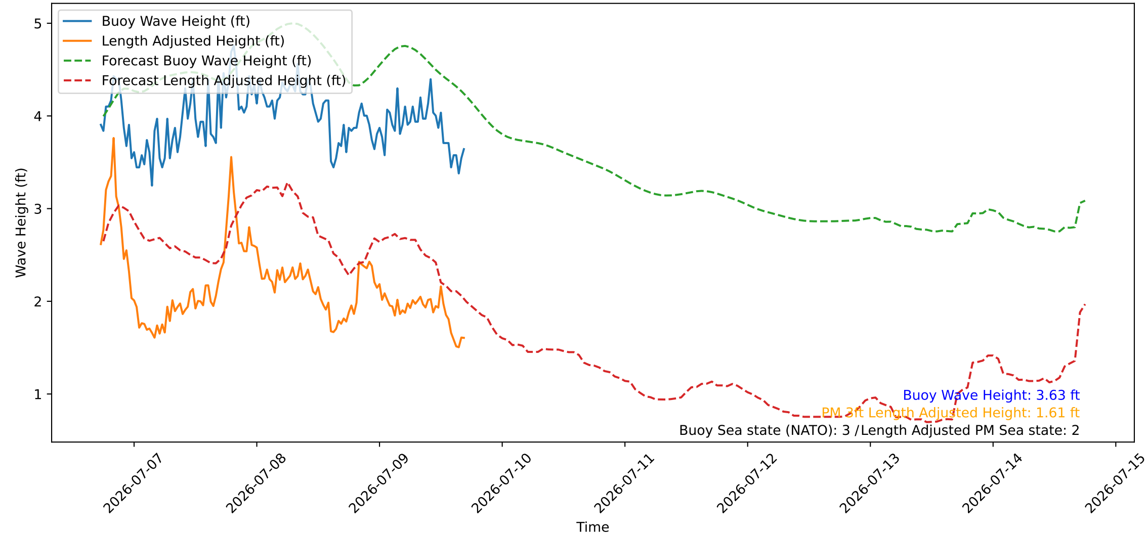
Wave Heights over Time for Green Beach at 2026-07-09 17:31:08
