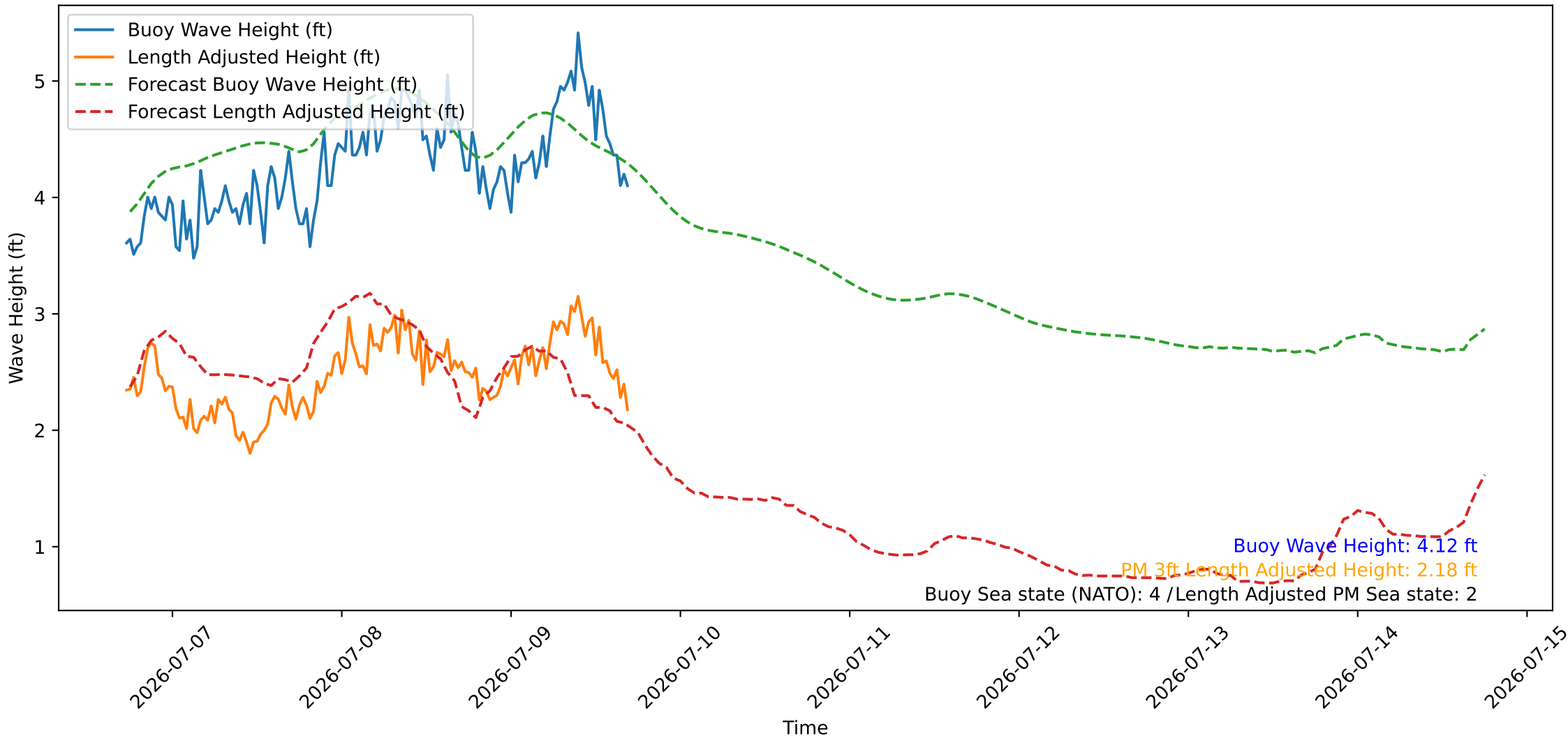
Wave Heights over Time for Oceanside Harbor at 2026-07-09 17:30:27
