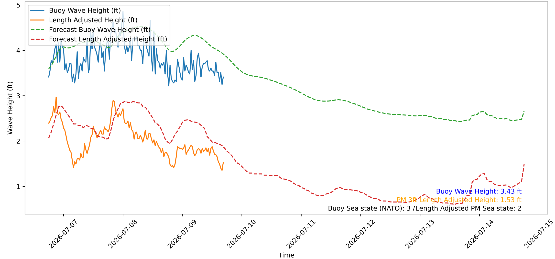
Wave Heights over Time for Red Beach at 2026-07-09 17:30:46
