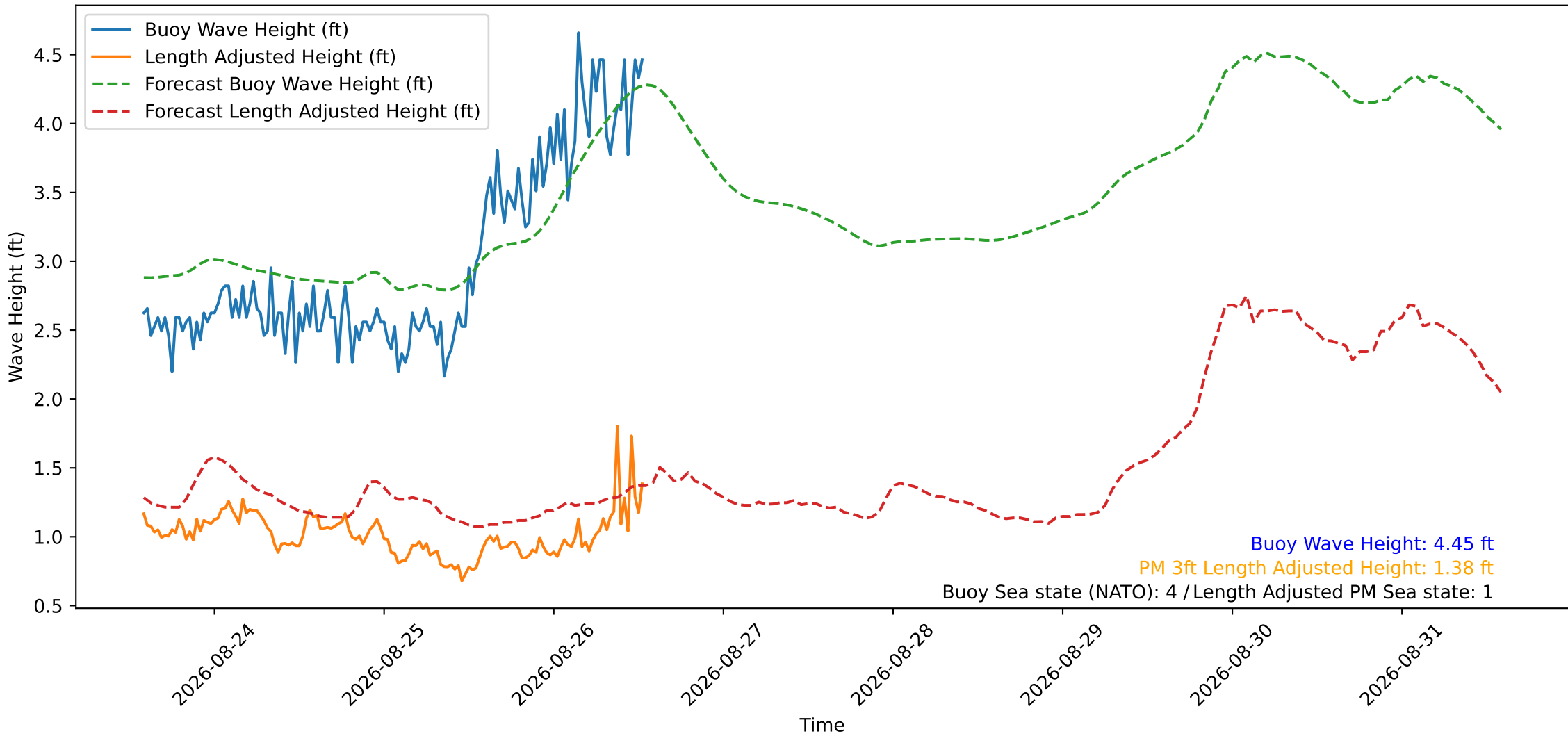
Wave Heights over Time for Red Beach at 2026-08-26 13:30:50
