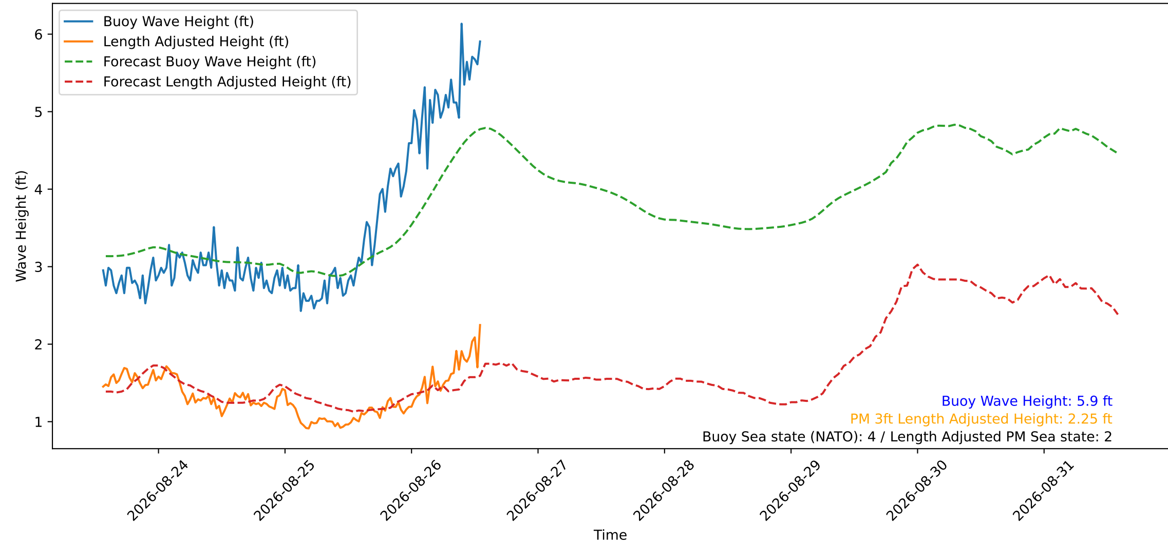
Wave Heights over Time for Oceanside Harbor at 2026-08-26 13:30:30
