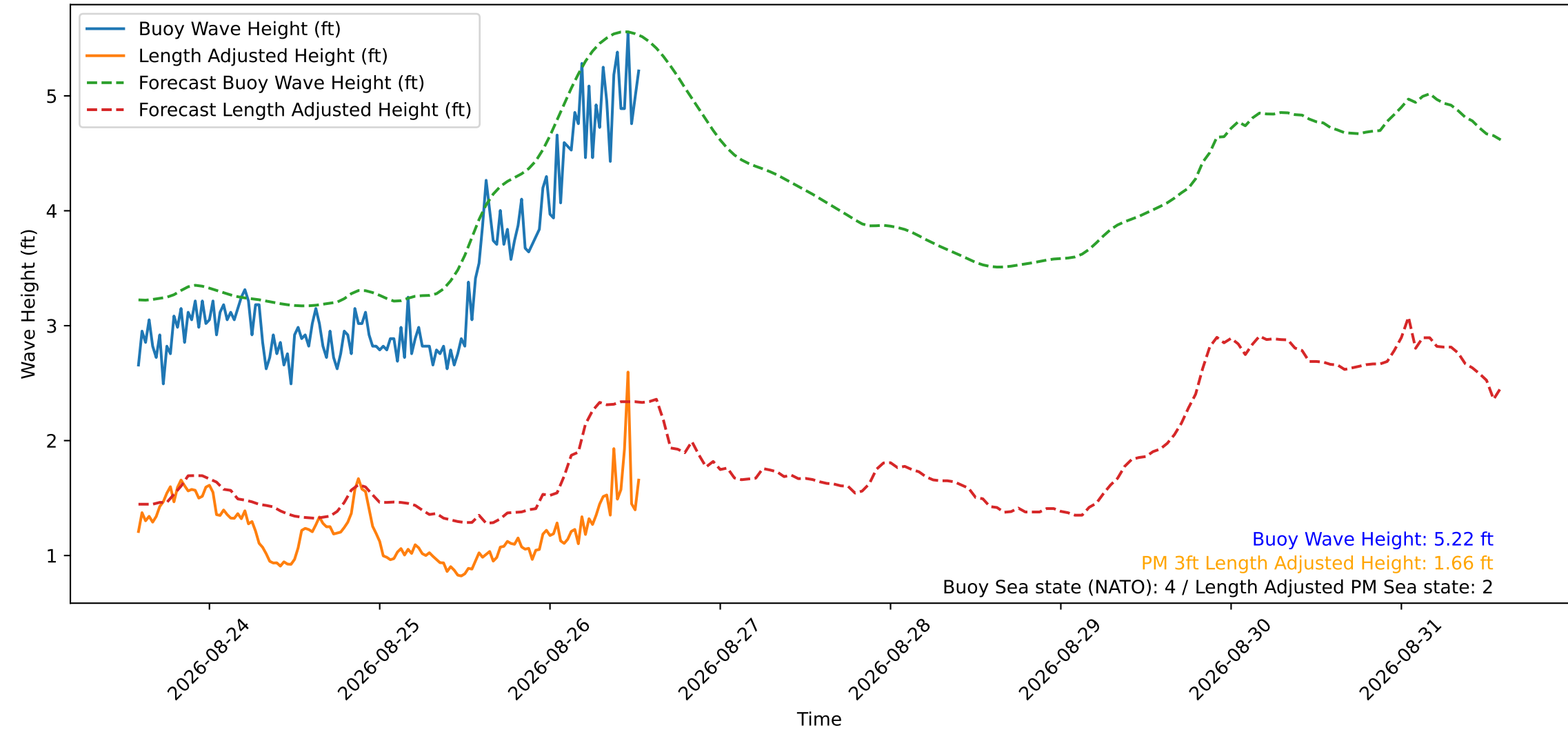
Wave Heights over Time for Green Beach at 2026-08-26 13:31:13
