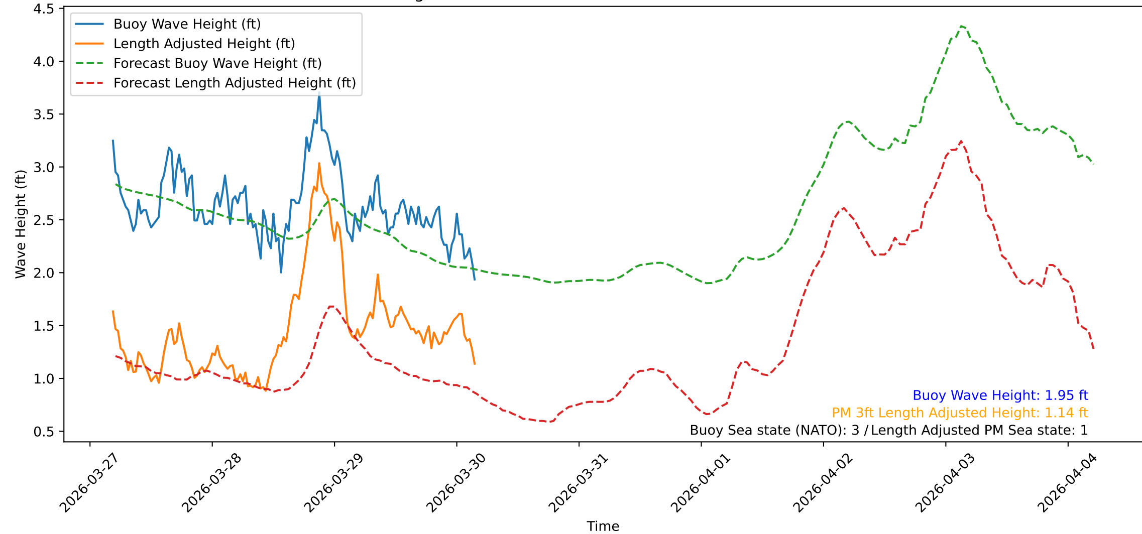
Wave Heights over Time for Green Beach at 2026-03-30 04:31:10
