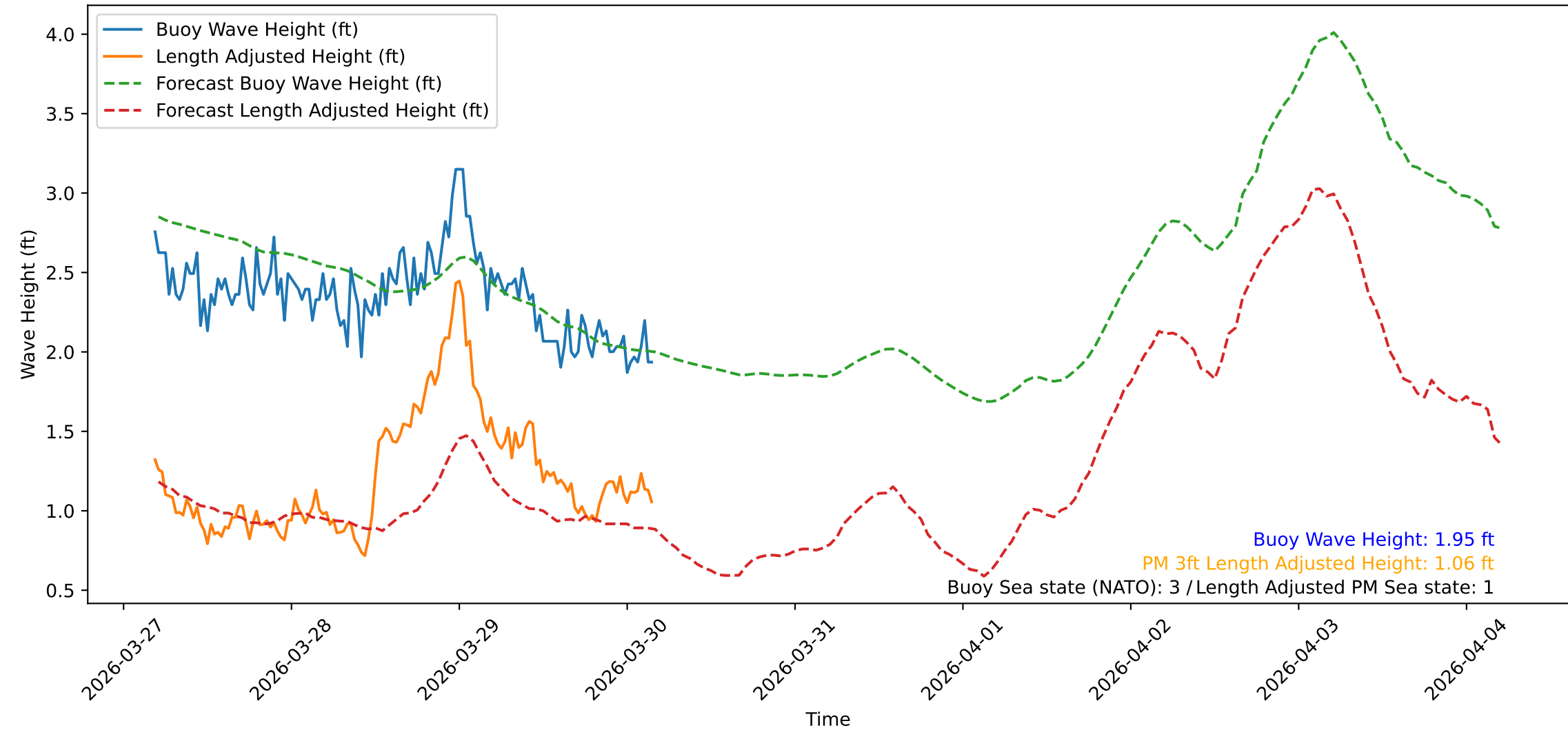
Wave Heights over Time for Oceanside Harbor at 2026-03-30 04:30:32
