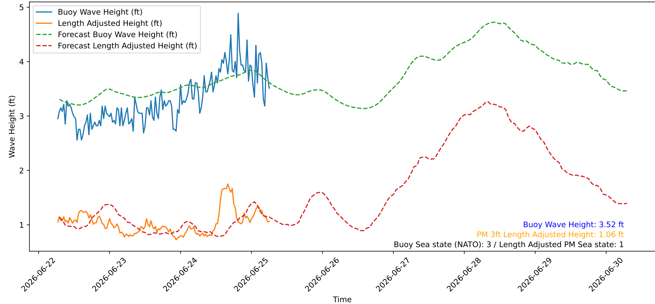
Wave Heights over Time for Oceanside Harbor at 2026-06-25 06:30:26
