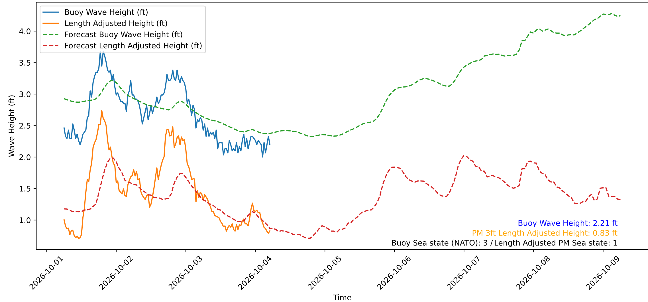
Wave Heights over Time for Green Beach at 2026-10-04 05:41:11
