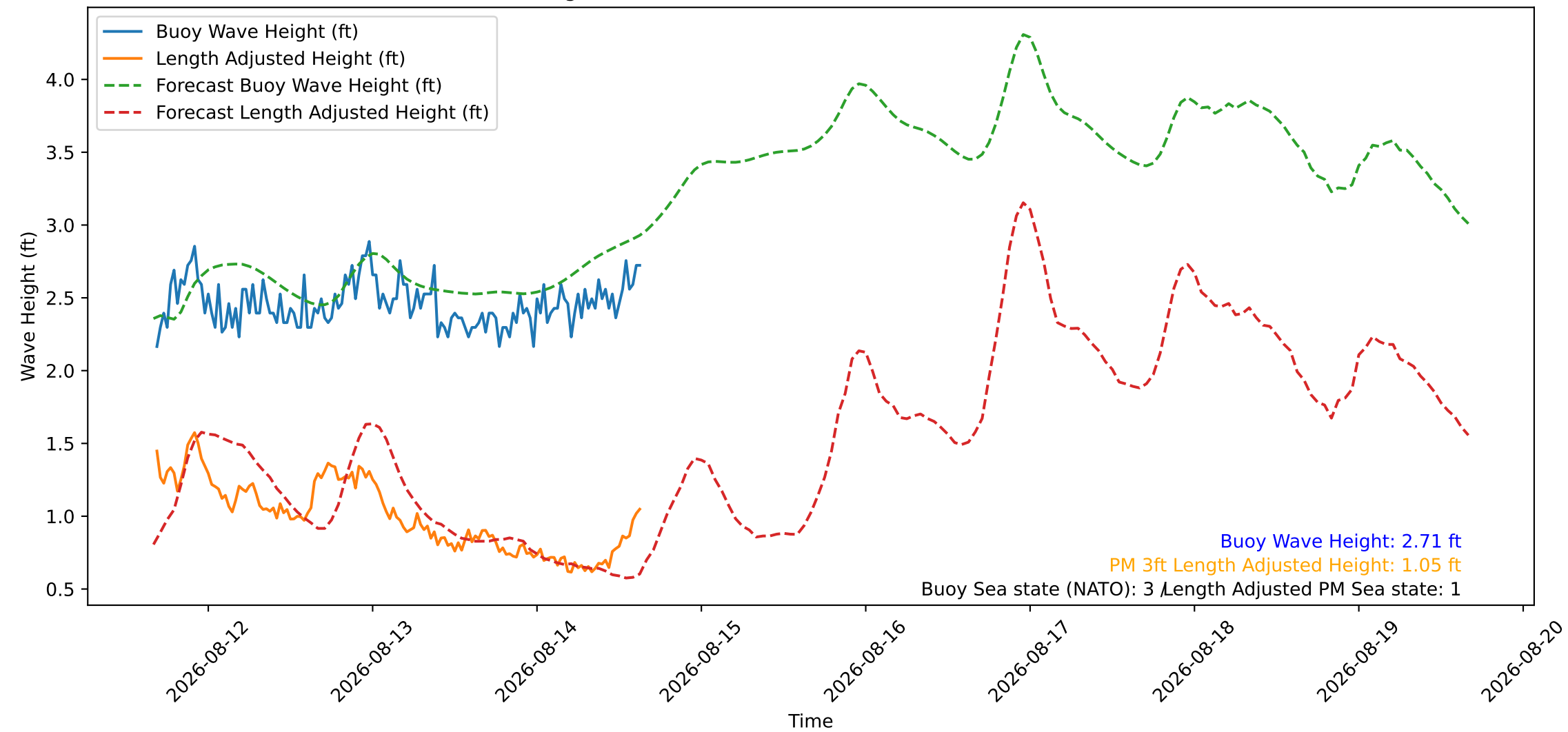
Wave Heights over Time for Red Beach at 2026-08-14 16:20:47
