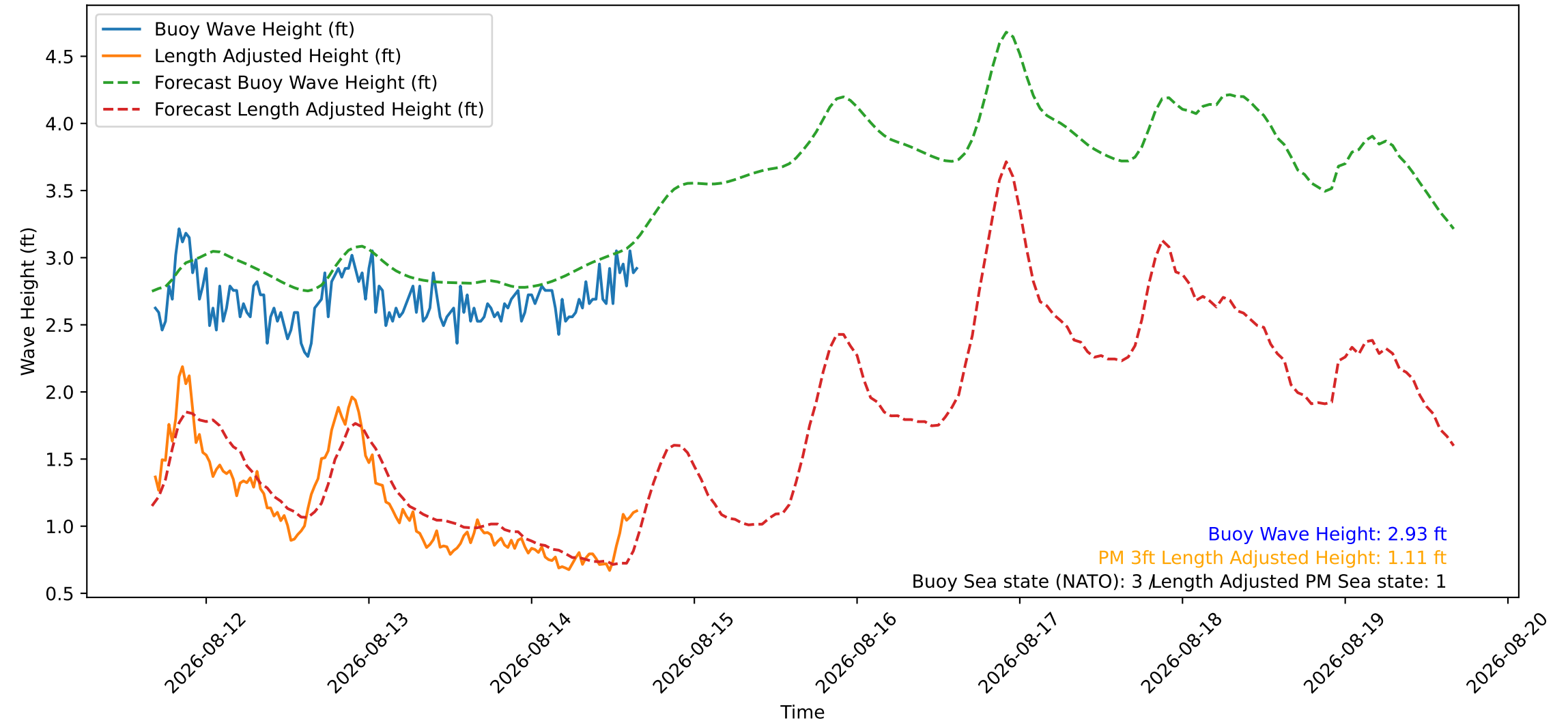
Wave Heights over Time for Green Beach at 2026-08-14 16:21:10
