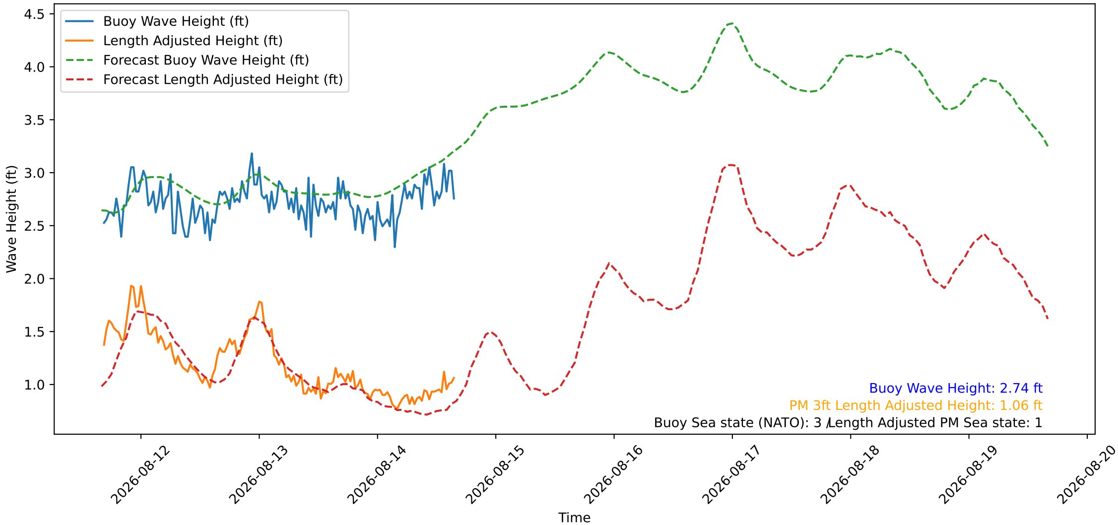
Wave Heights over Time for Oceanside Harbor at 2026-08-14 16:20:26
