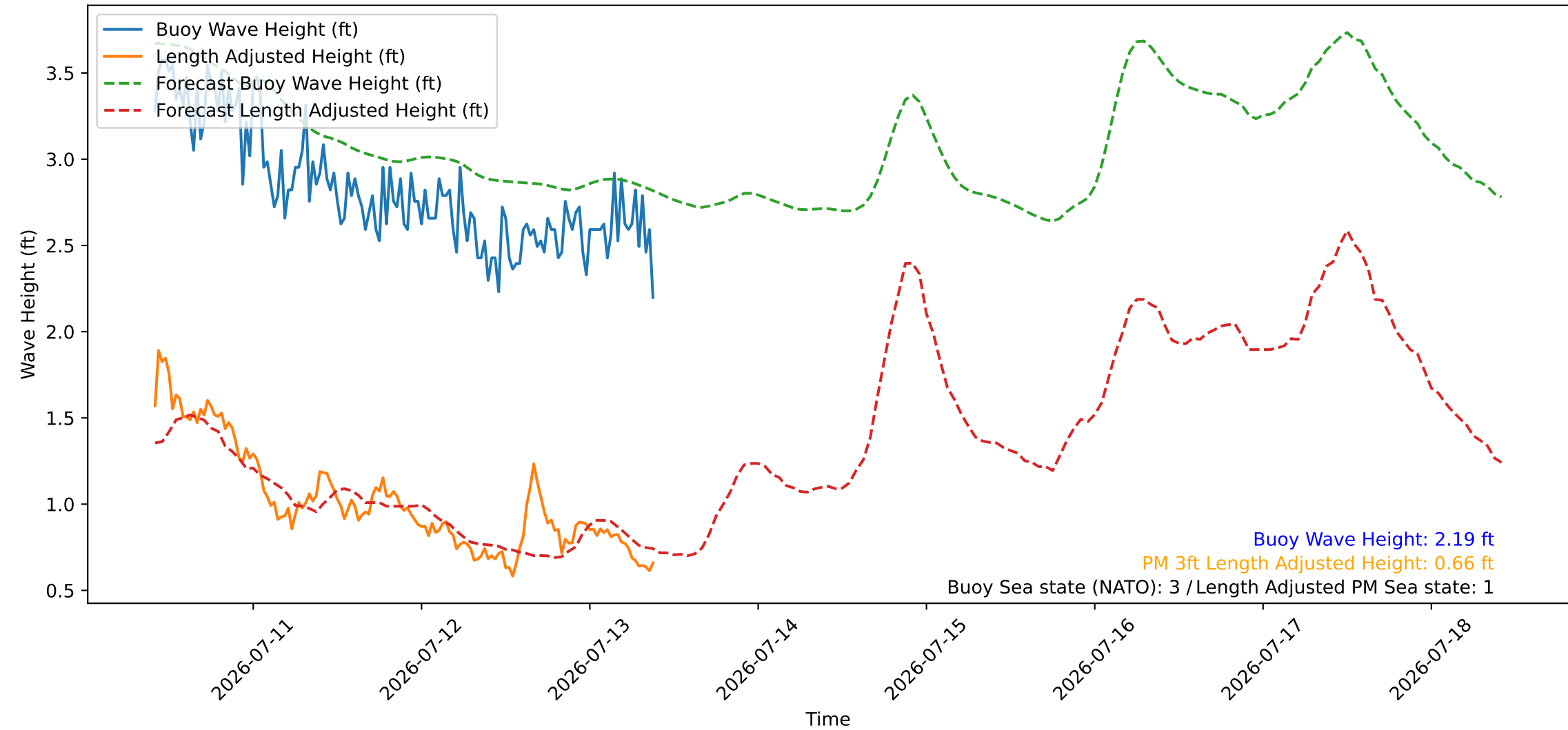
Wave Heights over Time for Green Beach at 2026-07-13 09:51:09
