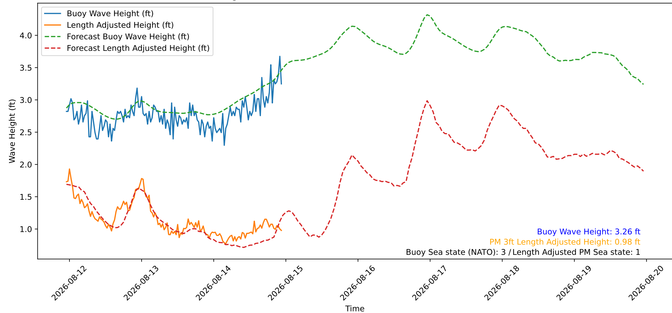
Wave Heights over Time for Oceanside Harbor at 2026-08-14 23:10:26
