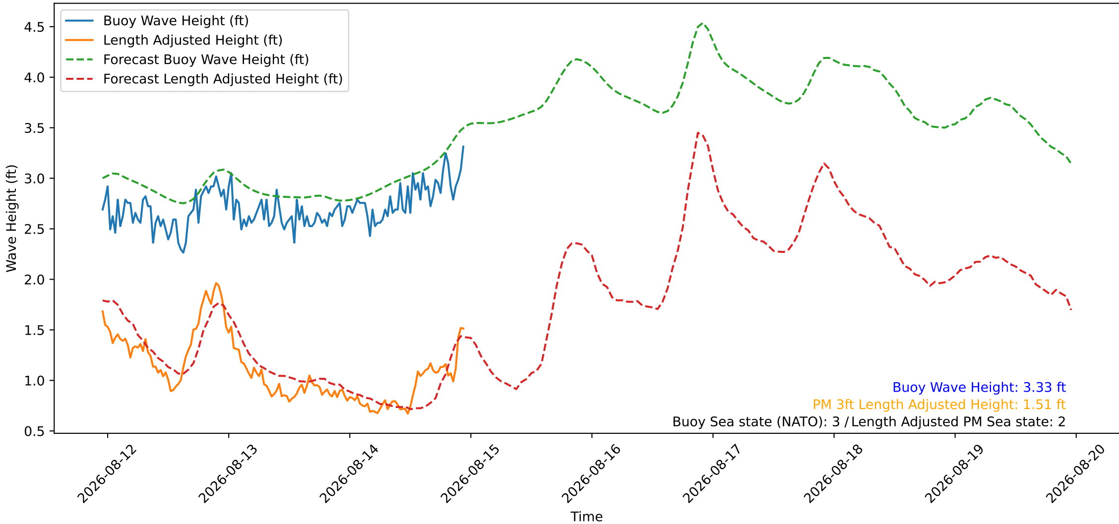
Wave Heights over Time for Green Beach at 2026-08-14 23:11:09
