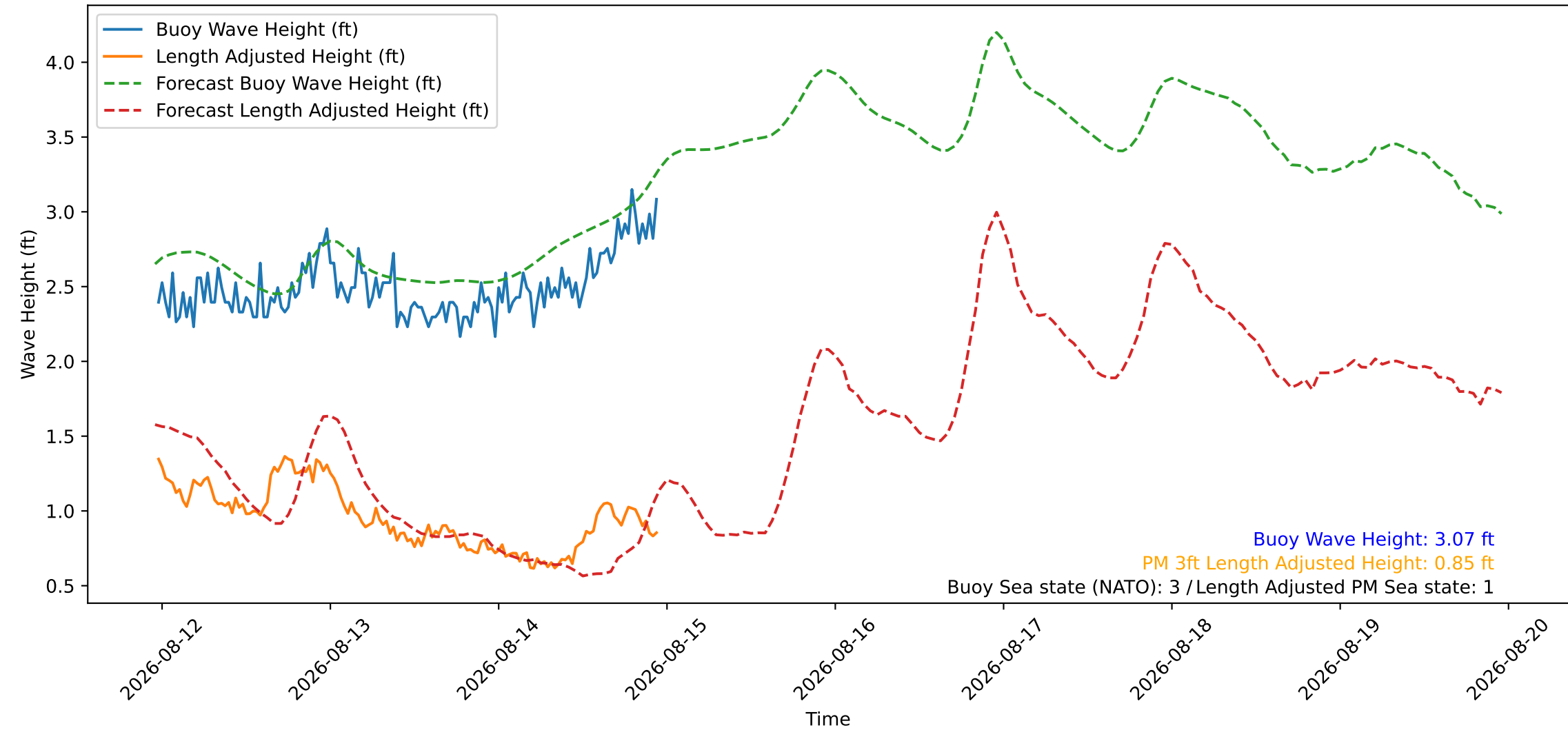
Wave Heights over Time for Red Beach at 2026-08-14 23:10:46
