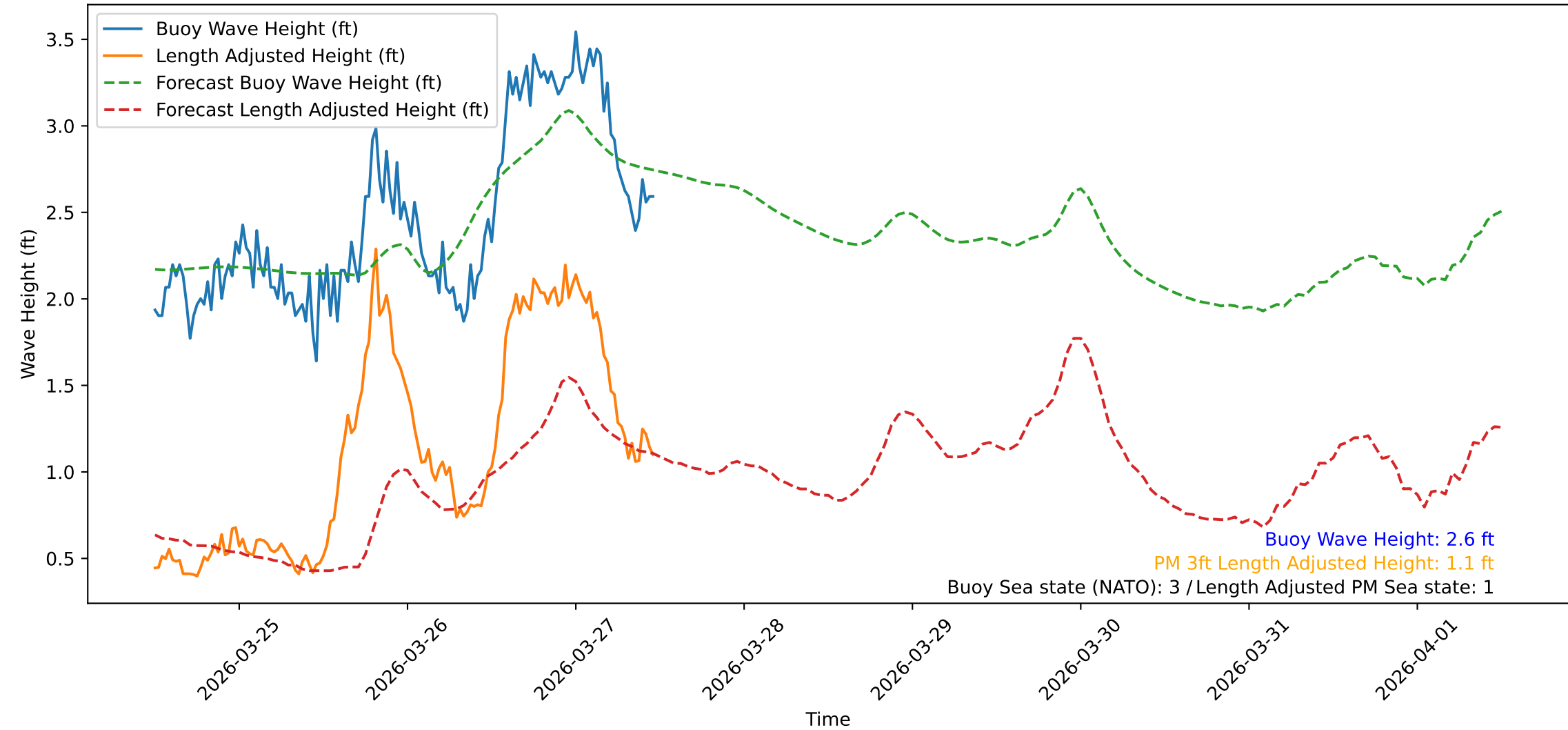
Wave Heights over Time for Green Beach at 2026-03-27 11:51:10
