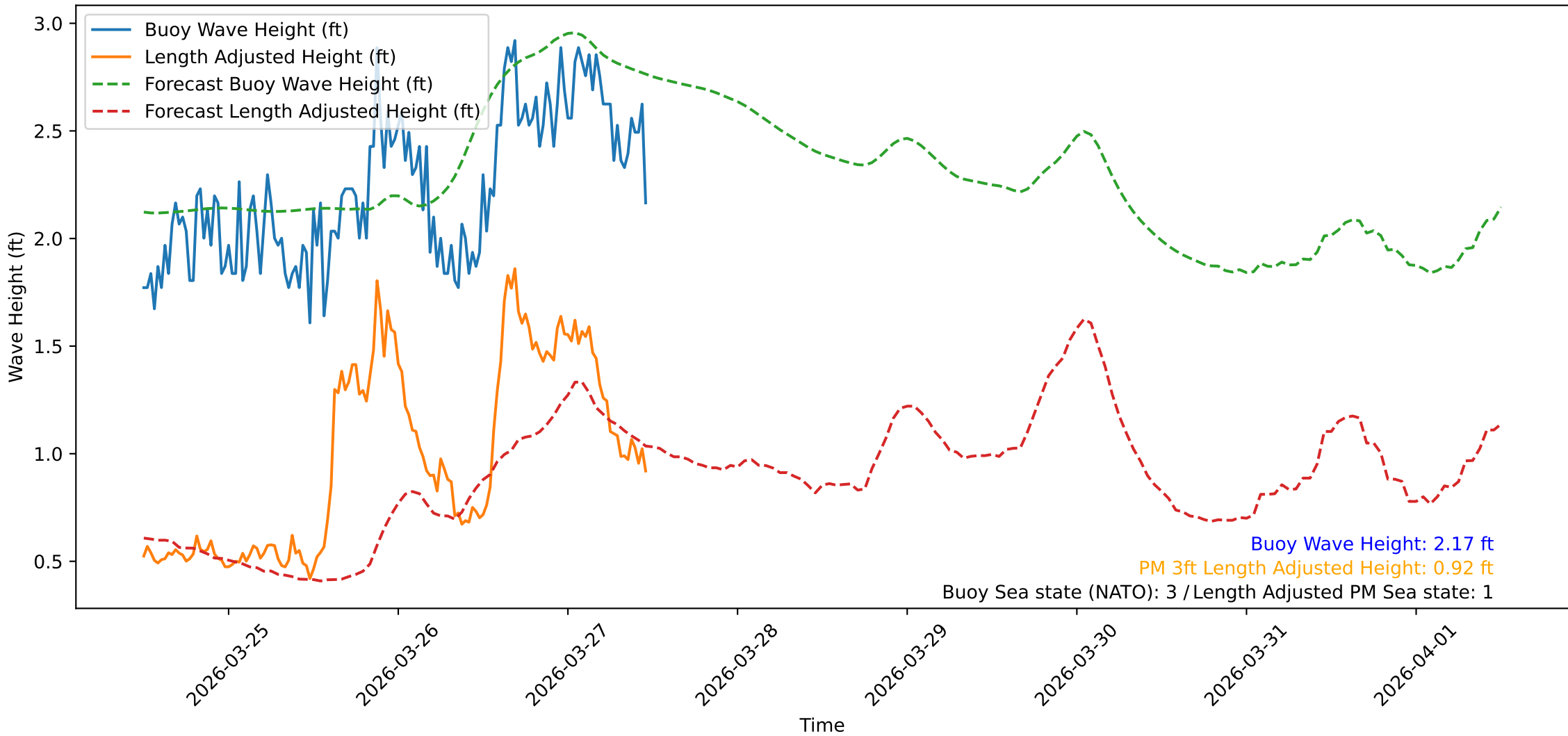
Wave Heights over Time for Oceanside Harbor at 2026-03-27 11:50:31
