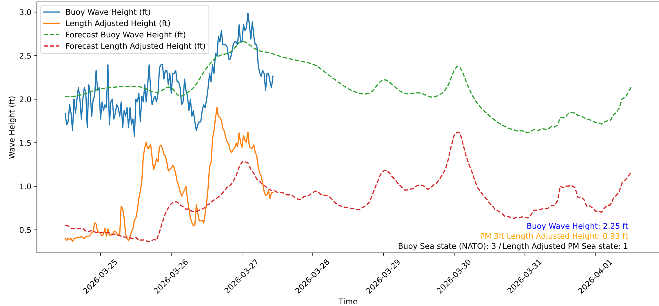
Wave Heights over Time for Red Beach at 2026-03-27 11:50:47
