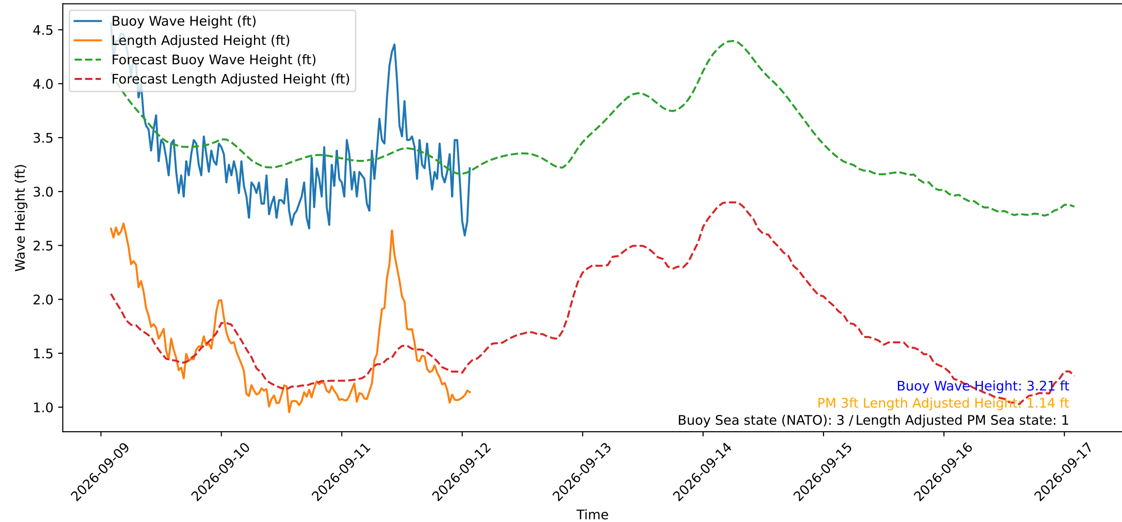
Wave Heights over Time for Oceanside Harbor at 2026-09-12 02:10:30
