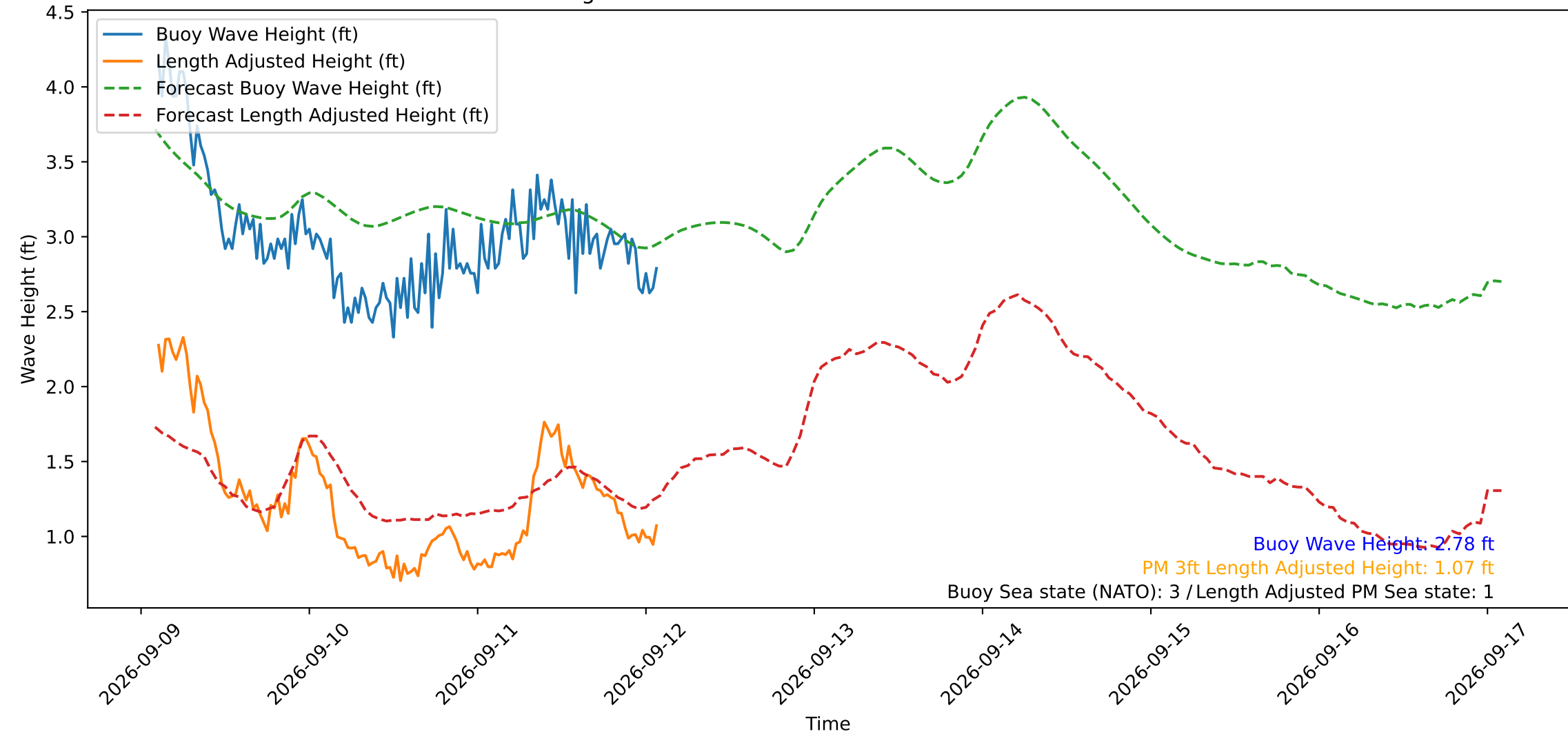
Wave Heights over Time for Red Beach at 2026-09-12 02:10:49
