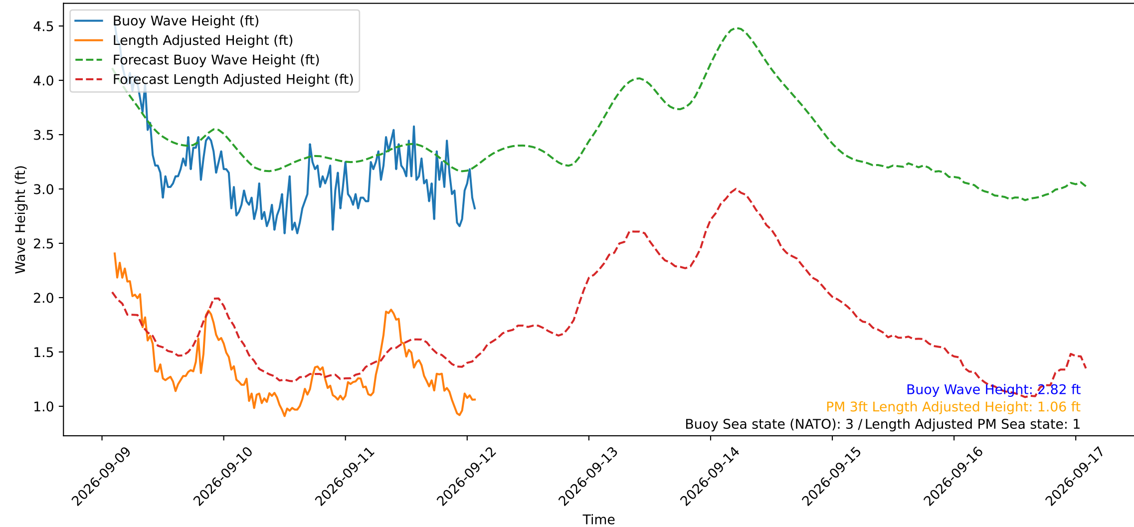
Wave Heights over Time for Green Beach at 2026-09-12 02:11:12
