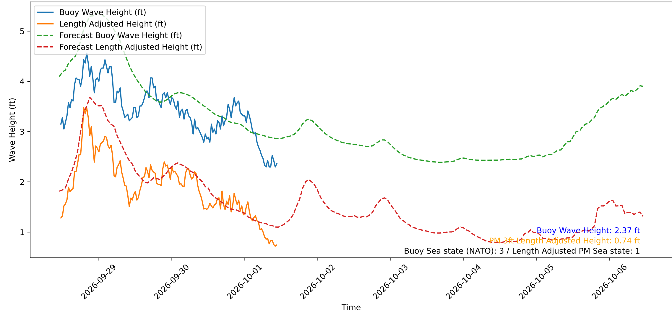
Wave Heights over Time for Green Beach at 2026-10-01 11:11:12
