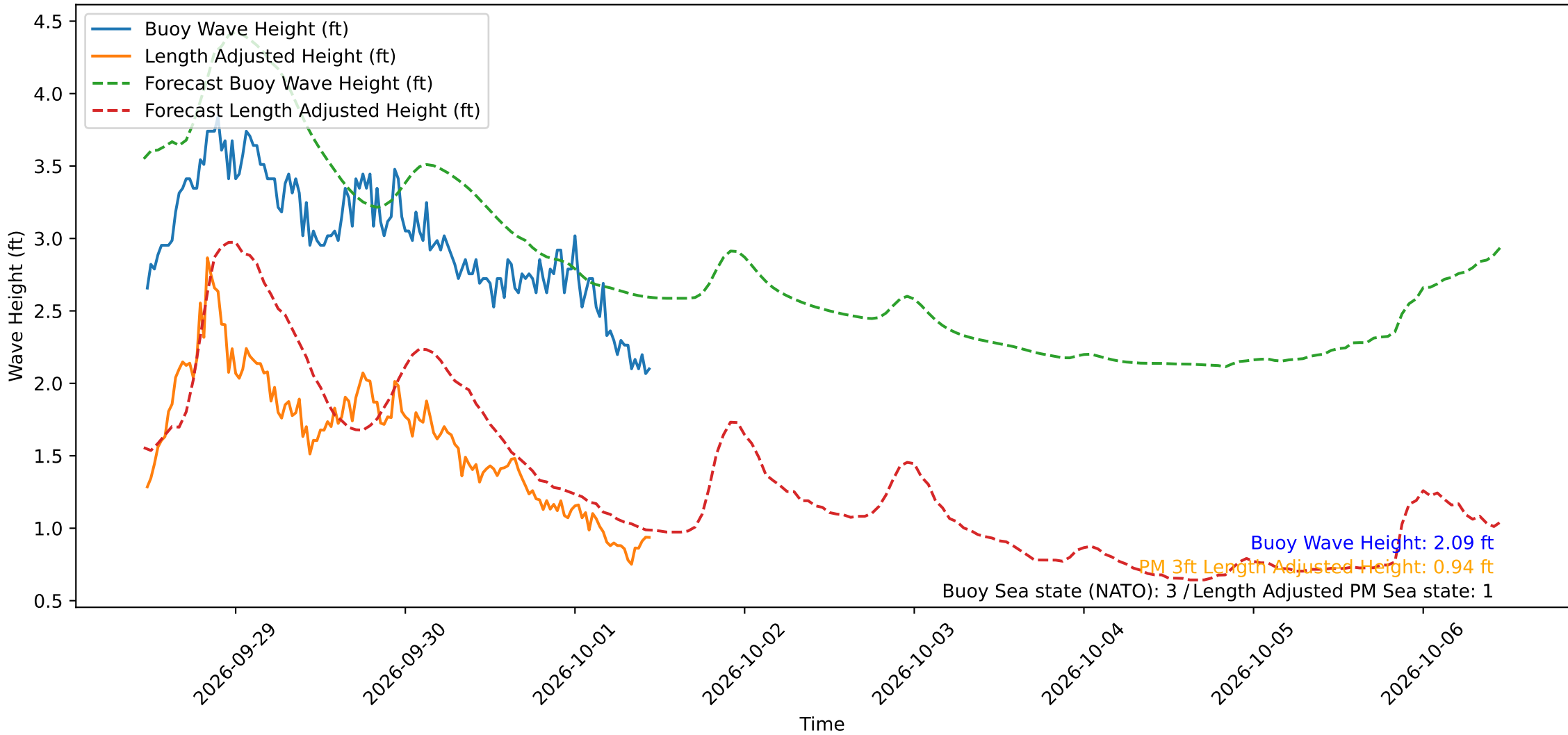
Wave Heights over Time for Red Beach at 2026-10-01 11:10:50
