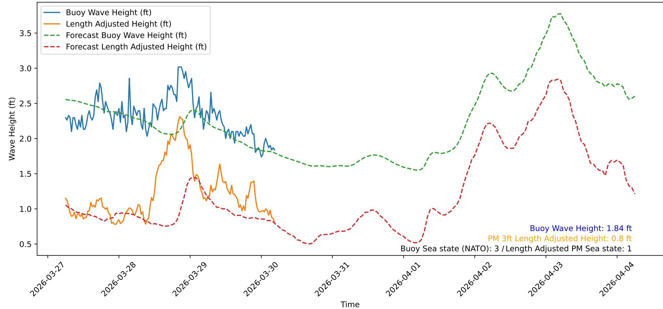
Wave Heights over Time for Red Beach at 2026-03-30 05:30:46
