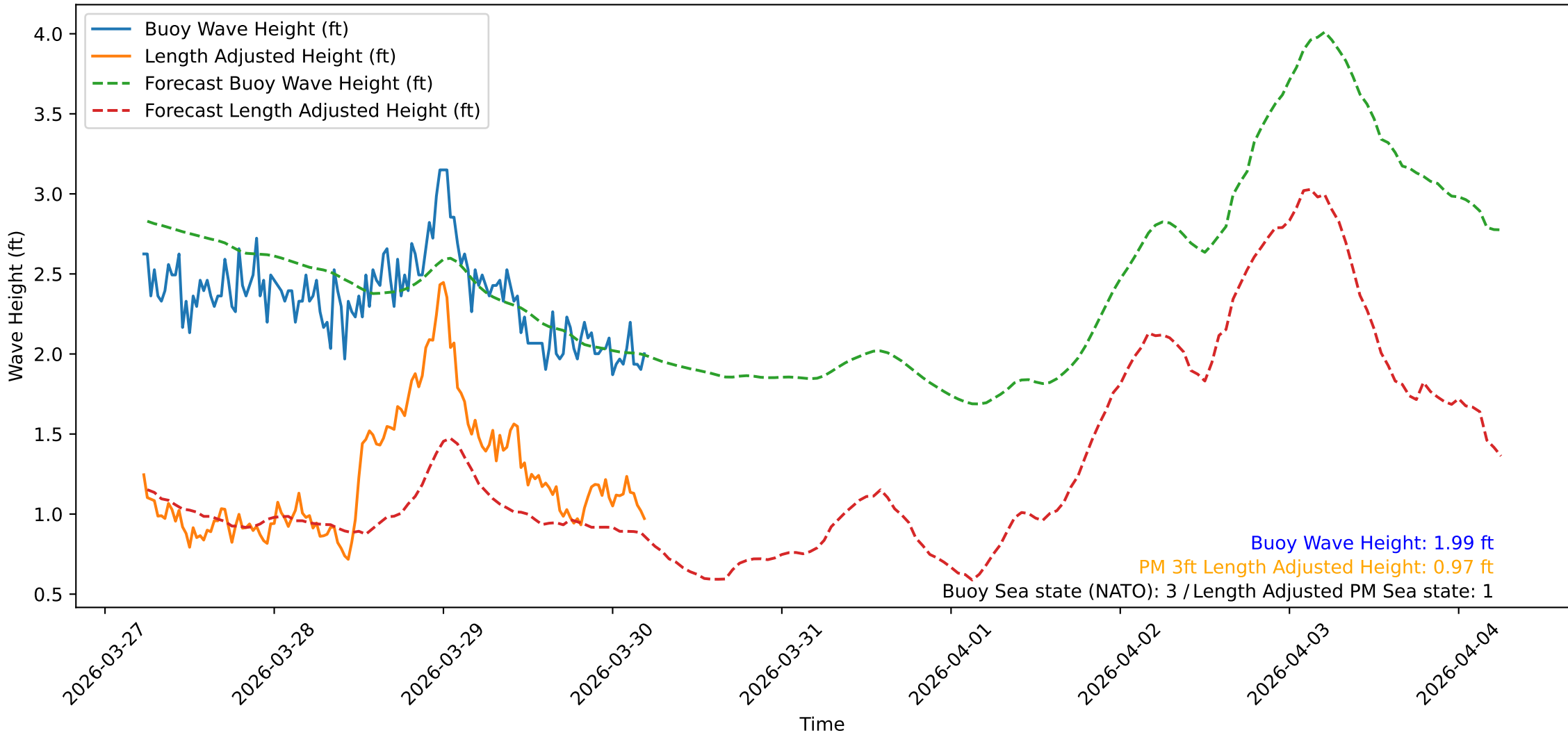
Wave Heights over Time for Oceanside Harbor at 2026-03-30 05:30:31
