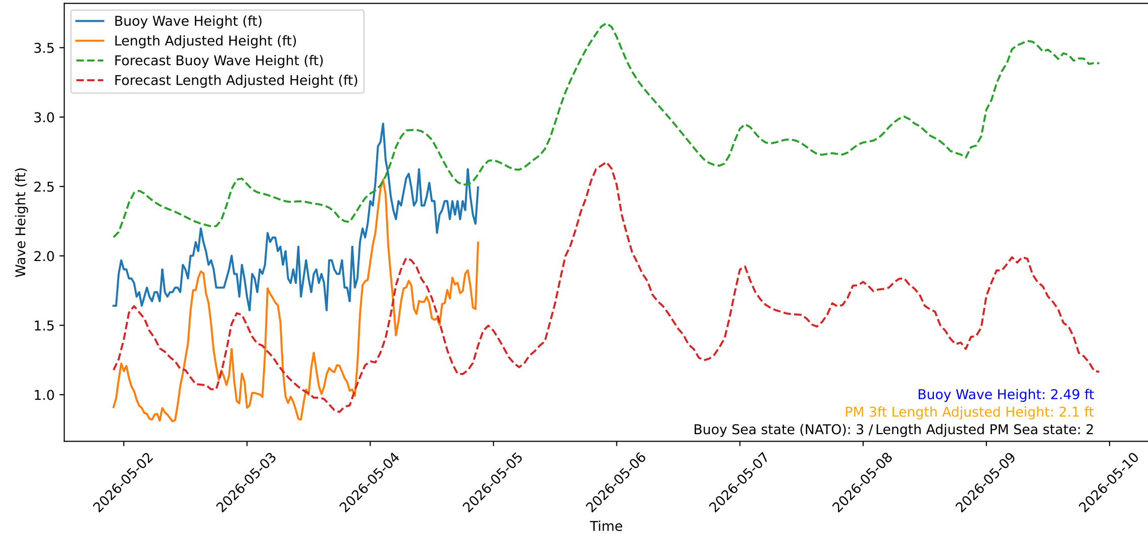
Wave Heights over Time for Red Beach at 2026-05-04 21:50:51
