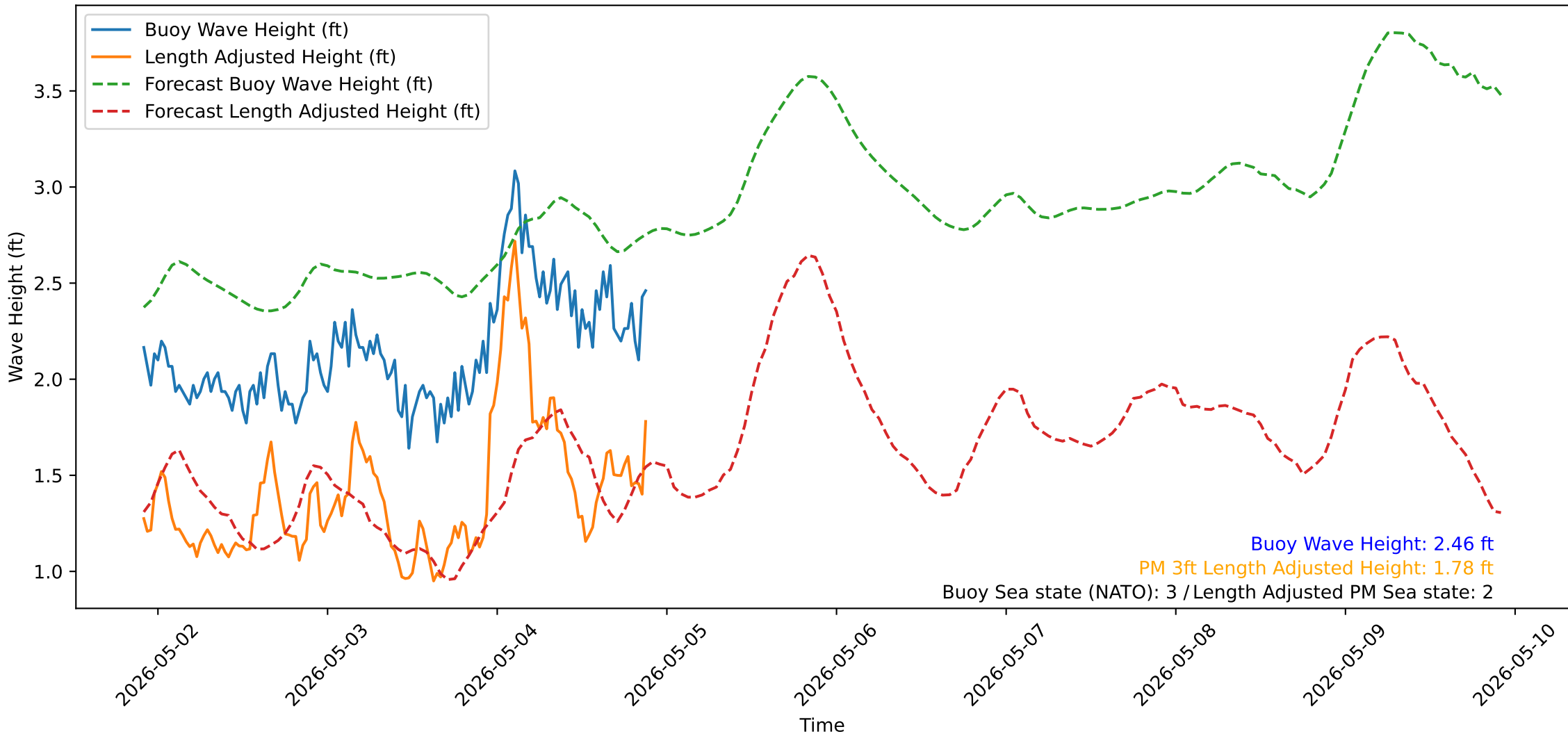
Wave Heights over Time for Oceanside Harbor at 2026-05-04 21:50:31
