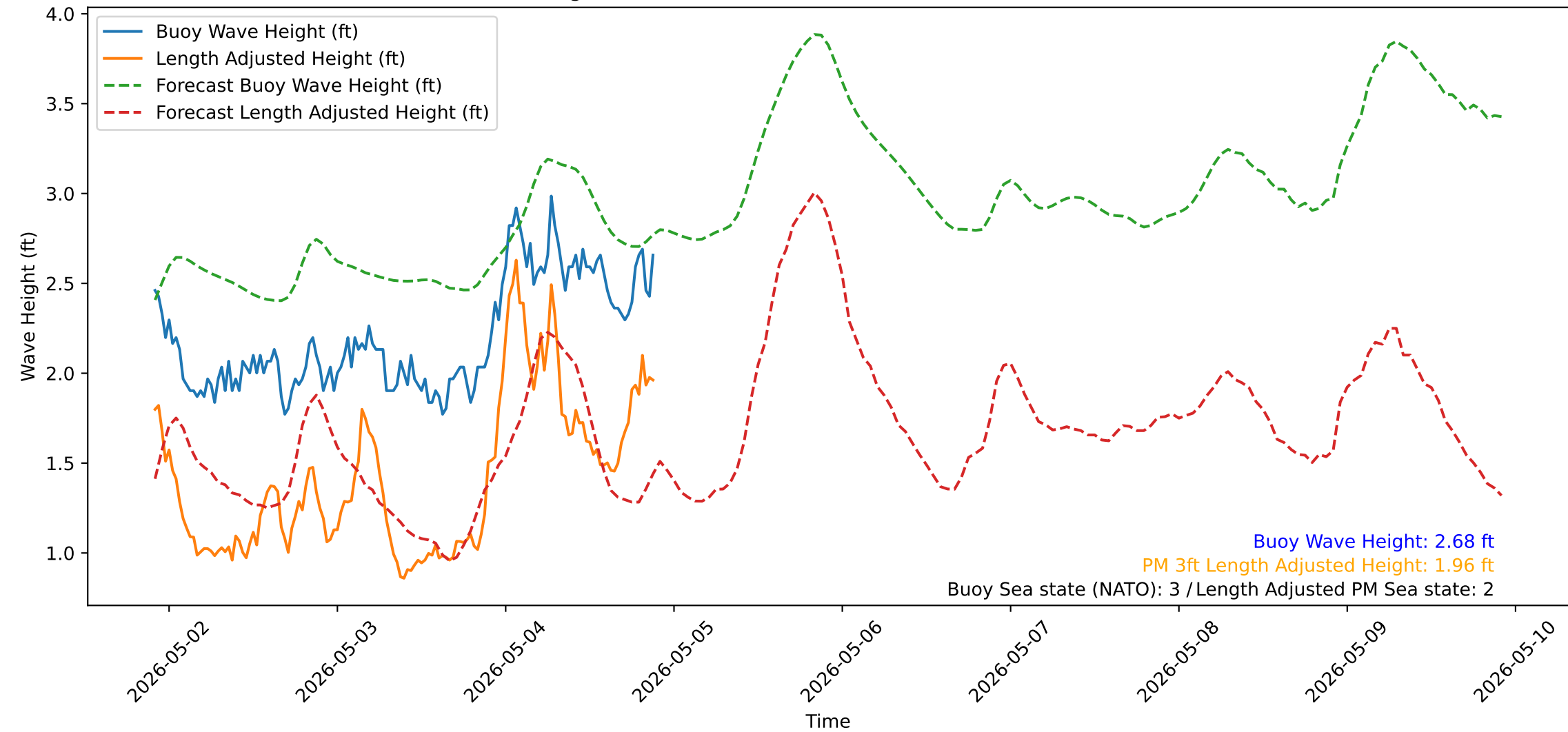
Wave Heights over Time for Green Beach at 2026-05-04 21:51:14
