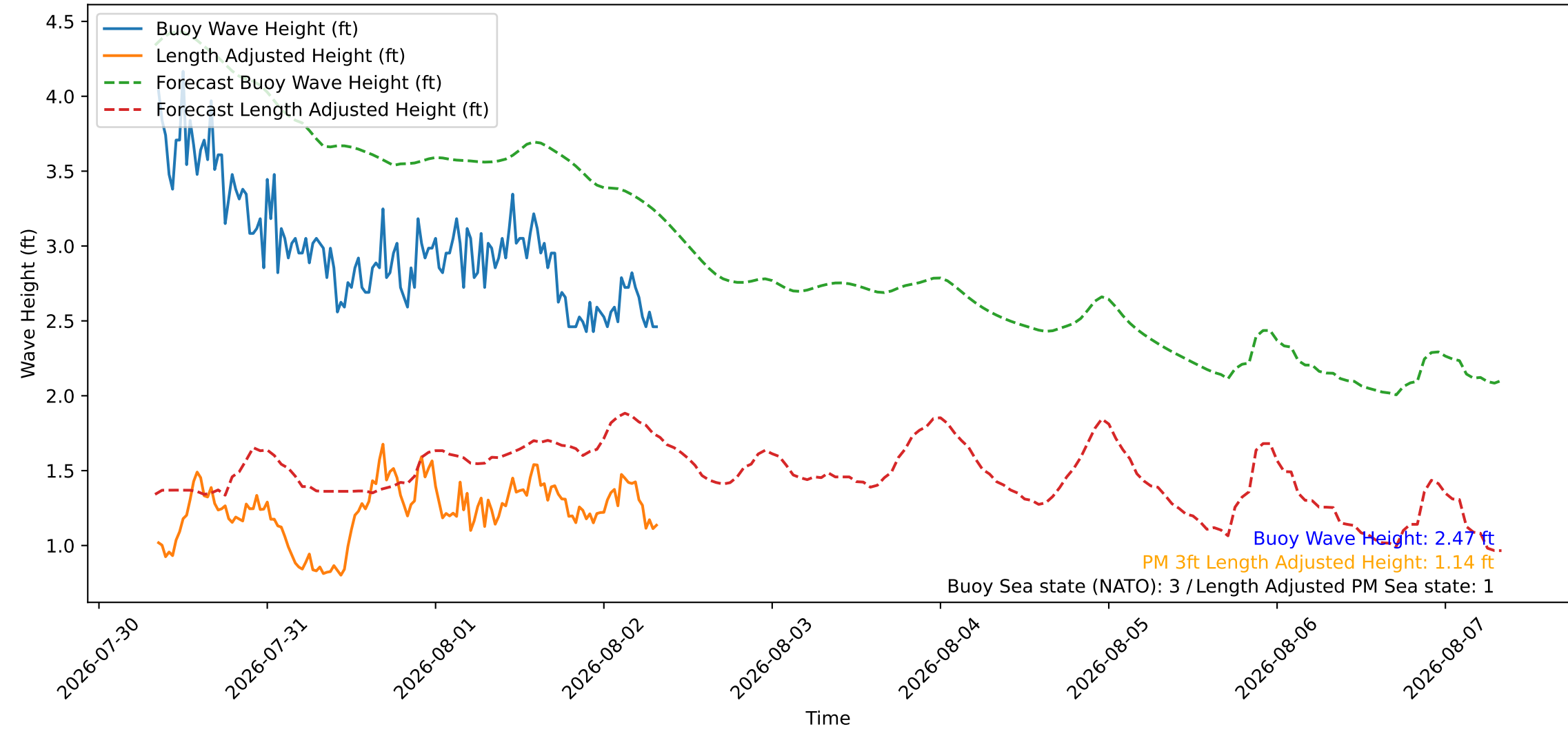
Wave Heights over Time for Red Beach at 2026-08-02 08:20:47
