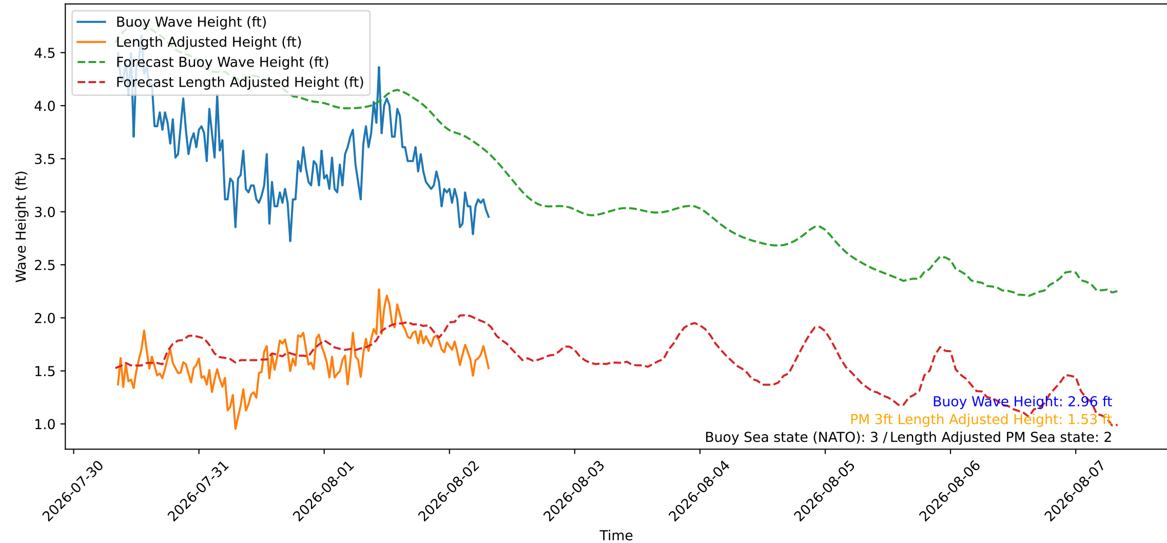
Wave Heights over Time for Oceanside Harbor at 2026-08-02 08:20:26
