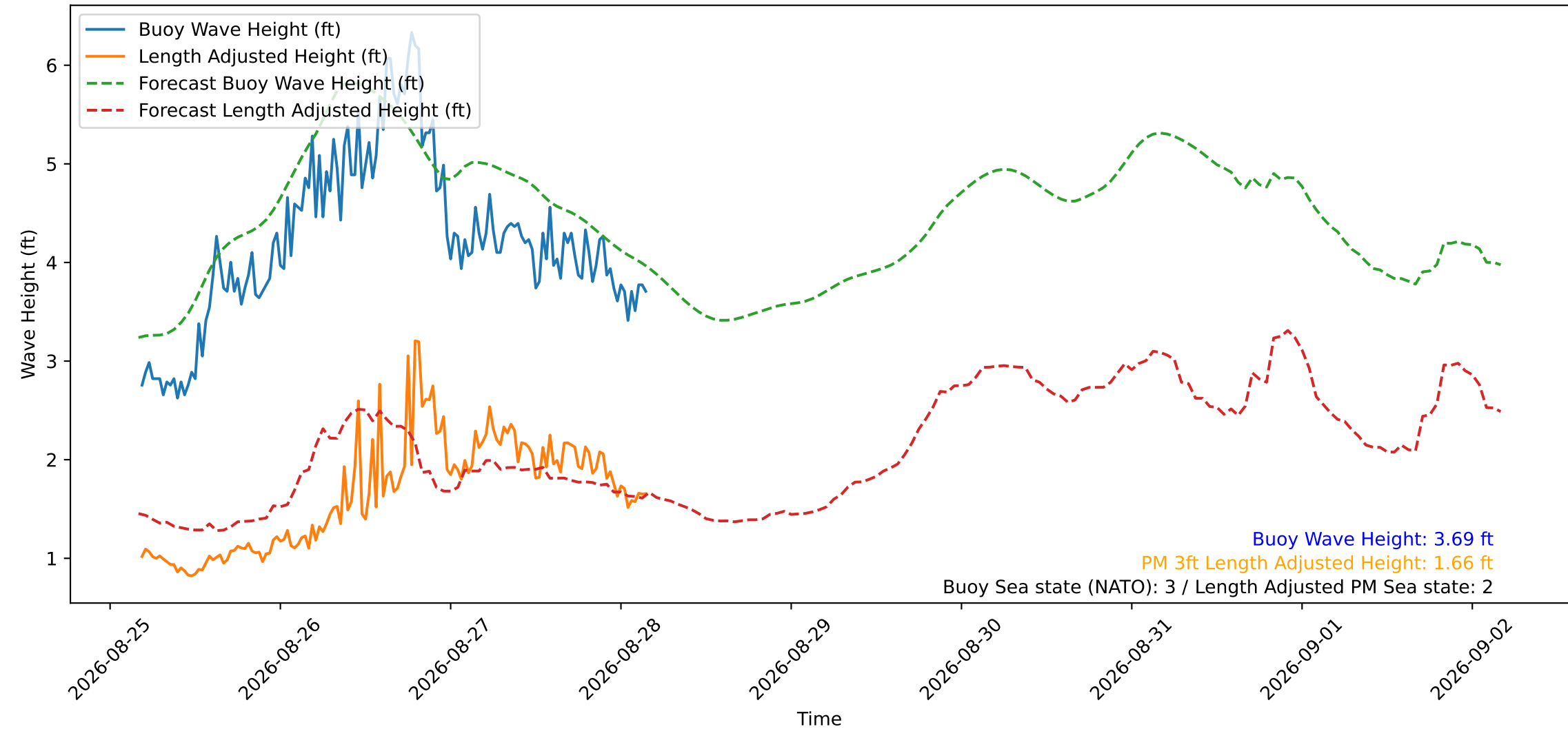
Wave Heights over Time for Green Beach at 2026-08-28 04:21:14
