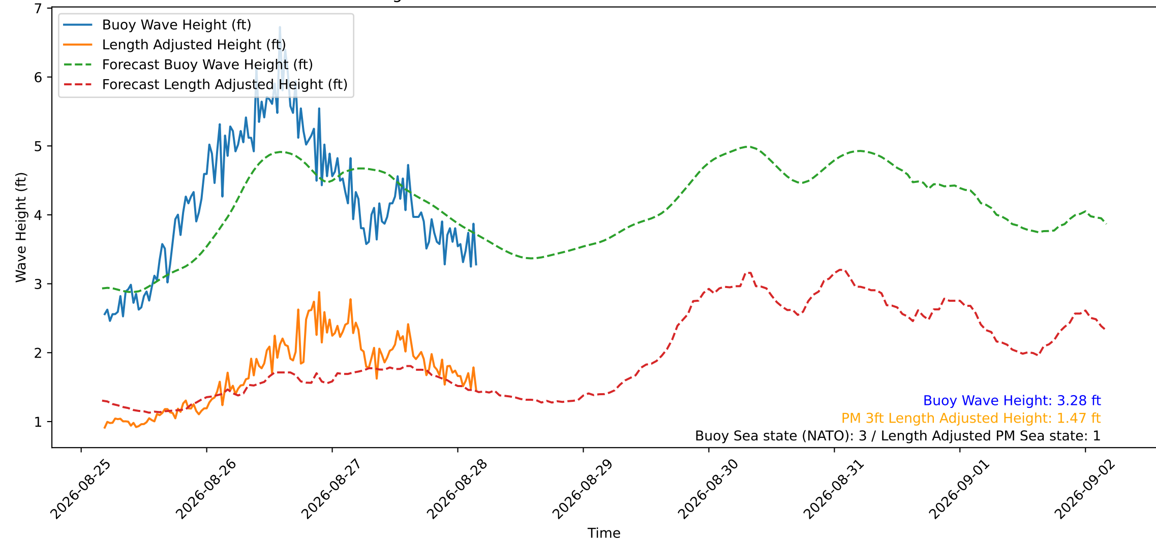
Wave Heights over Time for Oceanside Harbor at 2026-08-28 04:20:29
