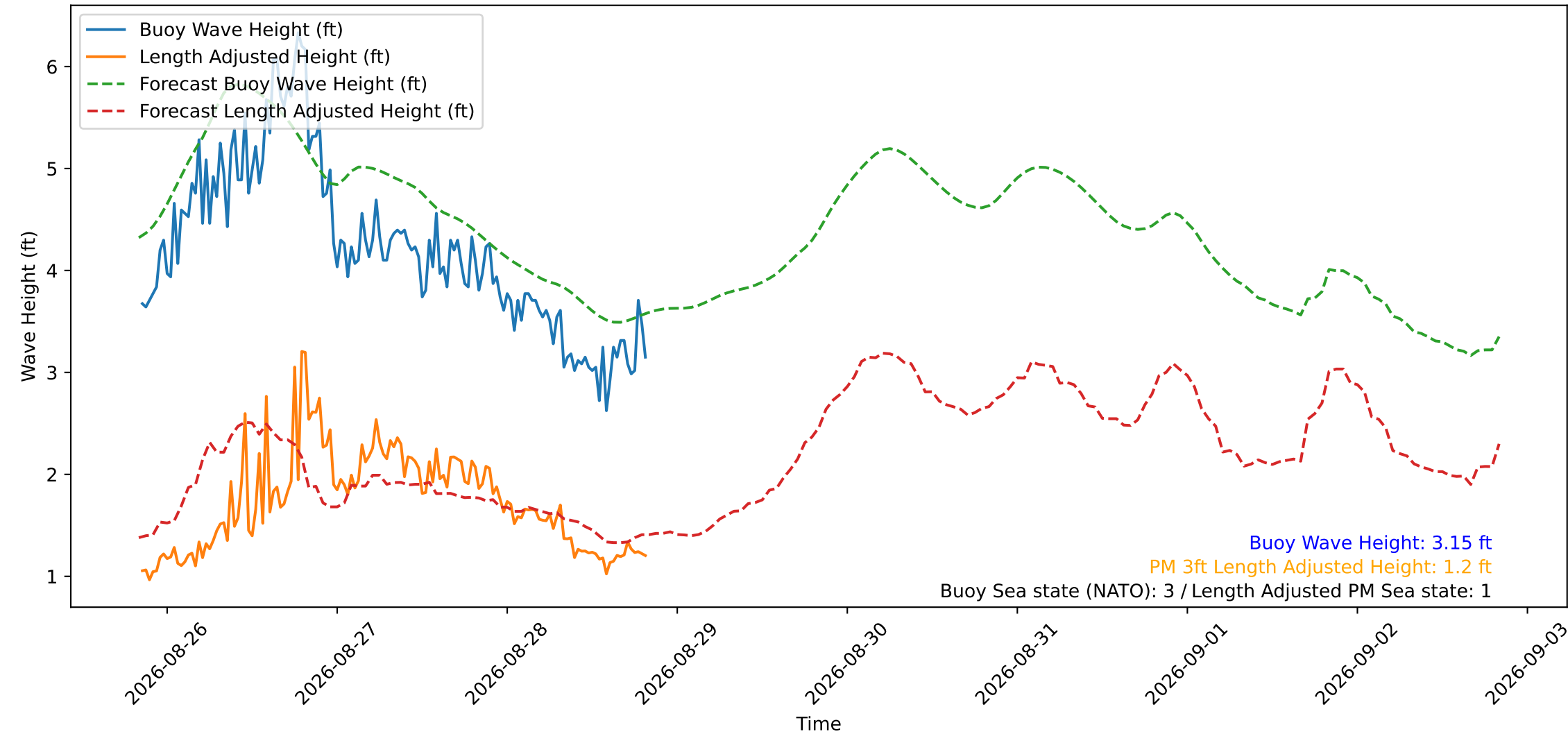
Wave Heights over Time for Green Beach at 2026-08-28 20:11:11
