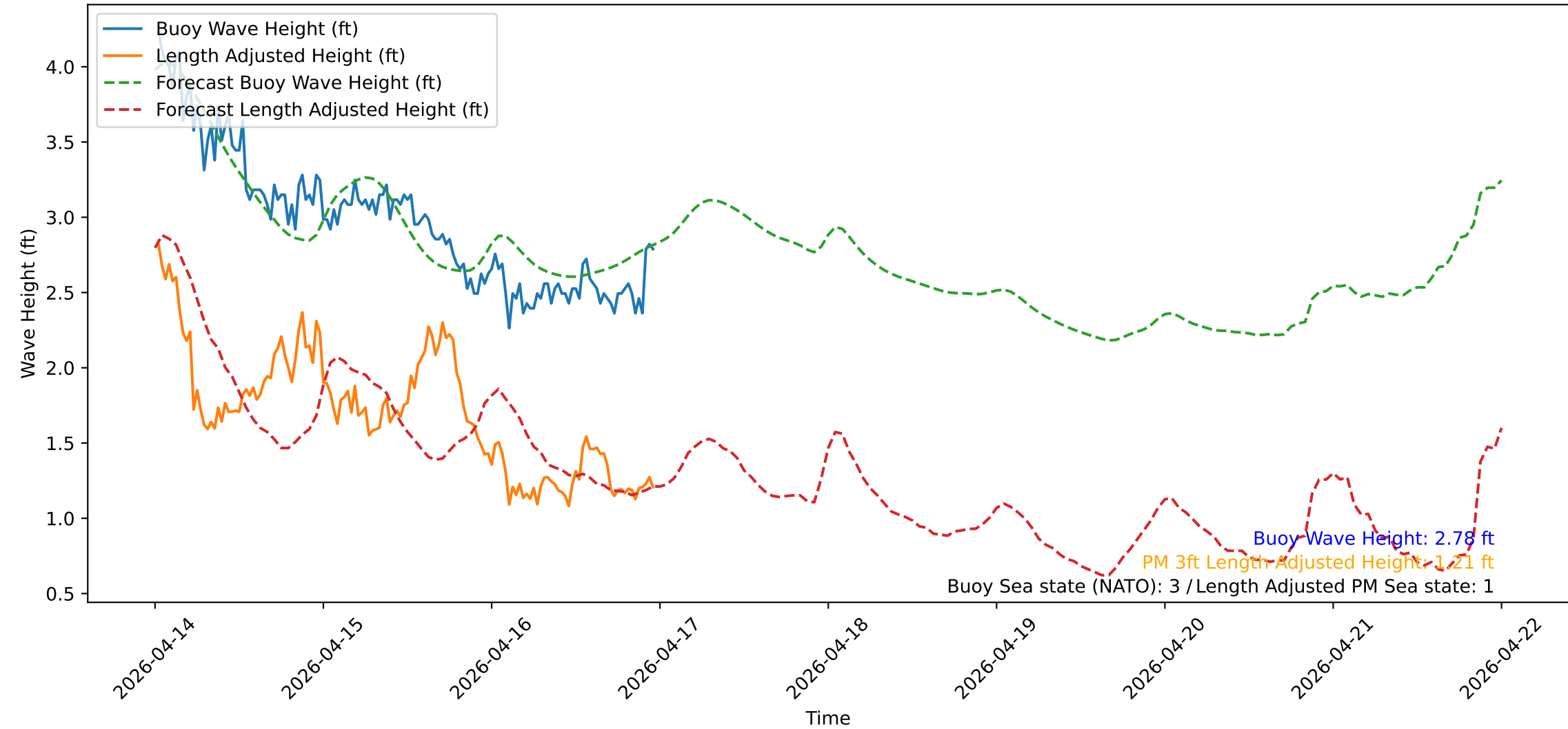
Wave Heights over Time for Red Beach at 2026-04-17 00:00:51
