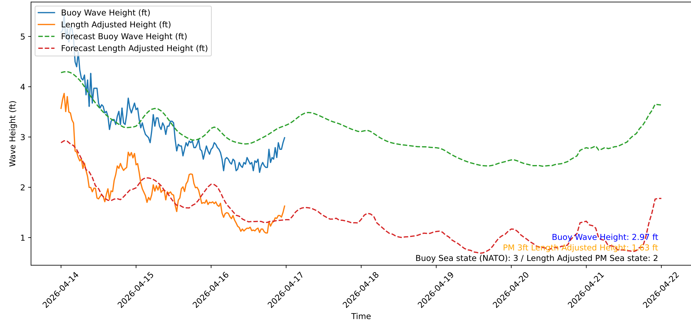
Wave Heights over Time for Oceanside Harbor at 2026-04-17 00:00:32
