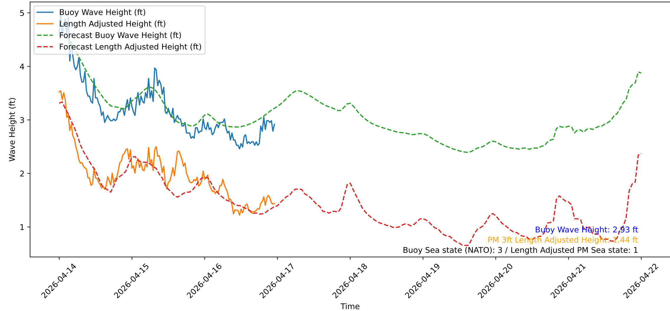
Wave Heights over Time for Green Beach at 2026-04-17 00:01:13
